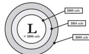
Region of LOWEST pressure relative to its surroundings
