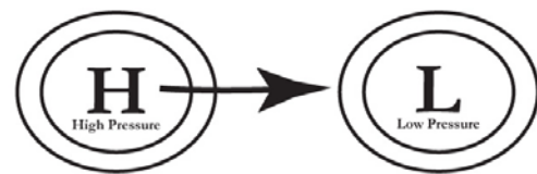
The influence of the pressure gradient force
