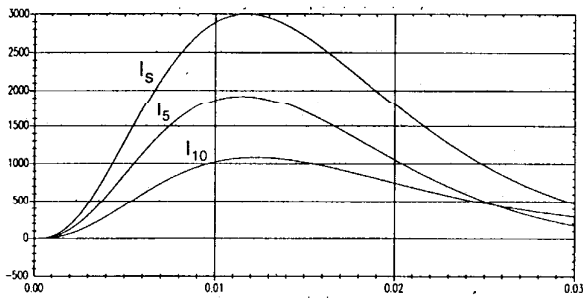
Currents in branches: Time in milliseconds, peaks in amperes
