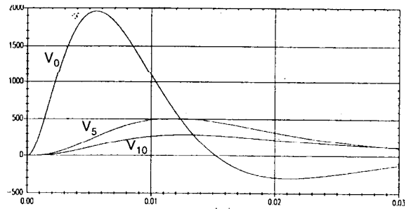
Voltages at nodes: Time in milliseconds, peaks in volts
