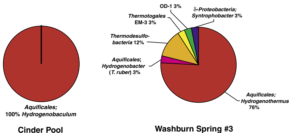
Figure 5. Results of phylogenetic analyses from Cinder Pool, Norris region, and a lower Washburn Spring, Canyon region, Yellowstone National Park. Cinder Pool is 88°C, pH 4.2, and contains 77 nM H 2 , 1.2 \mu M CH 4 , 47 \mu M sulfide, and 1 \mu M sulfate. One of the Lower Washburn Springs, #3, is 86°C, pH 6.2, and contains 19 nM H 2 , 5.8 \mu M CH 4 , 167 \mu M sulfide, and 44 \mu M sulfate.
