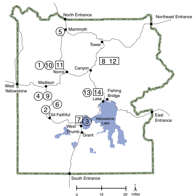
Figure 3. Map of Yellowstone National Park showing the authors' research locations by site number. Hydrogen measurements were conducted in the field by the method described at all sites. Site numbers in boxes represent sites with associated phylogenetic analyses conducted in the laboratory at the University of Colorado.
