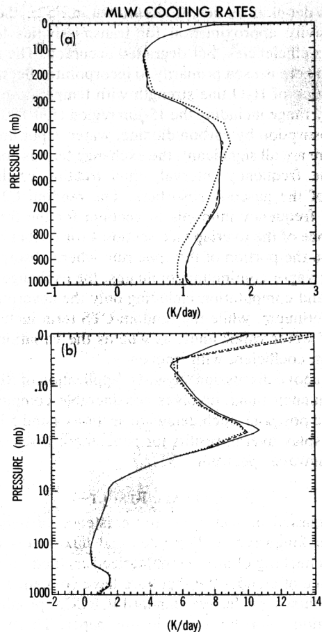
Fig. 4. Same as Figure 2, but with cooling rates for the AFGL mid-latitude winter (MLW) profile.
