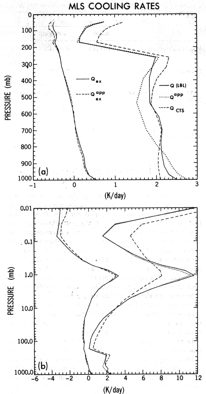
Fig. 1. Cooling rates (in K/d) for the AFGL mid-latitude summer (MLS) profile with the absorbers \text{H}_2\text{O} , \text{CO}_2 , \text{O}_3 , and the water vapor continuum included. The three curves on the right side of the figure give the line-by-line cooling rate ( Q(\text{LBL}) ), the LBL cool-to-space cooling rate ( Q_{\text{CTS}} ), and Q^{\text{app}} , obtained by the methods given in this paper. The two curves on the left side of the figure give Q_{\text{ex}} (defined in (6)) and Q_{\text{ex}}^{\text{app}} . In Figure 1a, tropospheric results are emphasized, with the ordinate being pressure, ranging from 0 to 1000 mbar. In Figure 1b, middle atmosphere results are emphasized; the ordinate is pressure, ranging from 1000 to 0.01 mbar on a logarithmic scale.
