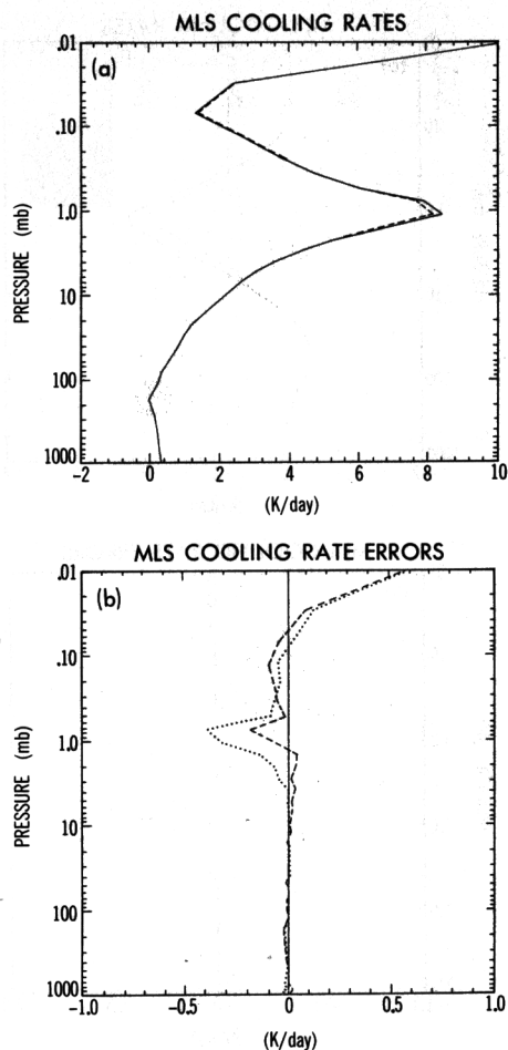
Fig. 25. (a) Cooling rates for the MLS profile in the middle atmosphere. The absorber is \text{CO}_2 . The solid line gives LBL results for the 0\text{--}3000\text{ cm}^{-1} frequency range, and the dashed line the LBL results over the 490\text{--}850\text{ cm}^{-1} frequency range. Both calculations use the degraded vertical resolution. (b) Cooling rate errors for the MLS profile in the middle atmosphere. The absorber is \text{CO}_2 . The dotted line gives the difference between the SEA88 computation and the LBL result for the 0\text{--}3000\text{ cm}^{-1} frequency range, and the dashed line gives the difference between the SEA88 computation and the LBL result for the 15\text{-}\mu\text{m} band ( 490\text{--}850\text{ cm}^{-1} ).
