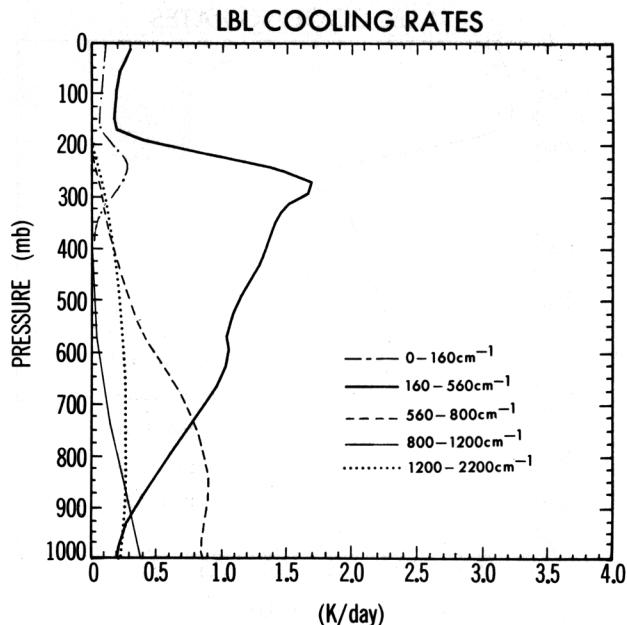
Fig. 11. Cooling rates by frequency range for the MLS profile using the LBL method. The absorber is \text{H}_2\text{O} (lines only). The frequency ranges included are 0–160, 160–560, 560–800, 800–1200, and 1200–2200 \text{cm}^{-1} .
