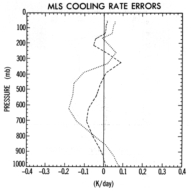
Fig. 15. Same as Figure 14, but the dotted line gives errors using the emissivity calculation with 10 \text{cm}^{-1} bandwidth in the 160\text{--}560 \text{cm}^{-1} frequency range, and the dashed line gives errors using the SEA formulation, with a 10 \text{cm}^{-1} bandwidth used for calculation of the random CTS term.
