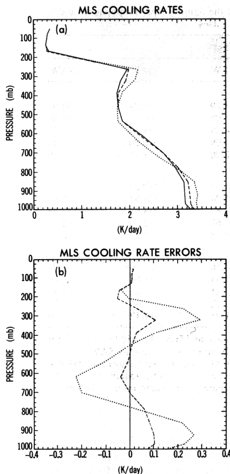
Fig. 8. (a) Cooling rates for the MLS profile. Absorption from H_2O (lines plus continuum) is included. The solid line gives degraded LBL results, the dashed line gives results for SEA88, and the dotted line gives results for SEA75. (b) Cooling rate errors for the MLS profile, with absorption from H_2O (lines plus continuum) included. The dashed line gives errors due to the SEA88 computation, and the dotted line errors owing to the SEA75 formulation, as in Figure 7a. Tropospheric results are emphasized.
