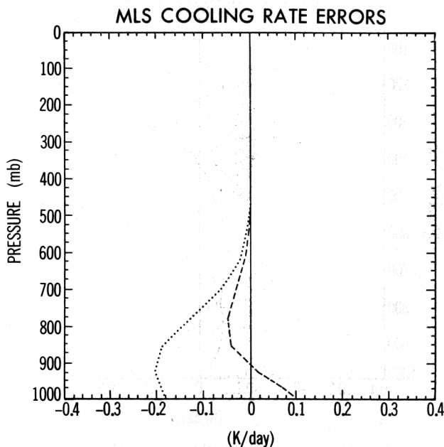
Fig. 19. Cooling rate errors for the MLS profile in the \text{H}_2\text{O} continuum-only case. The frequency range used is 800-1200 \text{ cm}^{-1} . The dotted line is the one-band ( Q^{\text{app}} ) error, and the dashed line the error of the SEA88 formulation. The LBL cooling rates are given in Figure 12.
