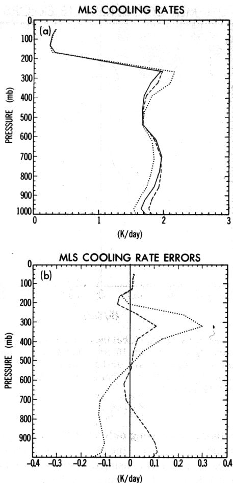
Fig. 10. (a) Same as Figure 8a, but absorption from \text{H}_2\text{O} (lines only) is included. (b) Same as Figure 8b, but absorption from \text{H}_2\text{O} (lines only) is included.
