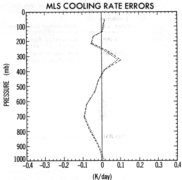
Fig. 17. Same as Figure 14, but the dotted line gives errors for the SEA calculation using 10 cm -1 bands for the random CTS term, while the dashed line gives errors for the SEA88 algorithm described in (19) and related text.
