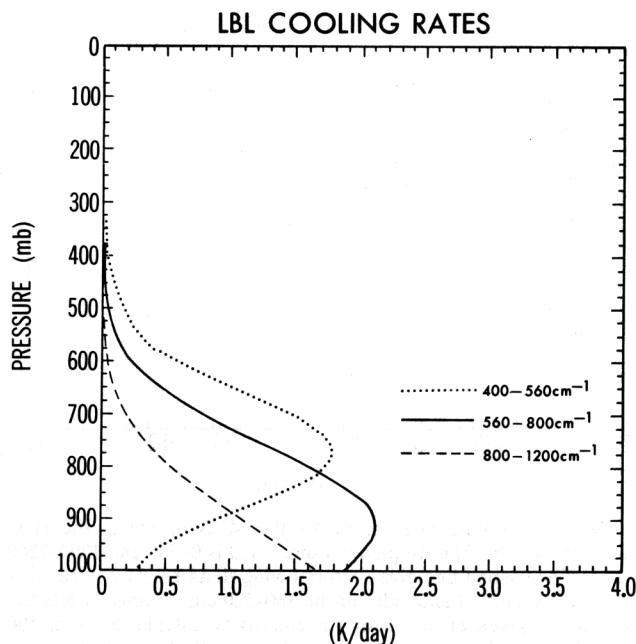
Fig. 12. Same as Figure 11, but the absorber is \text{H}_2\text{O} (continuum), and the frequency ranges included are 400–560, 560–800, and 800–1200 \text{cm}^{-1} .
