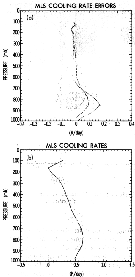
Fig. 23. (a) Cooling rate errors for the MLS profile in the 560\text{--}800\text{ cm}^{-1} range. Absorbers are \text{CO}_2 and \text{H}_2\text{O} (lines plus continuum). The dotted line is the one-band ( Q_{\text{app}} ) error, and the dashed line the error of the SEA88 calculation. The LBL cooling rates are given in Figure 23b. (b) LBL cooling rates for the MLS profile in the 560\text{--}800\text{ cm}^{-1} range. Absorbers are \text{CO}_2 and \text{H}_2\text{O} (lines plus continuum). Middle atmosphere results are not shown, since the vertical resolution used for these calculations is 20 mbar.
