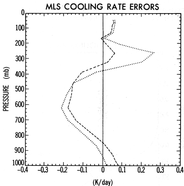
Fig. 14. Cooling rate errors for the MLS profile in the \text{H}_2\text{O} (lines only) case. The frequency range used is 0\text{--}560 and 1200\text{--}2200 \text{cm}^{-1} . The dashed line gives errors owing to an emissivity calculation with 10 \text{cm}^{-1} bandwidth in the 160\text{--}560 \text{cm}^{-1} range, while the dotted line gives errors using an emissivity calculation with 100 \text{cm}^{-1} bandwidth in the 160\text{--}560 \text{cm}^{-1} range. Both calculations use the same bandwidth in the rest of the frequency range. Differences are given as Q - Q(\text{LBL}) , as in Figure 7a. The LBL cooling rates are shown in Figure 11.
