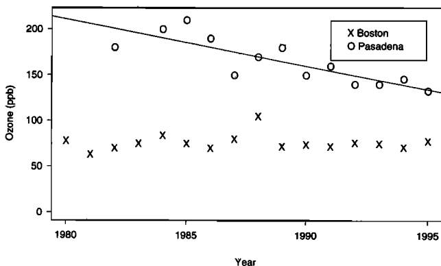
Figure 2. 1980-1995 trends of summer afternoon O 3 concentrations (90 th percentile) in Pasadena, California, and Boston, Massachusetts. The Pasadena data show a significant decreasing trend ( r^2 = 0.68 ; slope = -5.1 \text{ ppb yr}^{-1} ), while the Boston data do not ( r^2 = 0.01 ).
