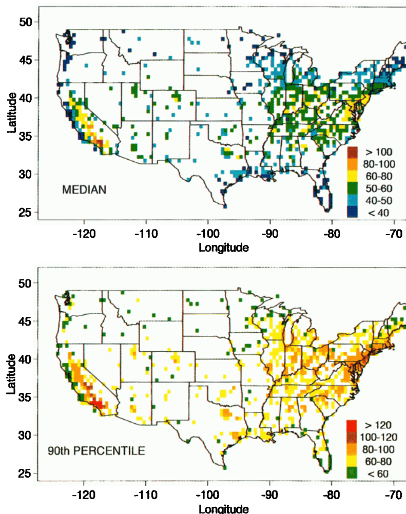
Plate 1. Summer afternoon O_3 concentrations (ppb) in surface air over the United States: (top) medians and (bottom) 90th percentiles. The maps were constructed from observations at 13-16 local time in June-August 1980-1995 for the sites of the EPA AIRS network. Data from individual sites were averaged over 50 \times 50 \text{ km}^2 grid squares.
