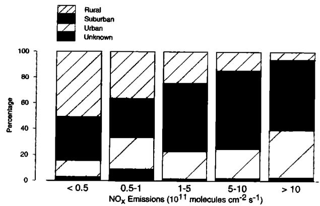
Figure 3. Relationship between the EPA/AIRS classification of sites (“urban,” “suburban,” “rural,” “unknown”) and the NAPAP NO x emission inventory for 1985. Sites with NO x emissions in a given range were sorted according to the EPA/AIRS classification.
