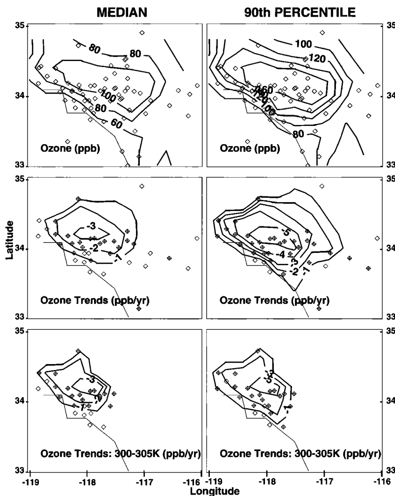
Figure 4b. Same as Figure 4a but for the Los Angeles Basin.
