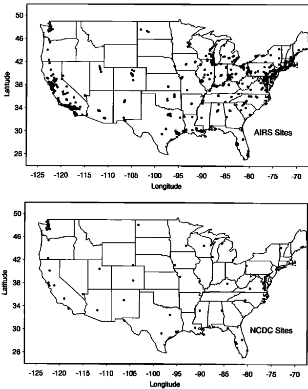
Figure 1. Ozone (EPA/AIRS) and temperature (NCDC) sites used in the trend analysis.
