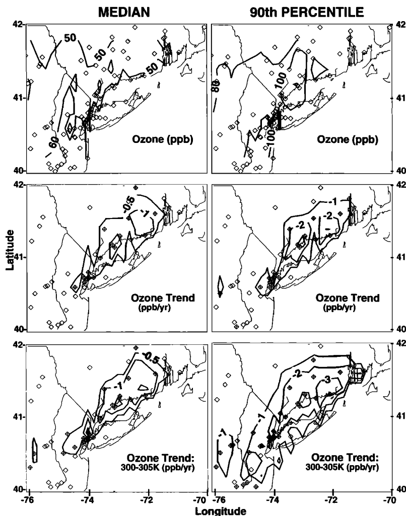
Figure 4a. Spatial distributions of O 3 concentrations and trends for the New York City metropolitan area in 1980-1995. The top panels show the median and 90 th percentile summer afternoon concentrations, the middle panels show the corresponding trends, and the bottom panels show the trends in the temperature-segregated data (300-305 K temperature bin). Diamonds show the individual data sites; there are fewer trend sites than concentration sites because of the data density requirement. Crossed diamonds in the middle and lower panels indicate sites with significant decreasing trends.
