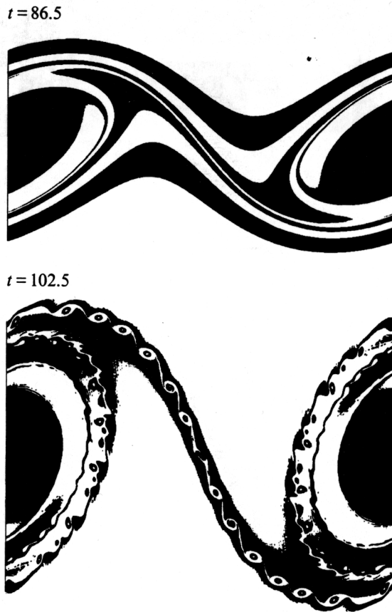
FIGURE 5. An unstable temperature filament, with the initial condition (21); temperatures shown at t = 86.5 and 102.5 .
