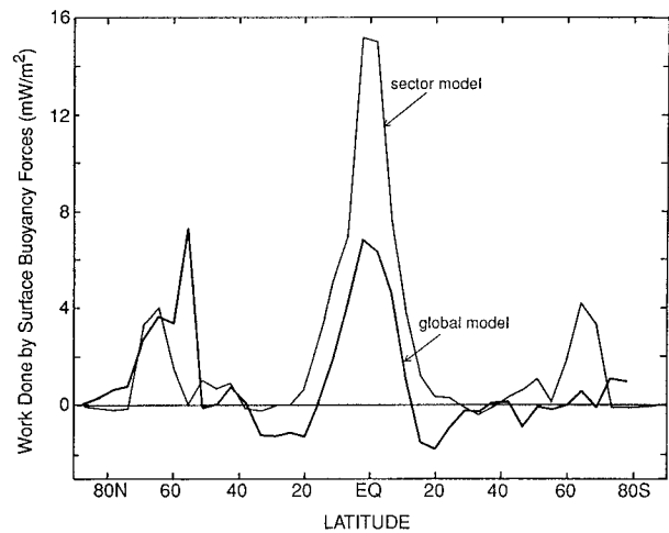
FIG. 7. Work done by surface buoyancy forces (heating/cooling plus freshening/salinification) in the standard global model and the sector model S1.0 plotted as a function of latitude. Results are simple zonal averages ( 10^{-3} W \text{m}^{-2} ).
