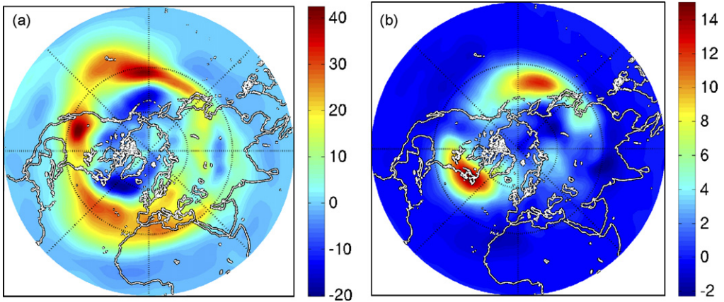
Fig. 3. Left: the eddy momentum fluxes at 250 hPa ( \text{m/s}^2 ). Right: the eddy heat fluxes at 500 hPa ( \text{mK/s} ), for the Northern Hemisphere winter (DJF). Both sets of data are band-pass filtered, allowing variability from 2 to 10 days, from the NCEP/NCAR re-analysis. Red values are large, blue values weak or negative.
