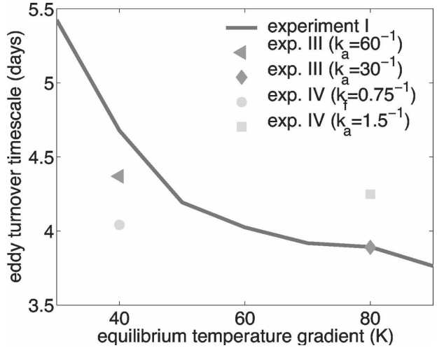
FIG. 4. The eddy turnover time scale, L/K^{1/2} , as a function of the equilibrium temperature gradient, \Delta T_{\text{eq}} . The eddy kinetic energy, K , increases linearly with the equilibrium gradient, while the eddy length scale is roughly constant. Hence the curve is proportional to \Delta T_{\text{eq}}^{-1/2} . Values for four other zonally symmetric simulations in experiments III and IV (where k_a and k_f were varied, respectively) are shown for comparison. The points were plotted near the simulation from experiment I that had the most similar climatology and intraseasonal variability.
