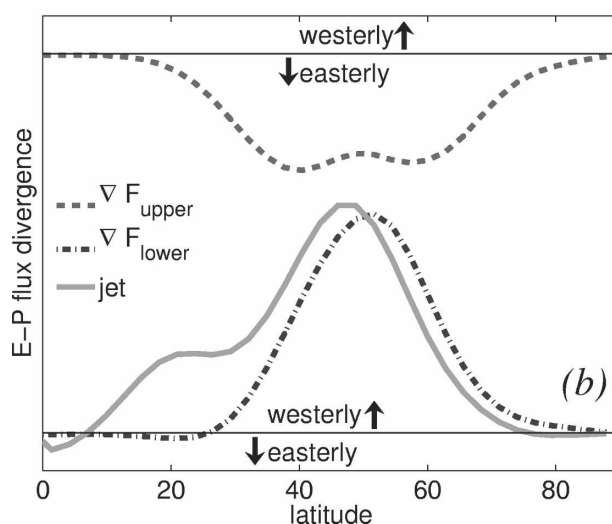
FIG. 13. Evidence for the eddy-mean flow interaction in the control simulation. Composites based on (a) weak and (b) strong zonal index events, as determined by a threshold of \pm 1 std dev of the zonal index Z_i(t) . The dot-dashed curves show the acceleration of the zonal average flow, \nabla\mathbf{F} , by 2–10-day bandpass eddies averaged over the lower half of the atmosphere. The torque is westerly at nearly all latitudes. The dashed curves show the acceleration of the upper half of the atmosphere; a negative (easterly) torque. The solid curves show composites of the upper-level jet: \bar{u} averaged over the upper half of the atmosphere.
