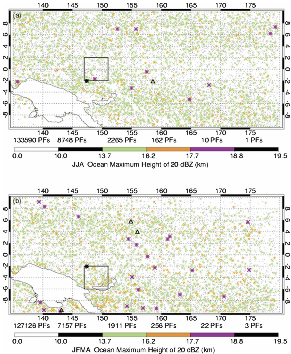
FIG. 20. Distribution of PFs in the TRMM database over the tropical western Pacific region. The 4^\circ \times 4^\circ boxes used for each season are shown; the black asterisk locates the Manus MMCR site. The color code shows the maximum height reached by the 20-dBZ contour for each PF, progressing from small black dot–green dot–orange diamond–purple asterisk–black triangle for increasingly rare and intense PFs (see text).
