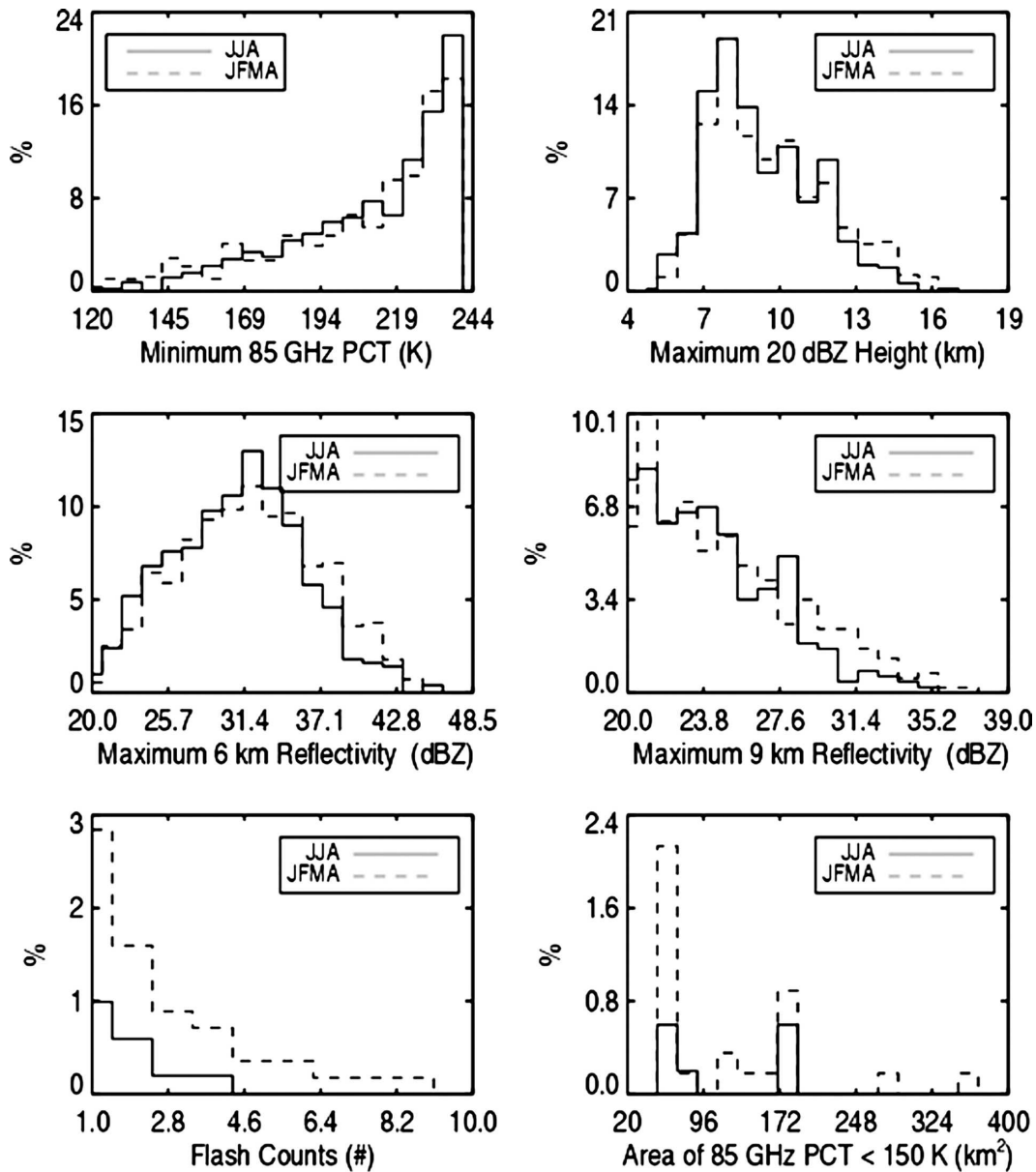
FIG. 19. Relative frequencies of occurrence of convective intensity proxy indicator magnitudes for precipitation features in the TRMM database within 4^\circ \times 4^\circ boxes noted in Fig. 20. Table 4 provides additional information. The box north of Manus is used in June–August; south of Manus in January–April.
