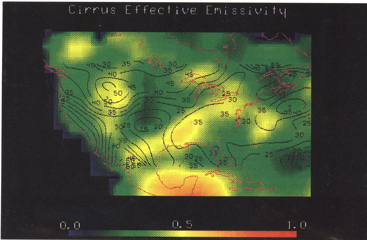
Plate 3. Map of the predicted emissivity from the HD parameterization overlain by contours of effective emissivity from the CO 2 -slicing technique.
