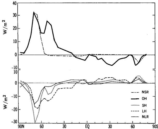
FIG. 18. Latitudinal distributions of the difference in various surface heat balance components zonally averaged over the Atlantic Ocean. Units are W m^{-2} . See explanation of Fig. 17 in text for sign convention.
