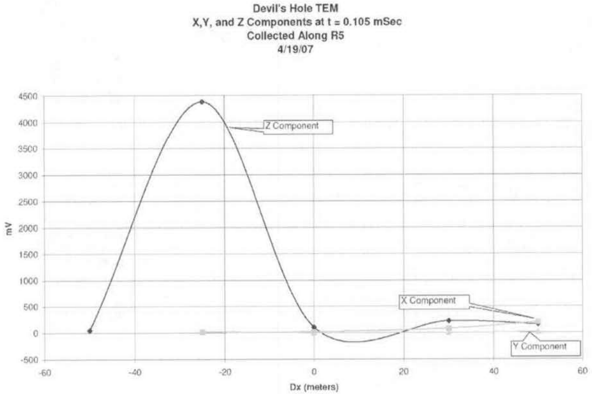
Figure 18. Graphical Analysis of Three-Component TEM Data Along Resistivity Line R5.
