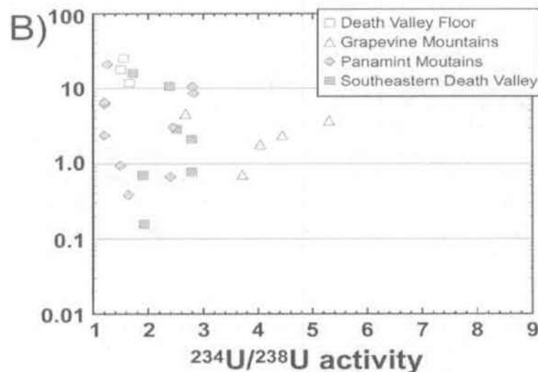
Plots of uranium concentrations versus ^{234}\text{U}/^{238}\text{U} activity ratios for saturated-zone waters. A) Regional ground water in the Yucca Mountain vicinity (from Paces and other, 1998). B) Death Valley springs. Southeastern Death Valley category includes Navel Spring and Upper Navel Seep, Willow Spring, Salisbury Spring, Ibex Spring, Saratoga Spring, and Owl Hole Spring.
