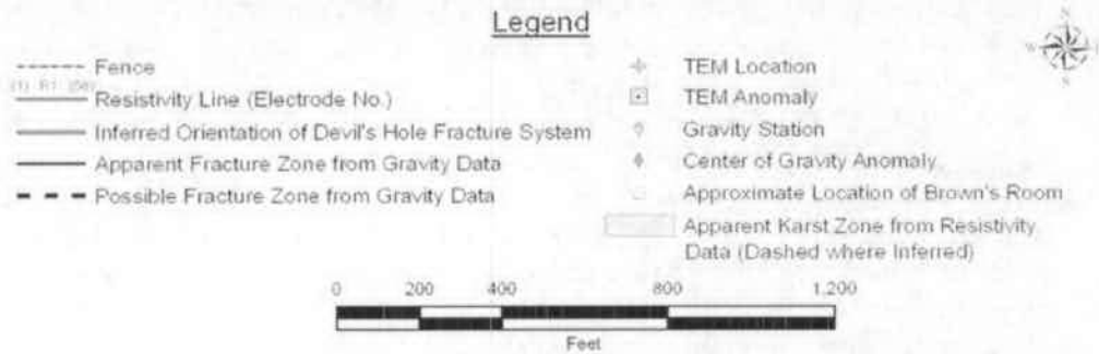
Figure 17. Interpreted Geophysical Anomalies in the Devil's Hole Area.
