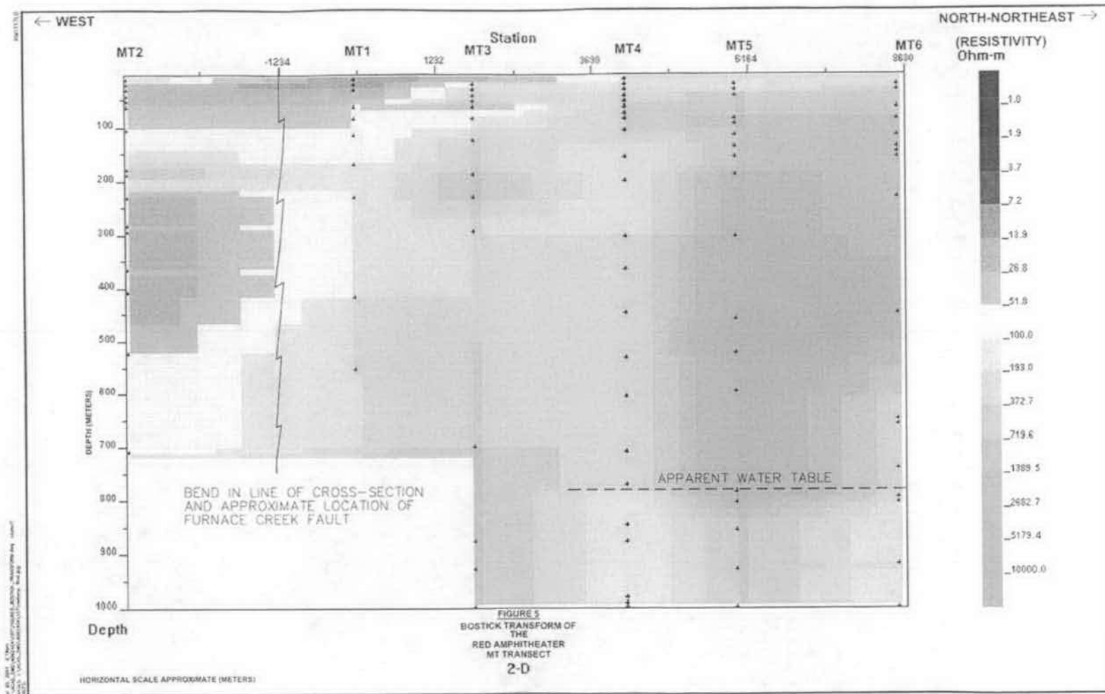
Figure 9. 2d Bostic Transform Interpretation of Red Amphitheater Transect.
