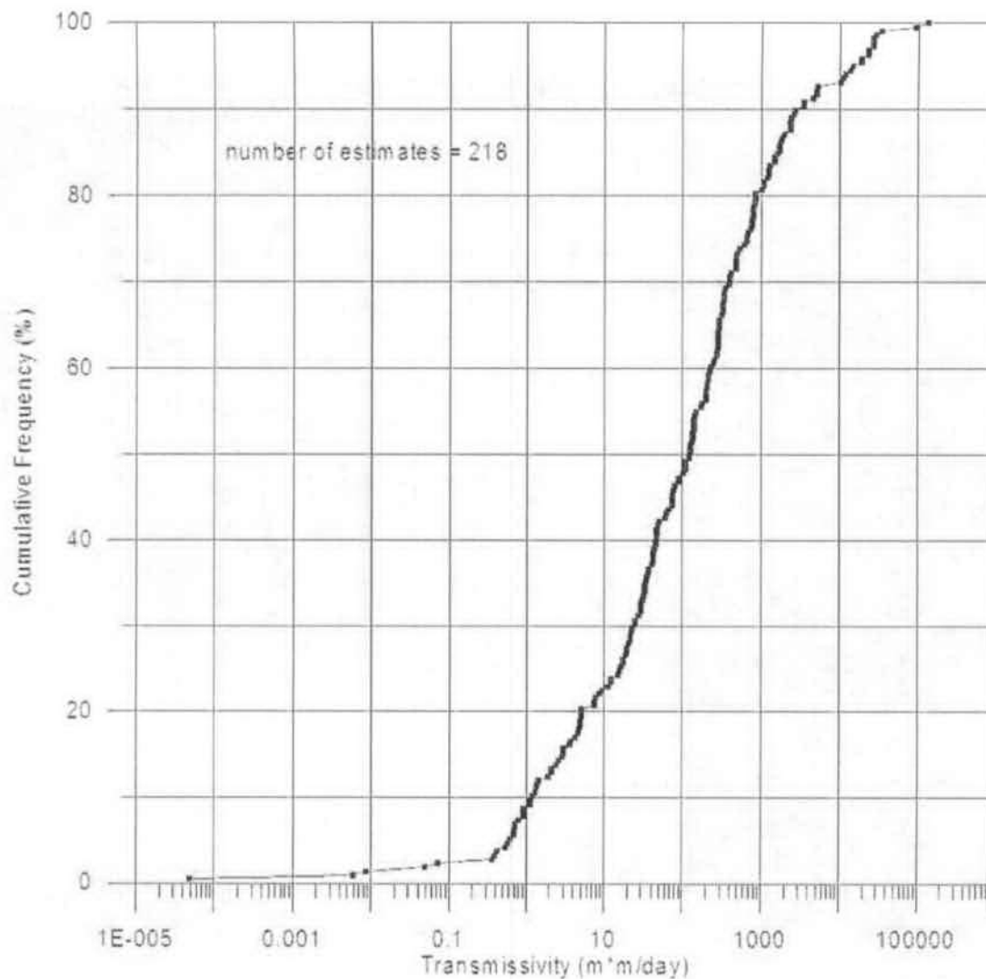
Figure 35. Cumulative Distribution of Transmissivity from SNWA Data (SNWA, 2006).
