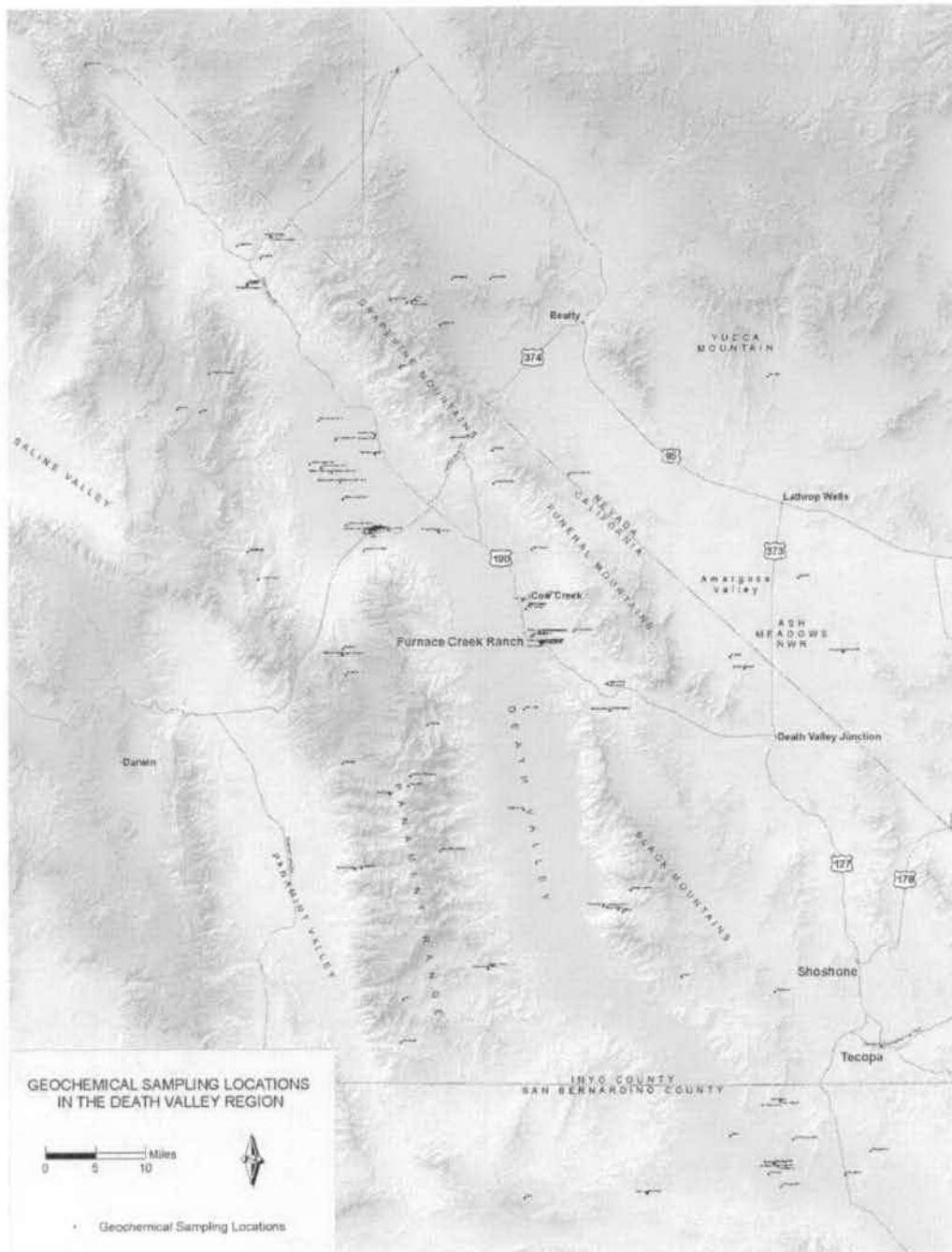
Figure 20. Location of Death Valley Regional Geochemical Data Collection Point.
