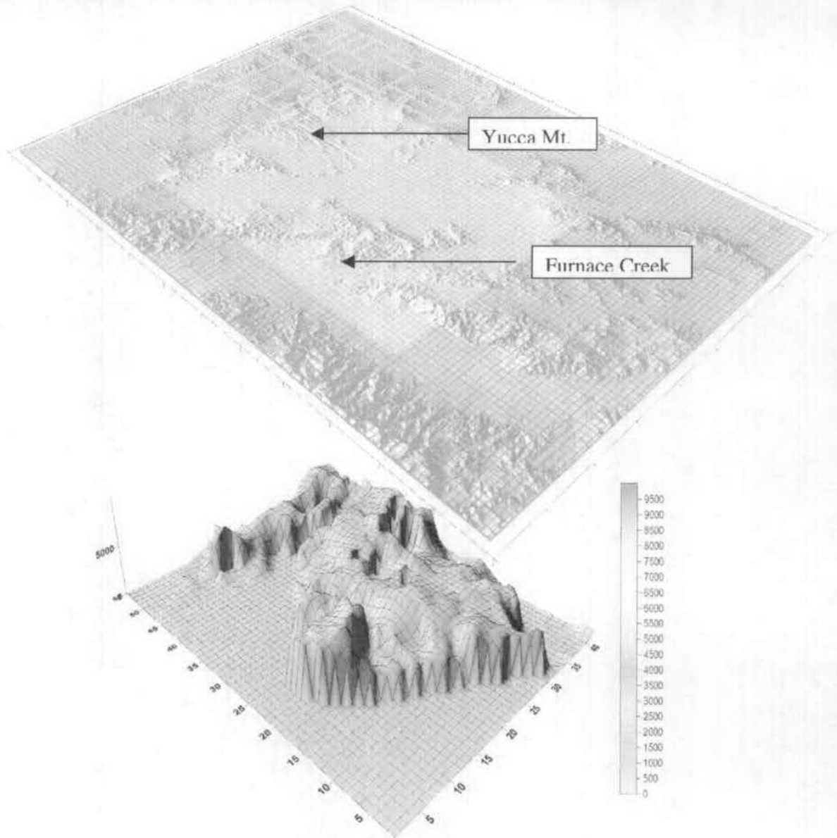
Figure 34. Thickness of the Paleozoic Carbonate Rocks in the Sub-Region.
