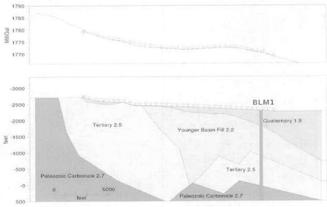
Figure 15. Geological Profile through an Eastern Portion of the Southern Funeral Mountains.
