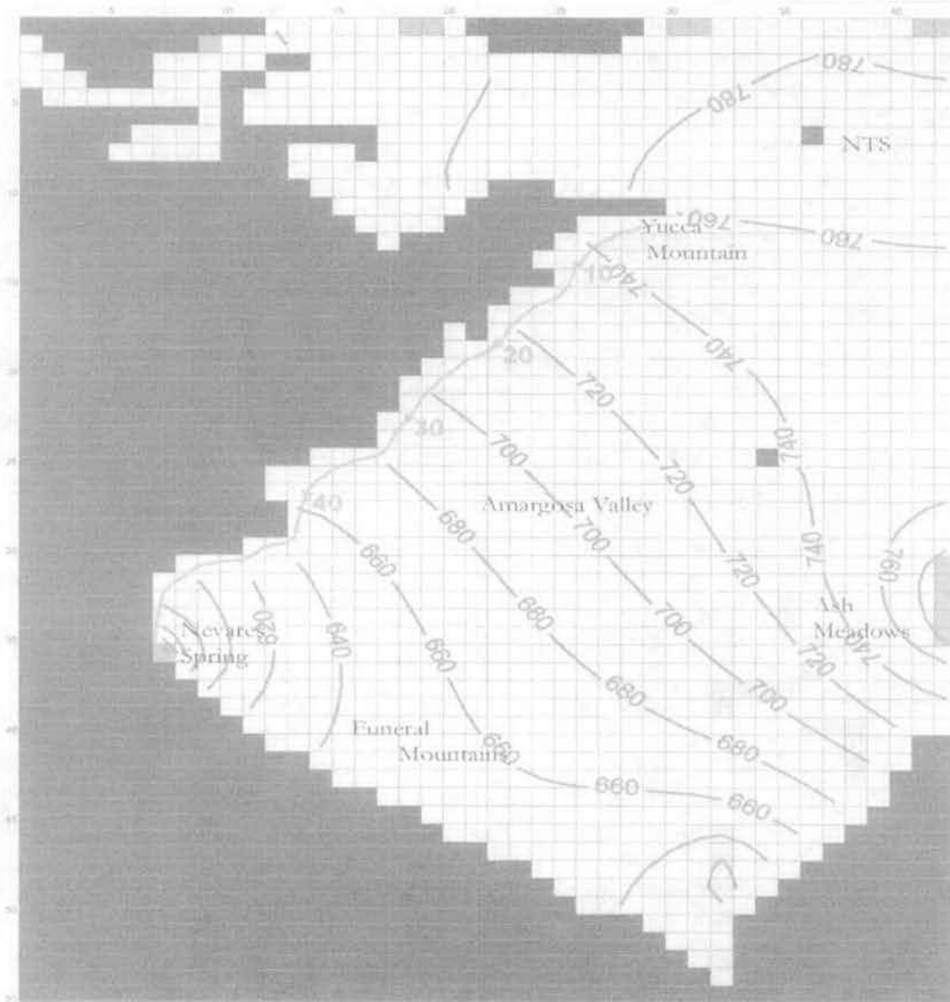
Figure 36. Map of Steady State Hydraulic Head from the One Layer Carbonate Aquifer Model.
