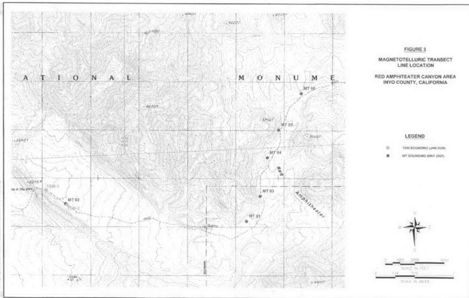
Figure 7. Location of Red Amphitheater Transect Location.
