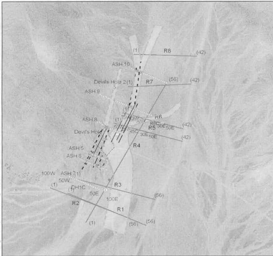
Figure 13 DEVIL'S HOLE AREA INTERPRETED GEOPHYSICAL ANOMALIES APRIL, 2007
