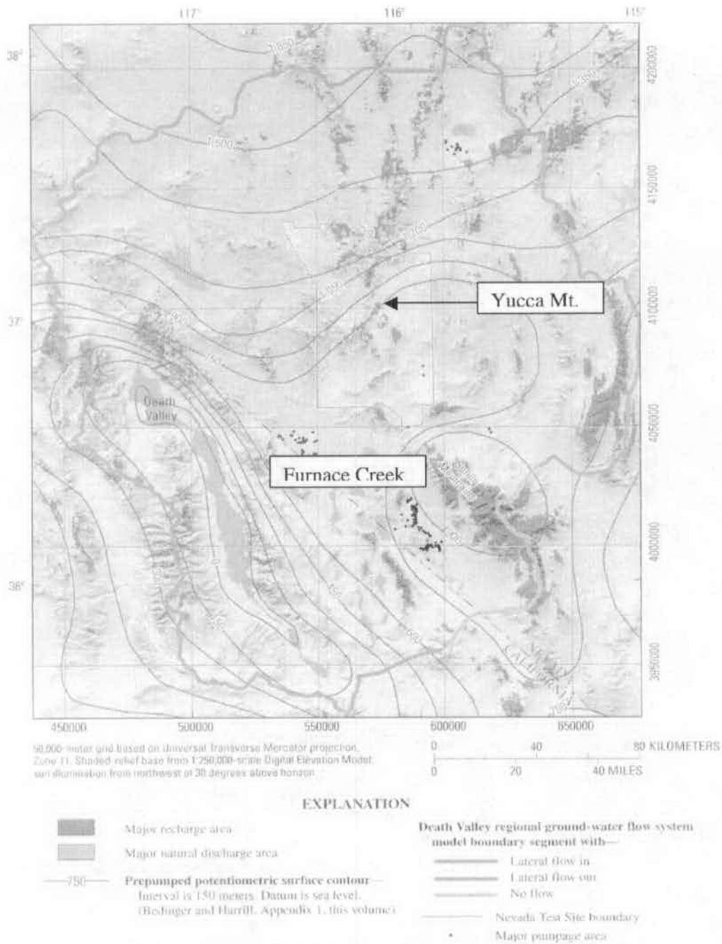
Figure 33. Potentiometric Surface Map for the Area of the U.S.G.S. Death Valley Regional Flow System Model (San Juan, et. al. 2004).
