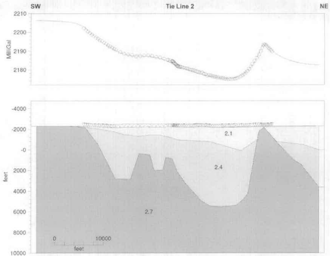
Figure 14. Gravity Model of Tie Line 2. Includes GRAV 15, TIE 2, and ASH 3 data.
