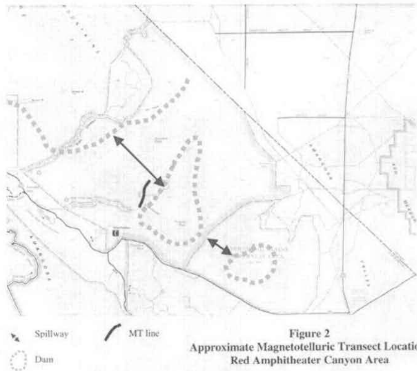
Figure 6. MT Transect through Red Amphitheater – Canyon.
