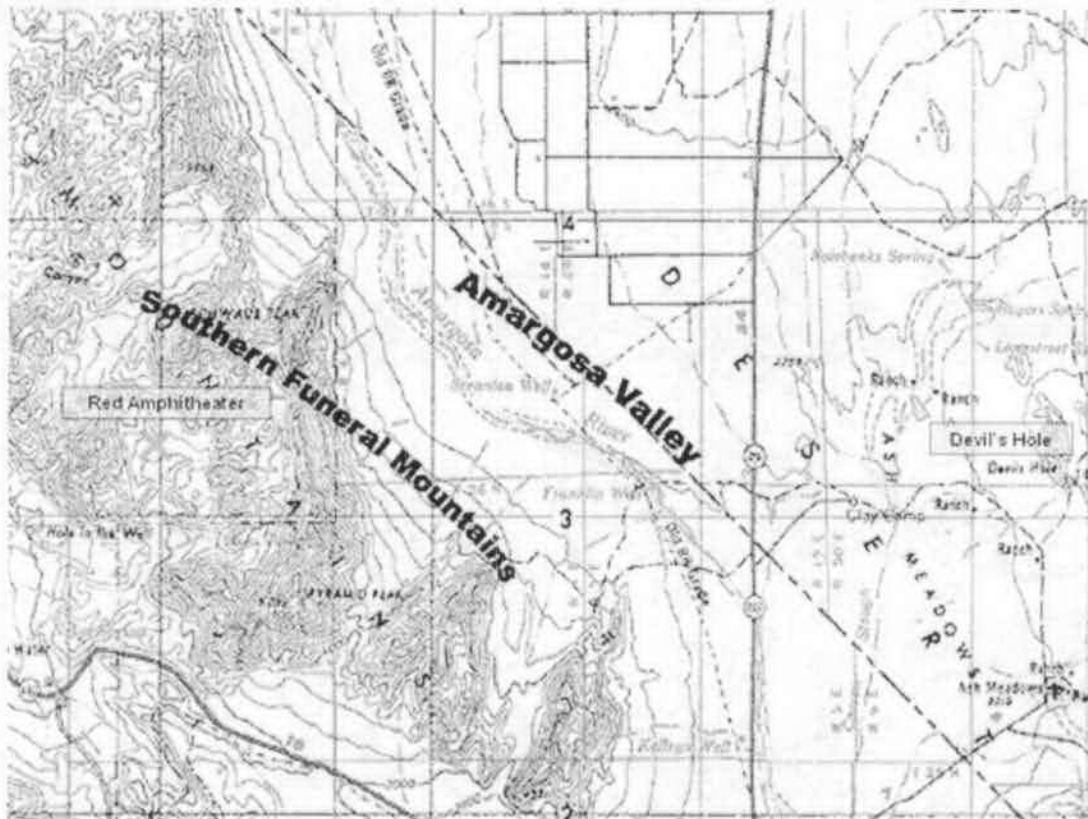
Figure 5. Location Map of Geophysical Survey Area.
