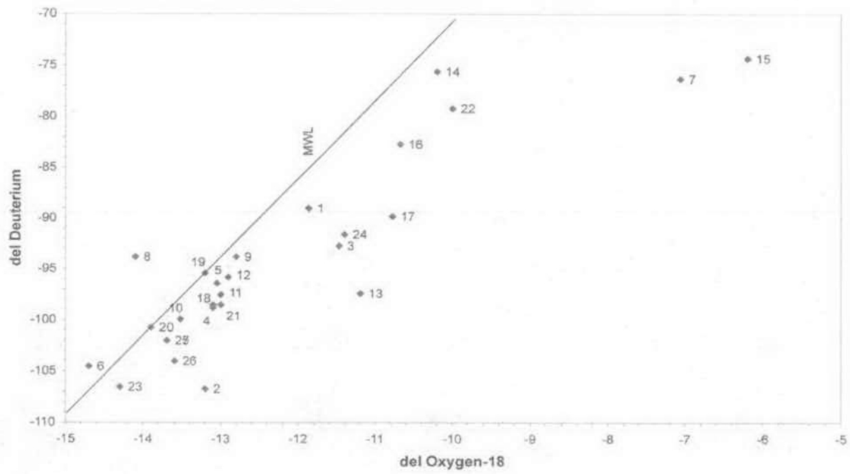
Deuterium and Oxygen-18 Graph of Death Valley Springs
