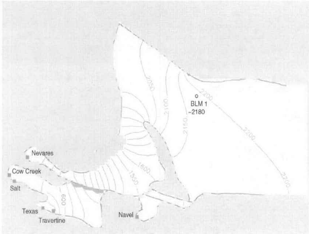
Figure 39. Computed Hydraulic Head in Carbonate Aquifer.
