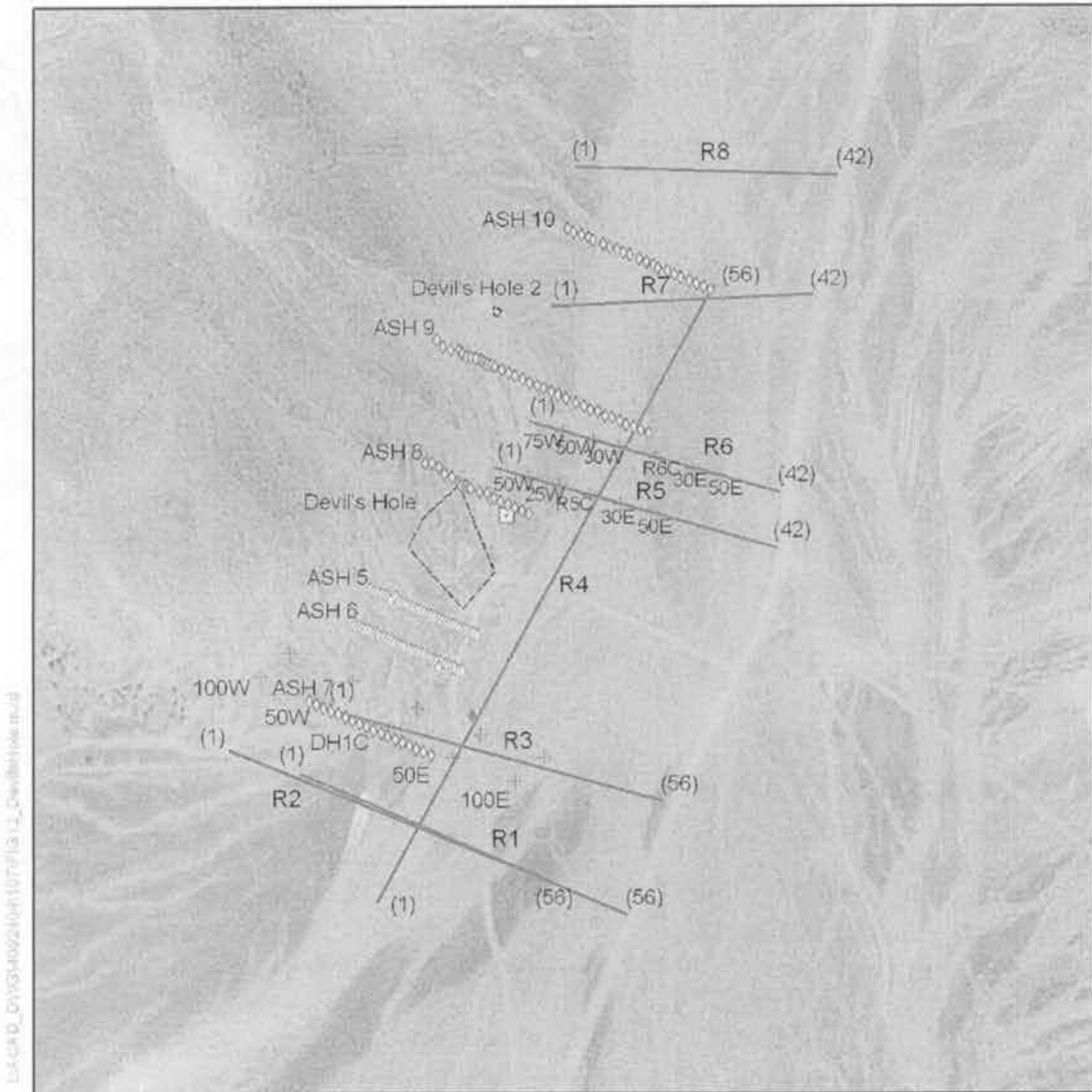
FIGURE 12 DEVIL'S HOLE AREA GEOPHYSICAL SURVEY LOCATIONS APRIL, 2007
