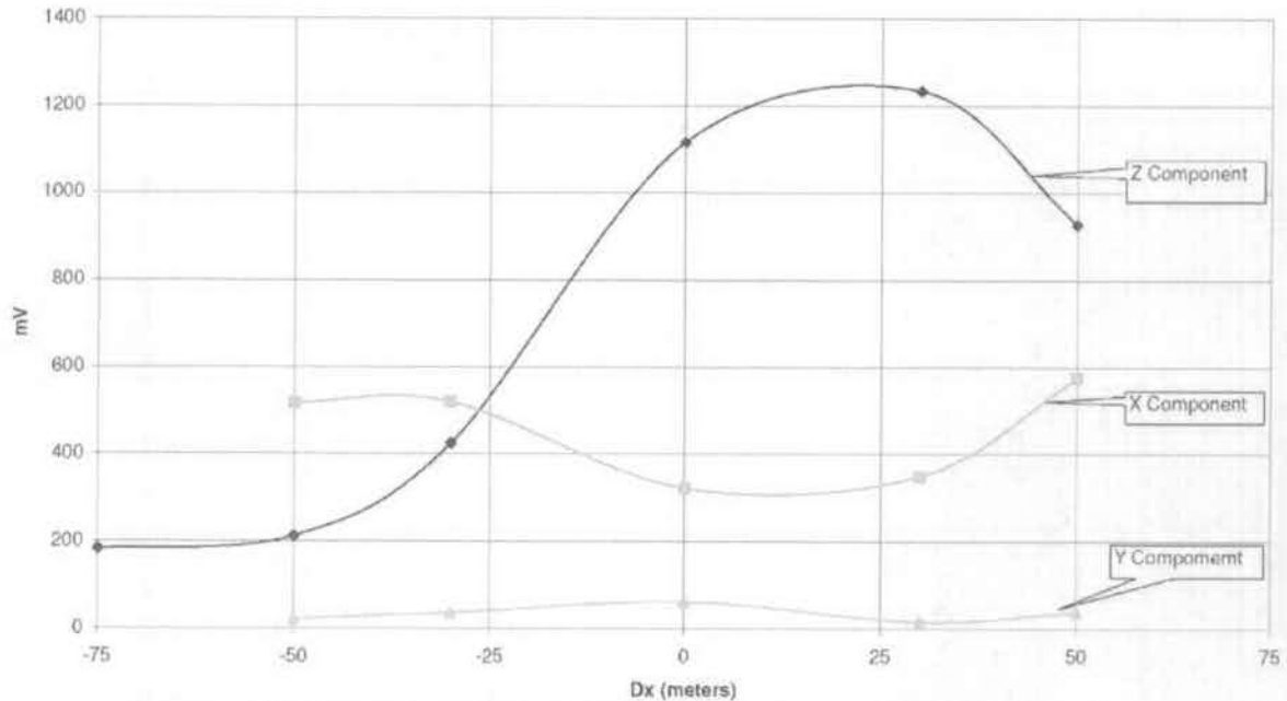
Figure 19. Graphical Analysis of Three Component TEM Data Along Resistivity Line R6.
