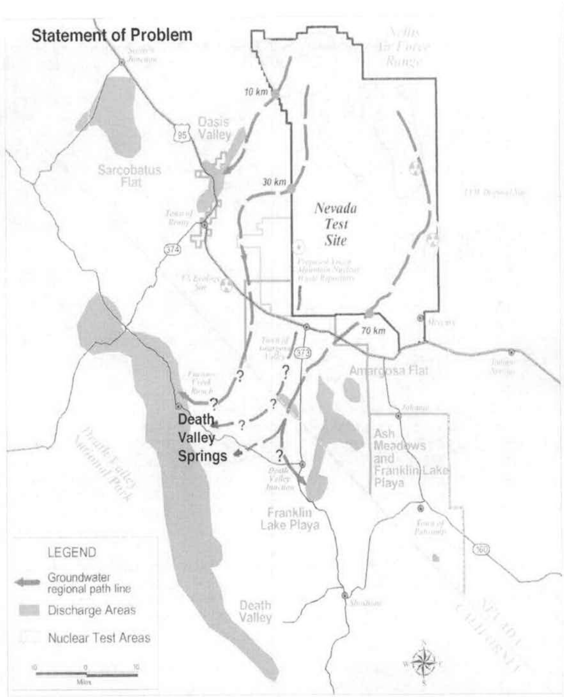
Figure 1. Regional Groundwater Flow Path Line from Yucca Mt. And Nevada Test Site.
