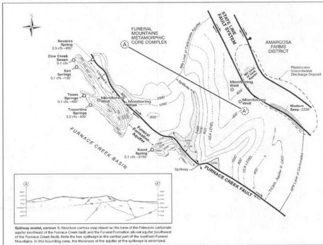
Figure 37. Structure contour map of the base of the Carbonate Aquifer formed by the fault planes with shallow dips.
