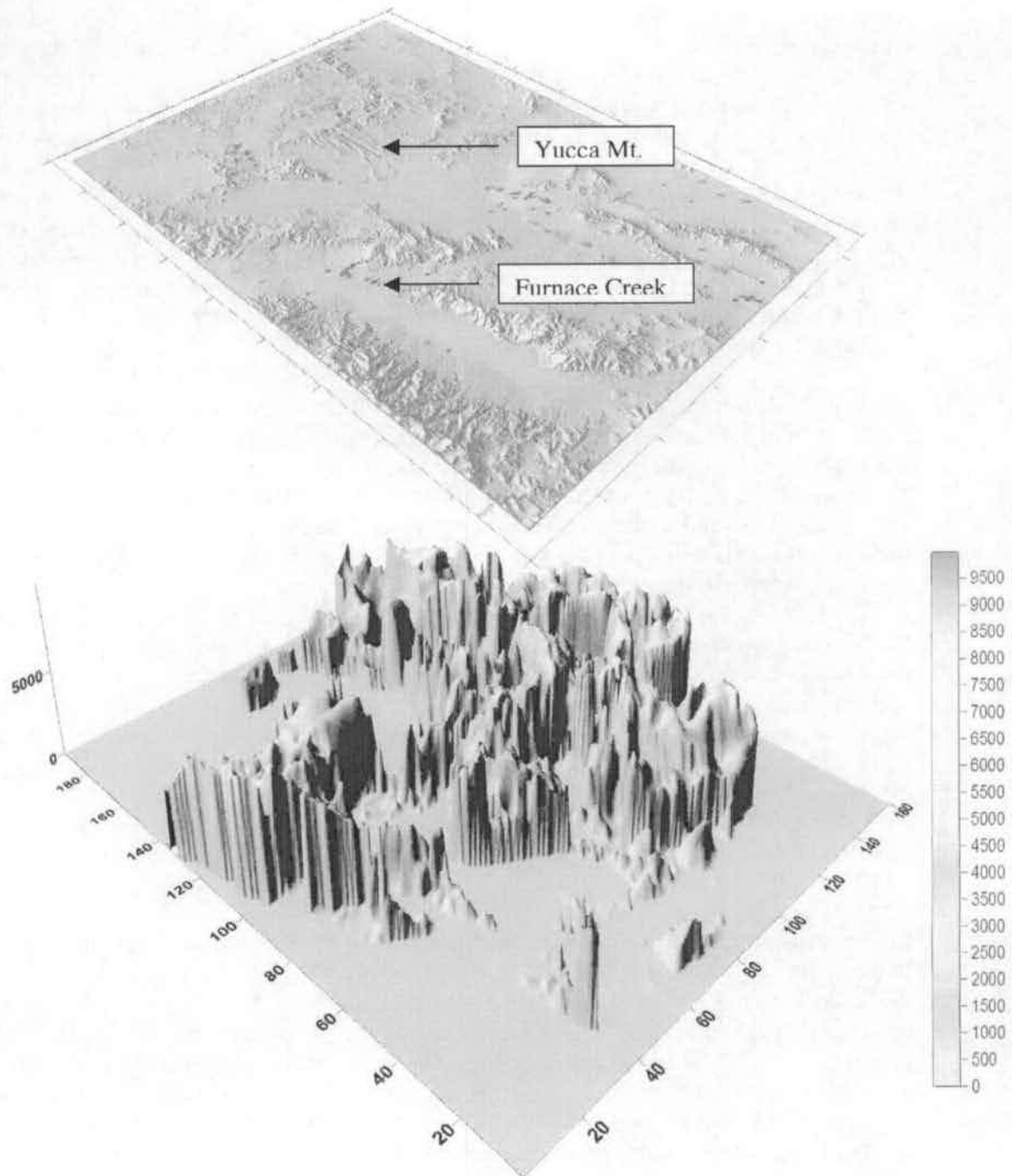
Figure 32. Distribution of Carbonate Rocks in the Death Valley Regional Flow System Model.
