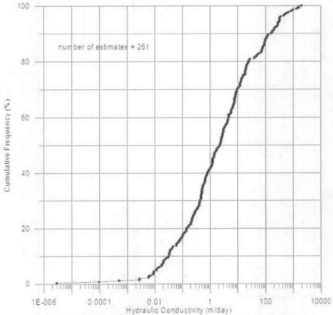
Figure 36. Cumulative Distribution of Hydraulic Conductivity from SNWA Data (SNWA, 2006).
