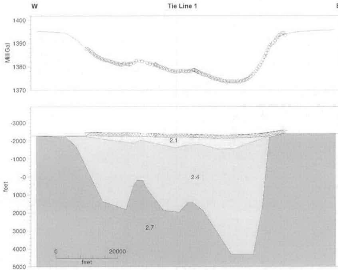
Figure 13. Gravity Model of Tie Line 1. Includes GRAV 14, TIE 1 and ASH 1 data.
