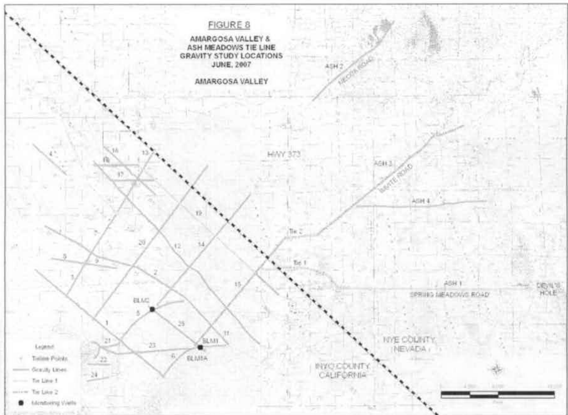
Figure 12. Location of Gravity Tie Line Stations.
