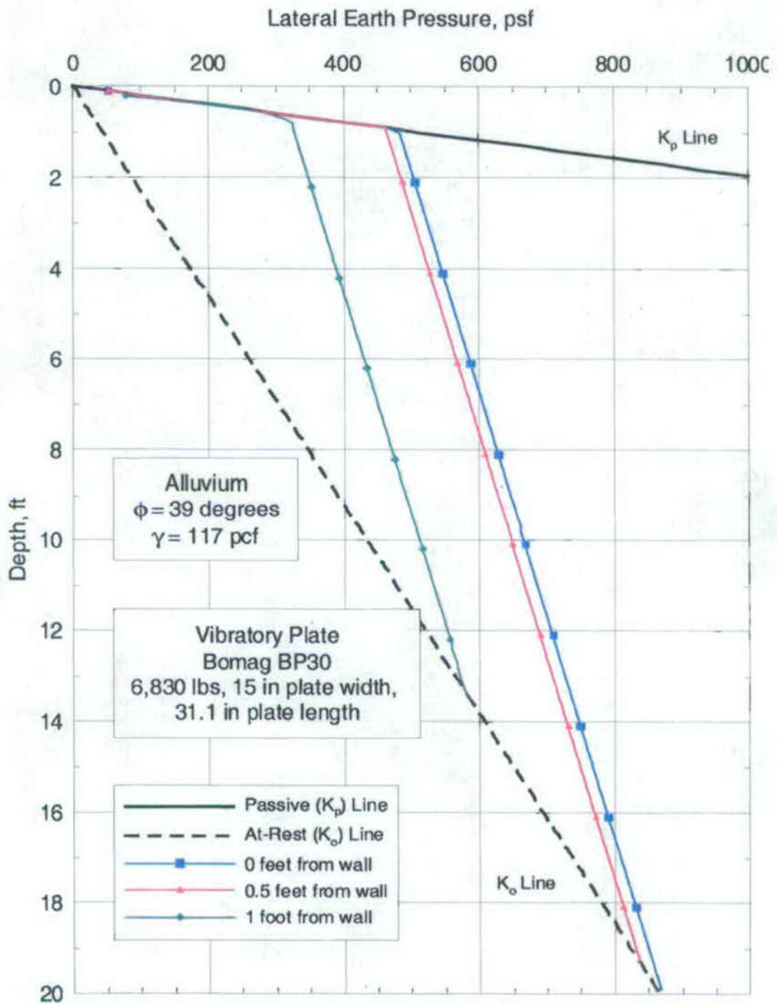
Figure 7-13. Compactor-induced pressures from plate compactor (Bomag BP30).
