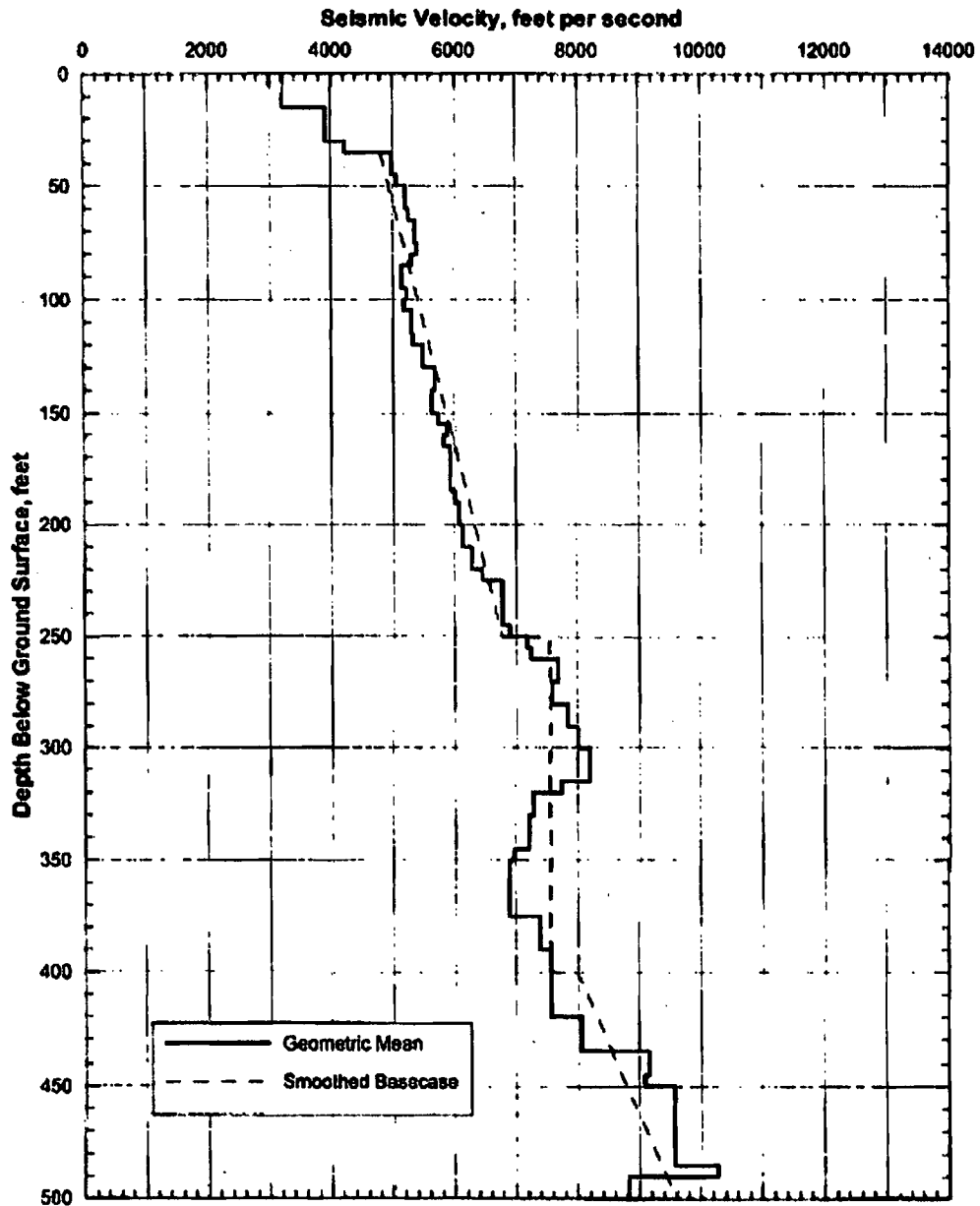
Figure 6-33. Base Case compression wave velocity profile for tuff in the surface facilities area—upthrown block. (Figure 6.2-120 from BSC 2004a)
