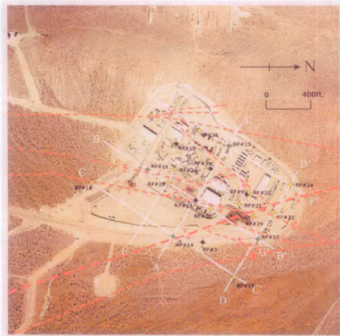
Figure 6-7. Locations of Soil Exploration in the surface facilities area (only pre-2005 borings shown). Cross-Sections shown in Figure 6-4, Figure 6-5, and Figure 7-1.
