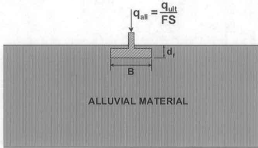
Figure B6-1. Schematic for shallow footing.
