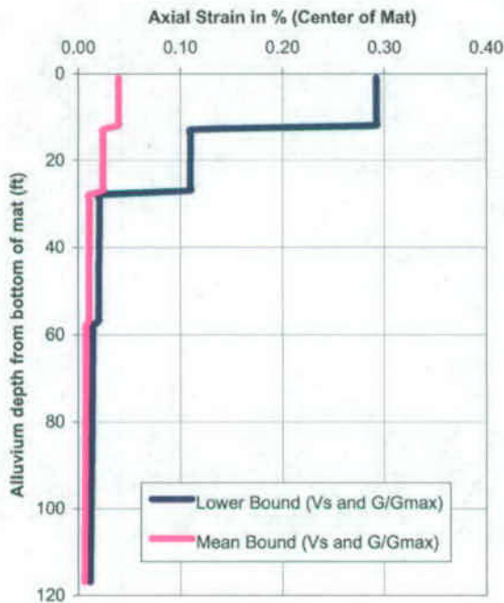
Figure B7-6. Elastic settlement of mat foundation (3 ksf vertical load).
