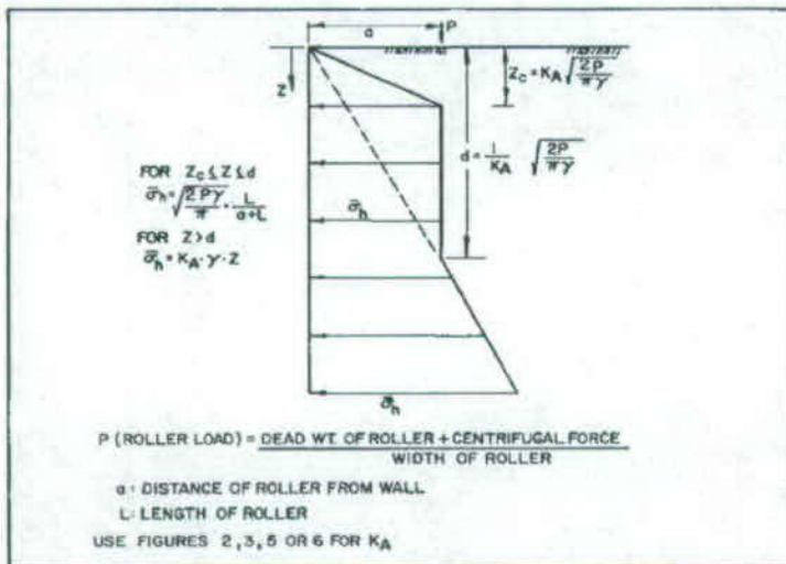
FIGURE 13 Horizontal Pressure on Walls from Compaction Effort
