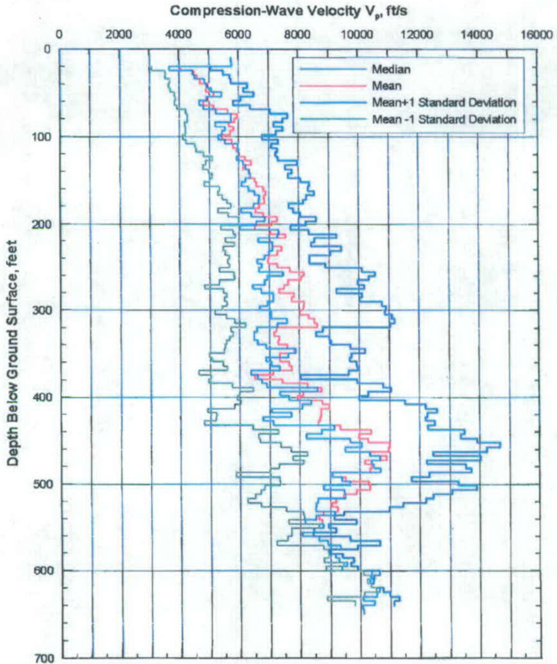
Figure 6-22. Compression wave velocity by depth interval from source to receiver interval suspension surveys in surface facilities area. (Figure 34 of BSC 2002a, DTN: MO02045FTDSUSP.001)
