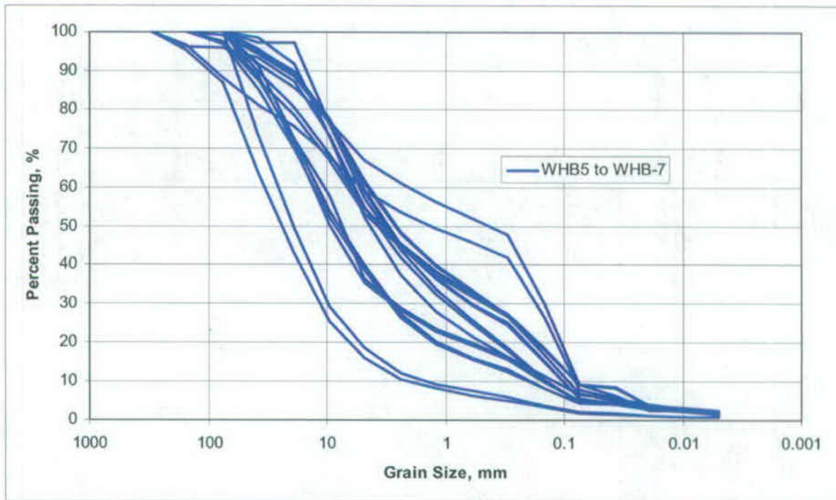
Figure 6-15. Particle-Size Distribution Curves for Alluvium for TP-WHB-5 to TP-WHB-7 (DTN: GS070683114233.004)
