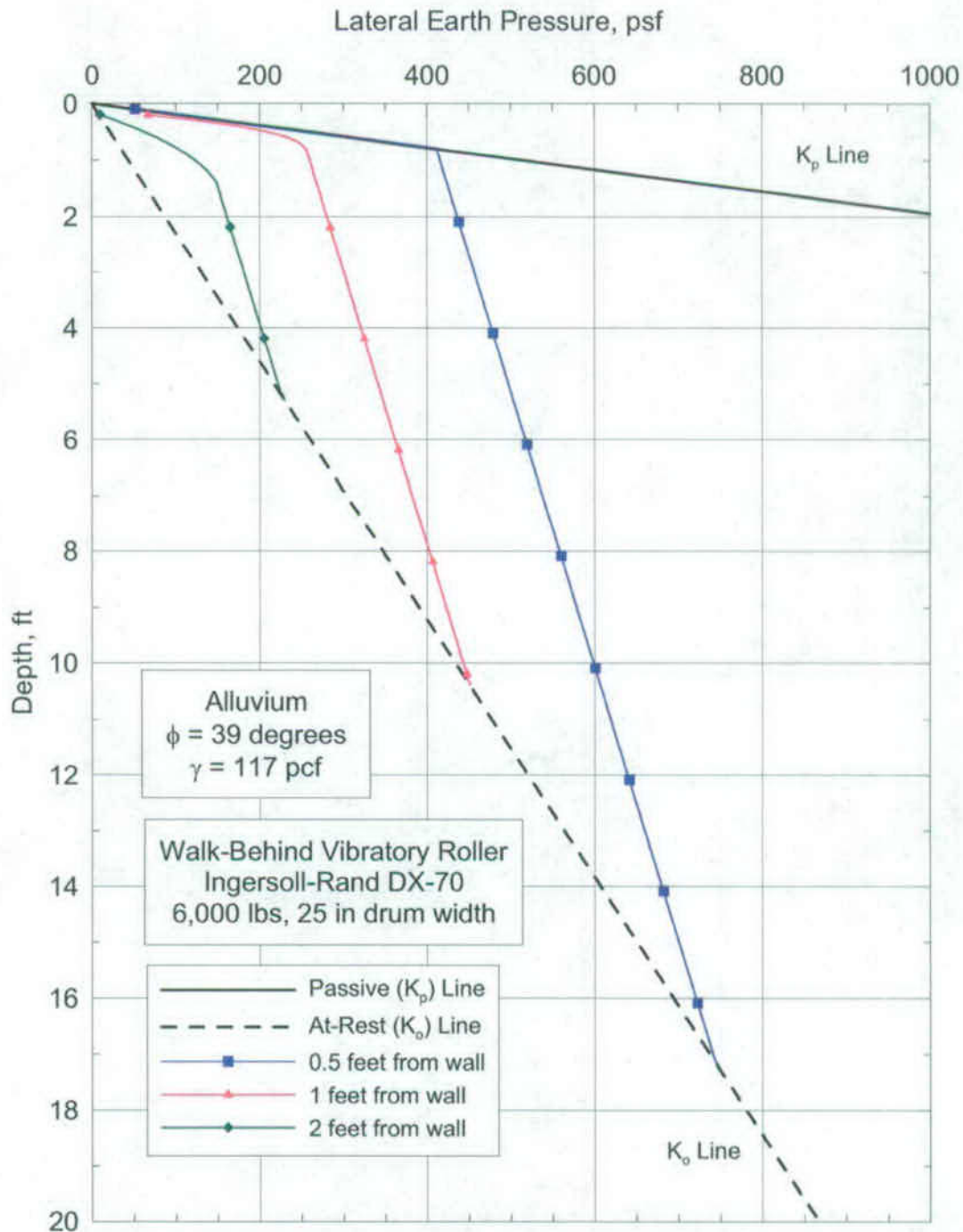
Figure C7-7. Compactor-induced pressures from roller compactor (Ingersoll-Rand DX-70).
