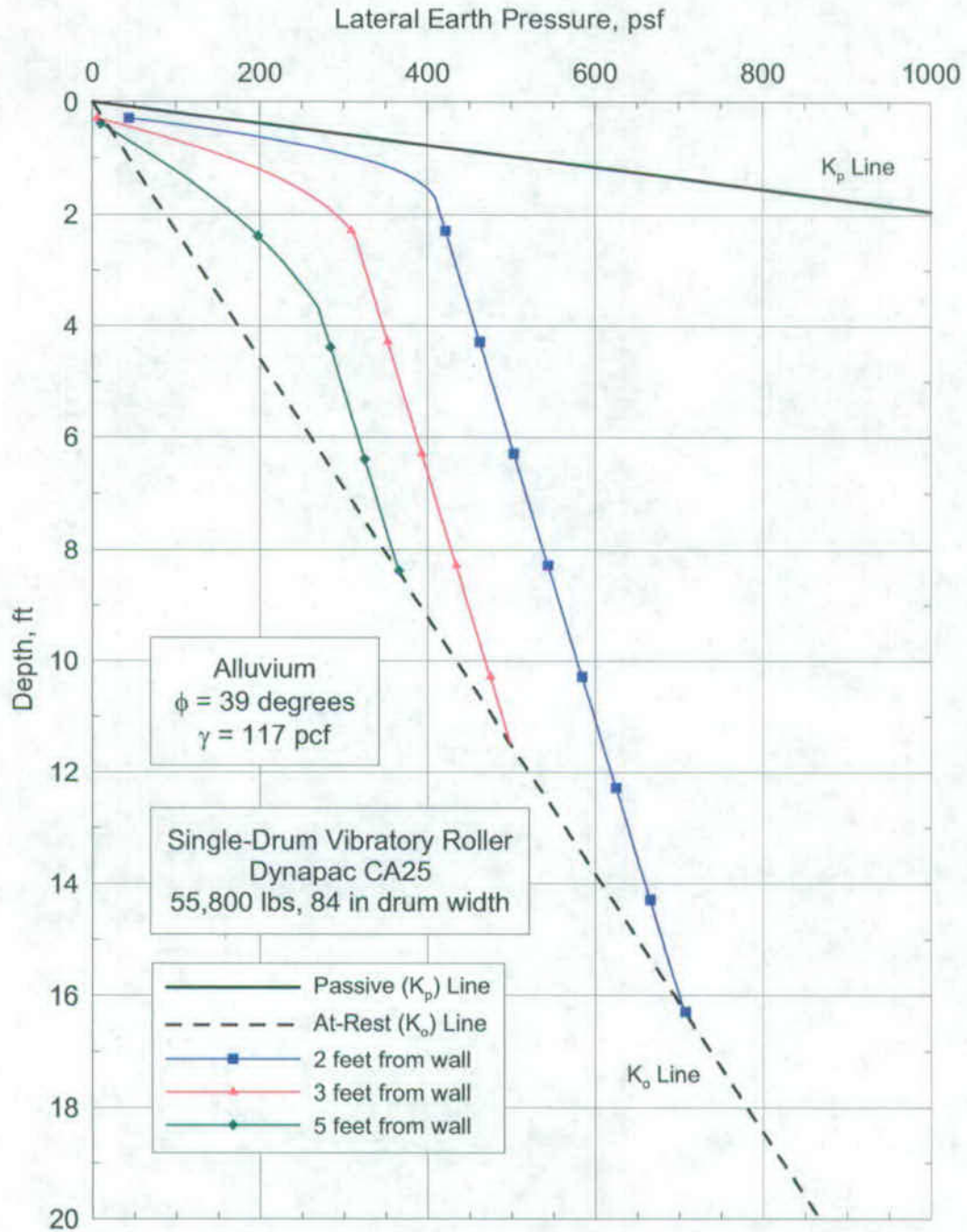
Figure C7-6. Compactor-induced pressures from roller compactor (Dynapac CA25).
