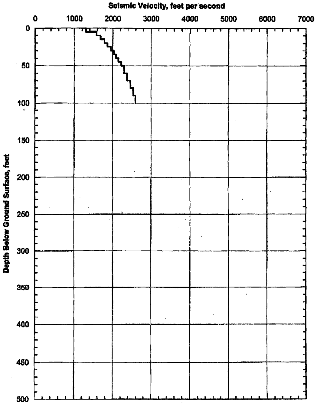
Figure 6-27. Base Case shear wave velocity profile for alluvium in the surface facilities area—upthrown side. (Figure 6.2-121 from BSC 2004a)
