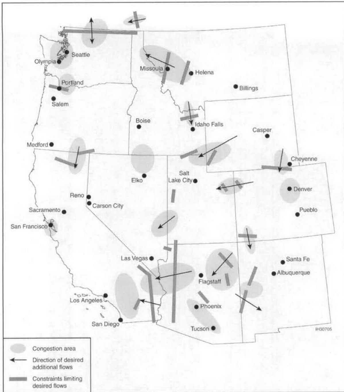
FIGURE 1.1-2 Transmission Constraints Limiting Desired Flows of Electricity, with Arrows Depicting the Direction of Additional Desired Flows That May Be Needed to Reduce Constraints in the West. (The red bars indicate near-term and potential longer-term [10 years] constraints [including congestion] on transmission infrastructure that crosses the bars.) (Source: DOE 2006a)
