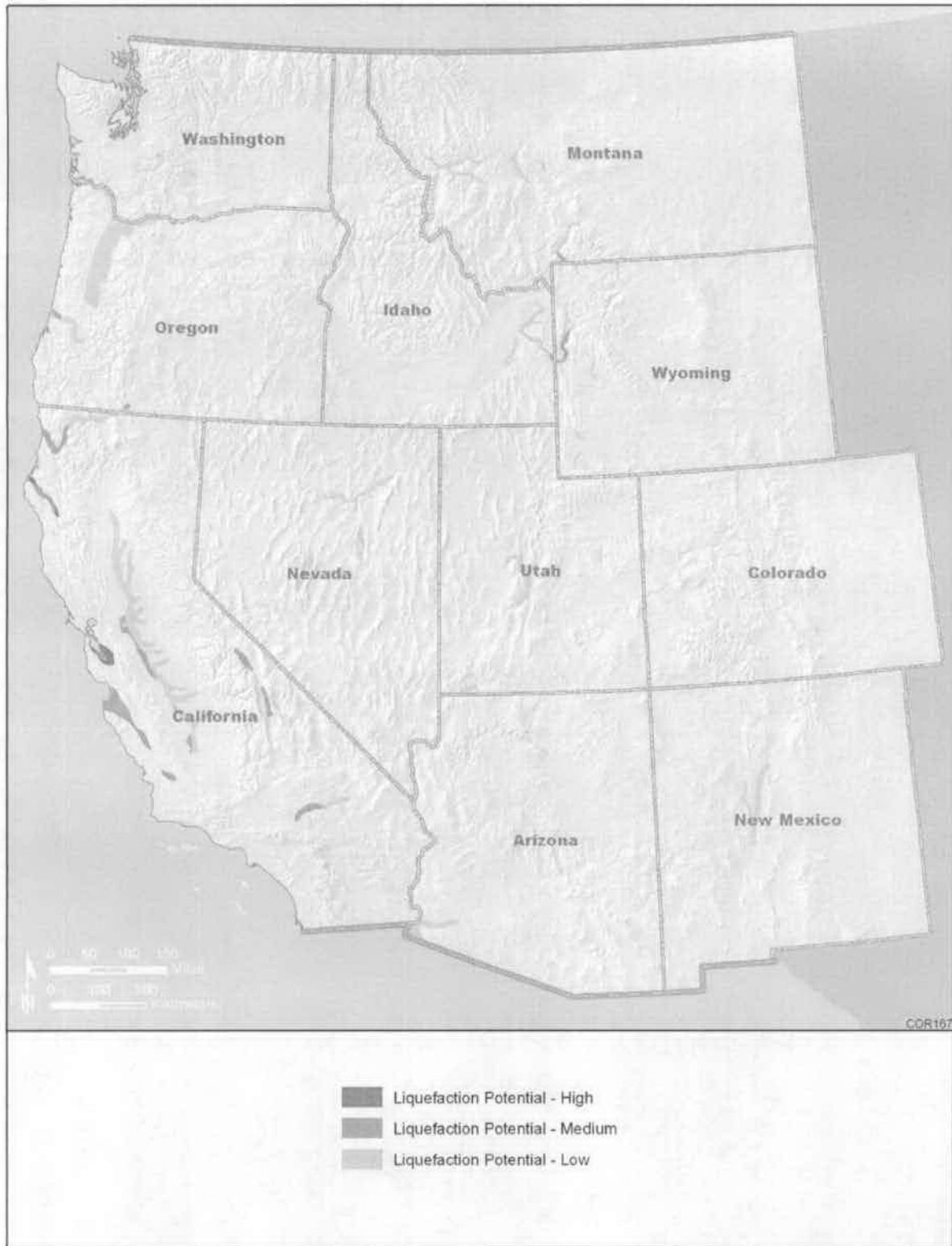
FIGURE 3.3-3 Major Areas with Liquefaction Potential in the 11 Western States (Sources: Modified from SCEC 1999 and National Atlas 2006)
