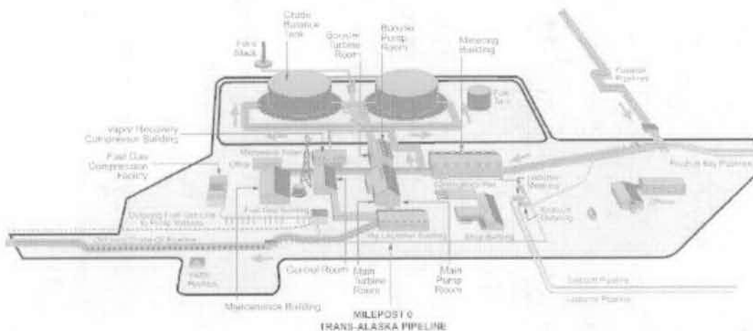
FIGURE 3.9-7 Schematic of Pumping Station
