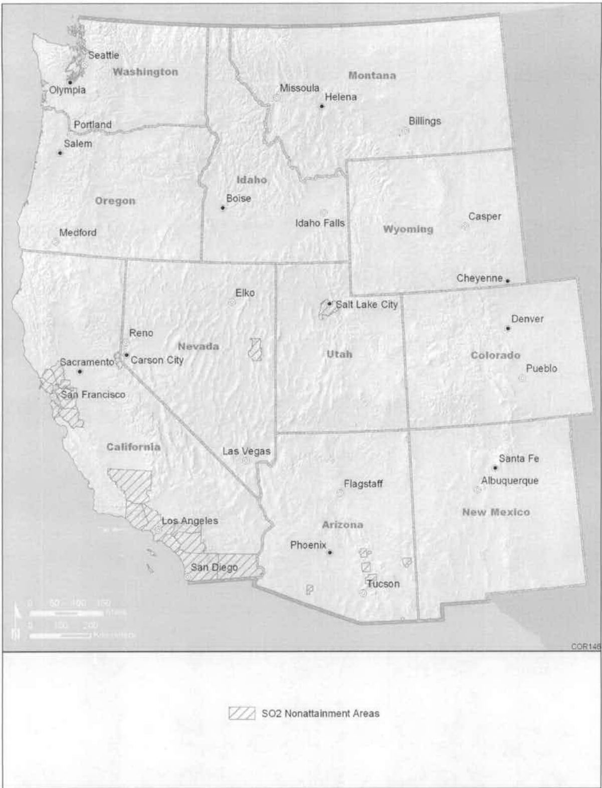
FIGURE 3.6-5 Sulfur Dioxide (SO 2 ) Nonattainment Areas in the 11 Western States
