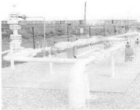
FIGURE 3.9-8 Typical Natural Gas City Gate
