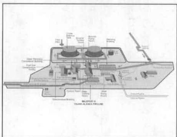
Schematic of pumping station
