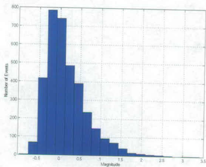
Figure 3. Distribution of earthquake magnitudes from the FY05-06 catalog.
