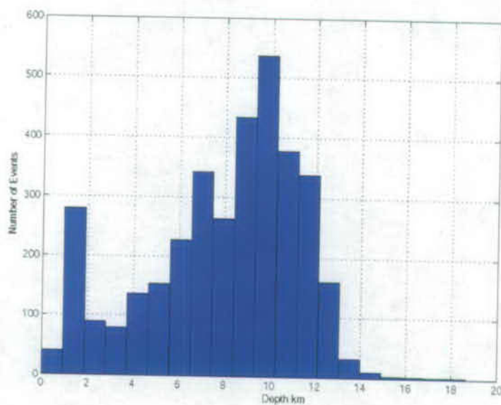
Figure 4. Distribution of hypocentral depths from the FY05-06 catalog.
