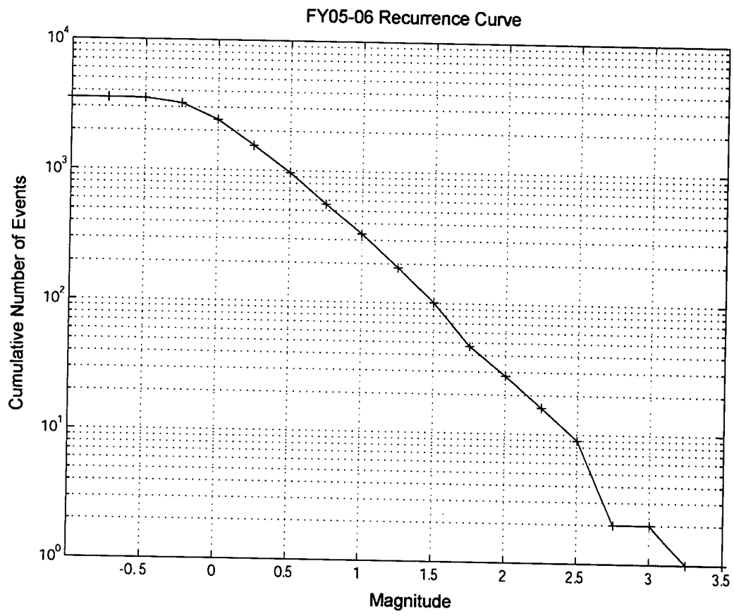
Figure 5. Cumulative magnitude distribution curve for FY05-06.
