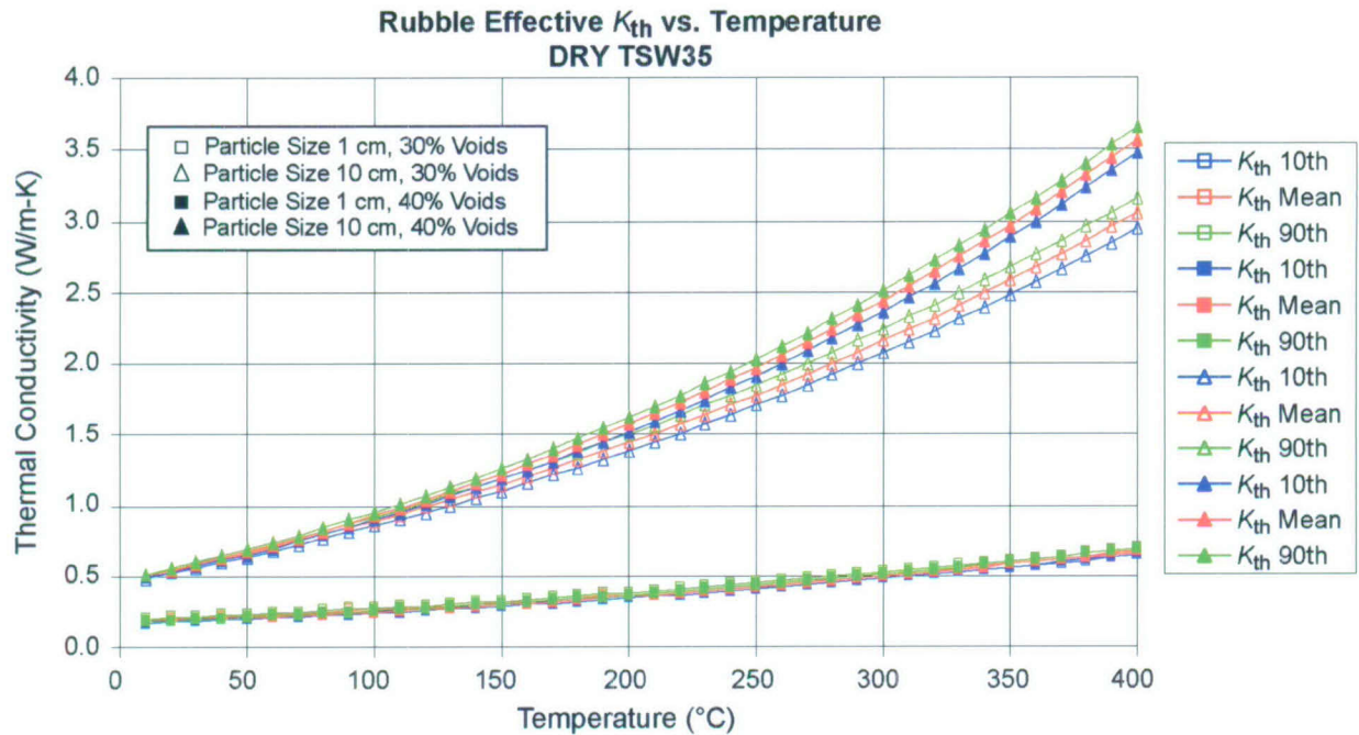
Figure XI-1[a]. Range of Effective K_{th} Calculated for Rubble with Dry Particles
