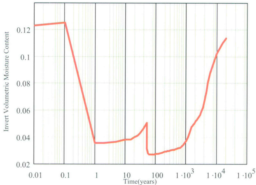
Figure XV-4. Invert Volumetric Moisture Content as a Function of Time
