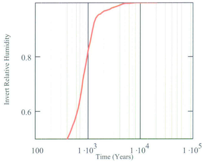
Figure XV-7. Relationship of Invert Relative Humidity over the Range from 0.50 to 1.0 After 100 Years
