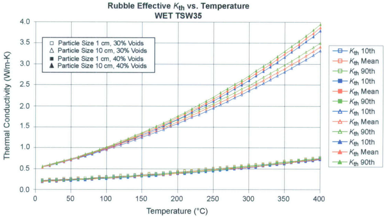
Figure XI-2[a]. Range of Effective K_{th} Calculated for Rubble with Wet Particles
