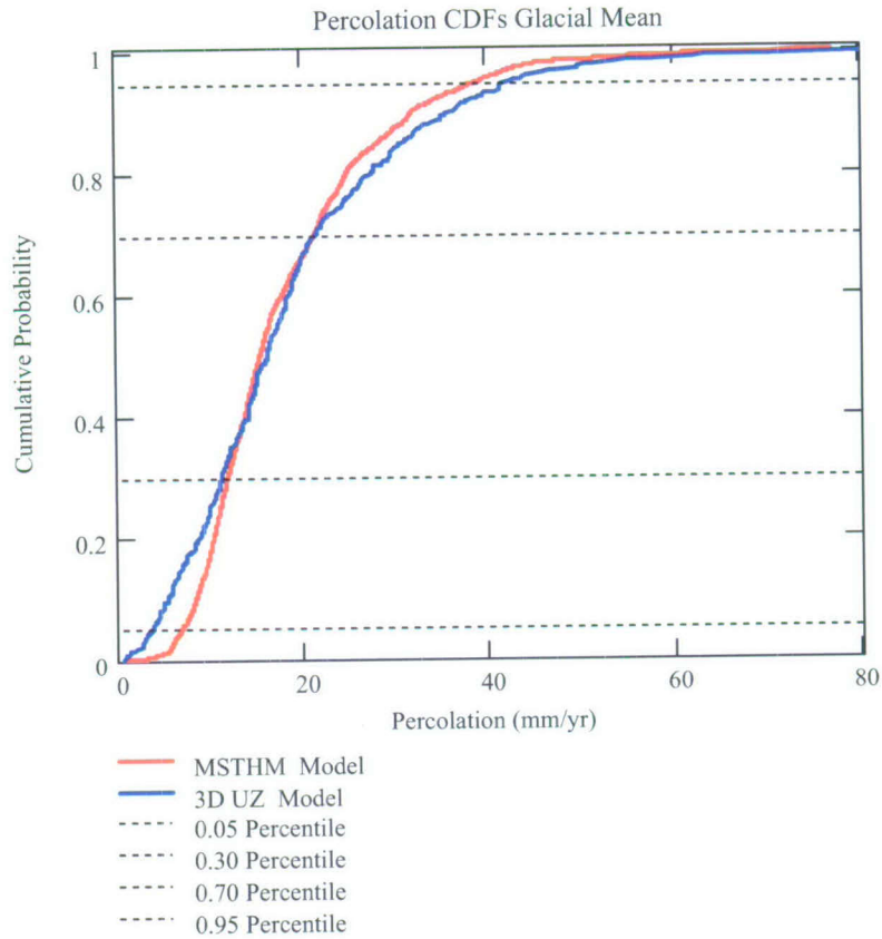
Figure XII-11. Cumulative Distribution Function Comparison for the Glacial-Climatc Mean Infiltration-Flux Case
