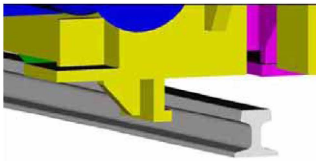
Figure 6.2-12 Conceptual Design of TEV Seismic Restraint
