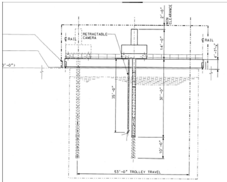
Figure 6.2-9. Spent Fuel Transfer Machine
