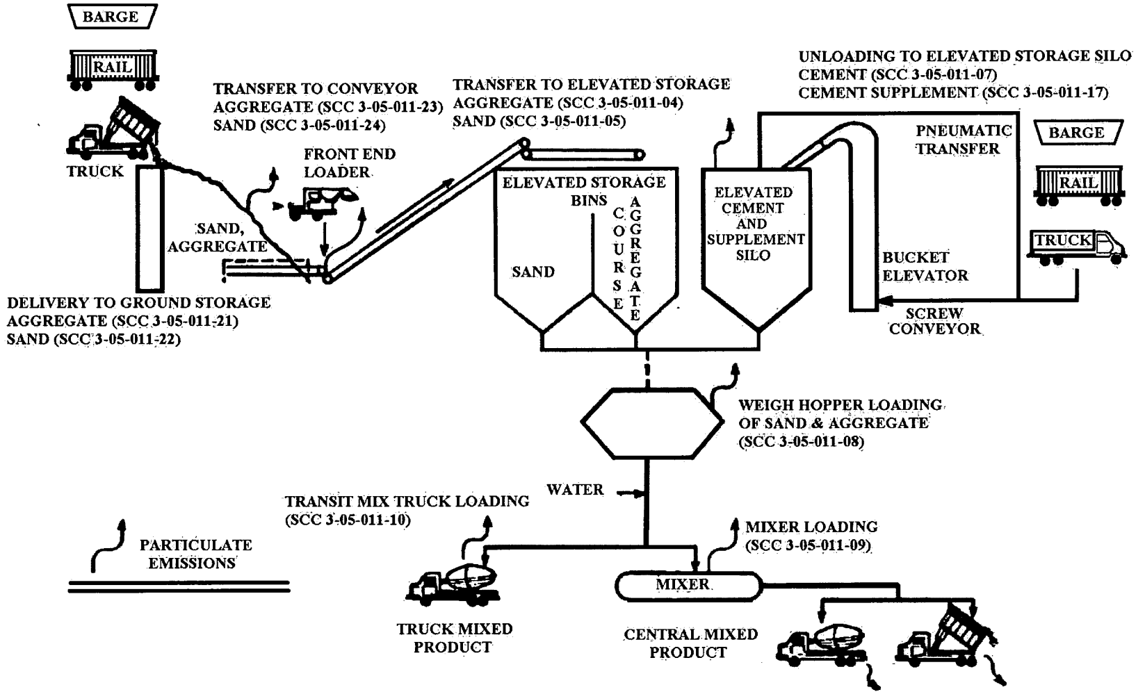
Figure 11.12-1. Typical Concrete Batching Process.
