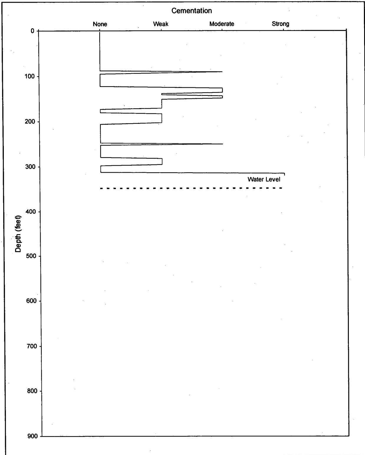
Appendix C-10 Cementation vs. Depth of Drill Cuttings in Alluvium for 29P
