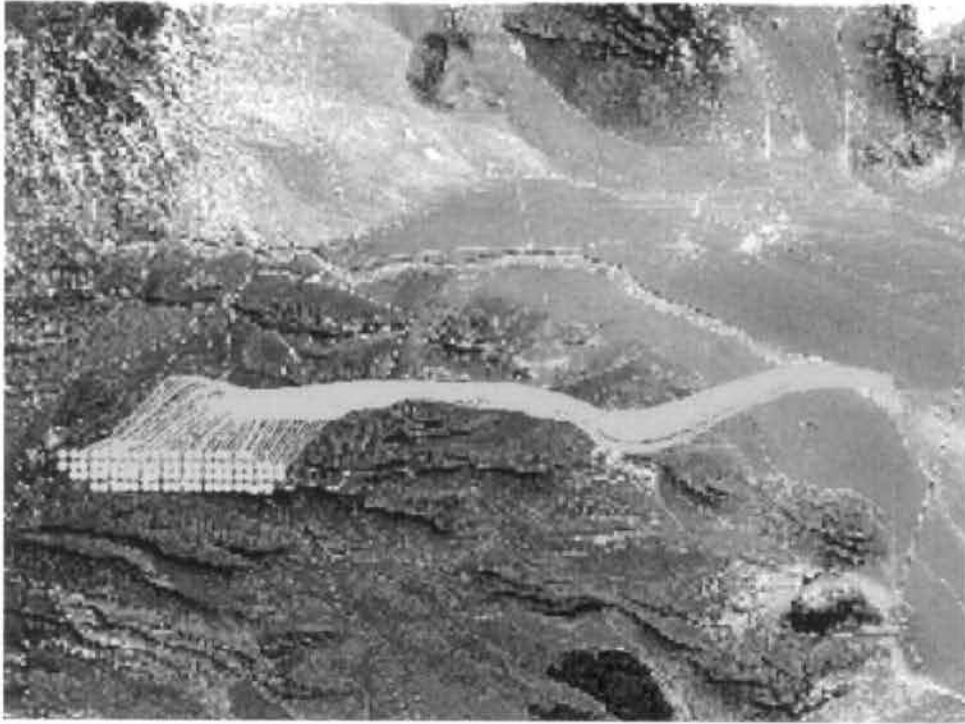
Modeled flowpaths for original model with Case 2 recharge rates
