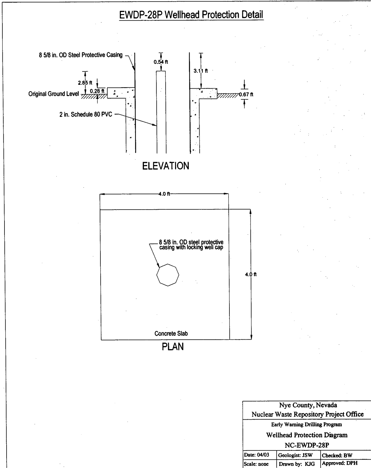
Wellhead Protection Diagram for 28P
