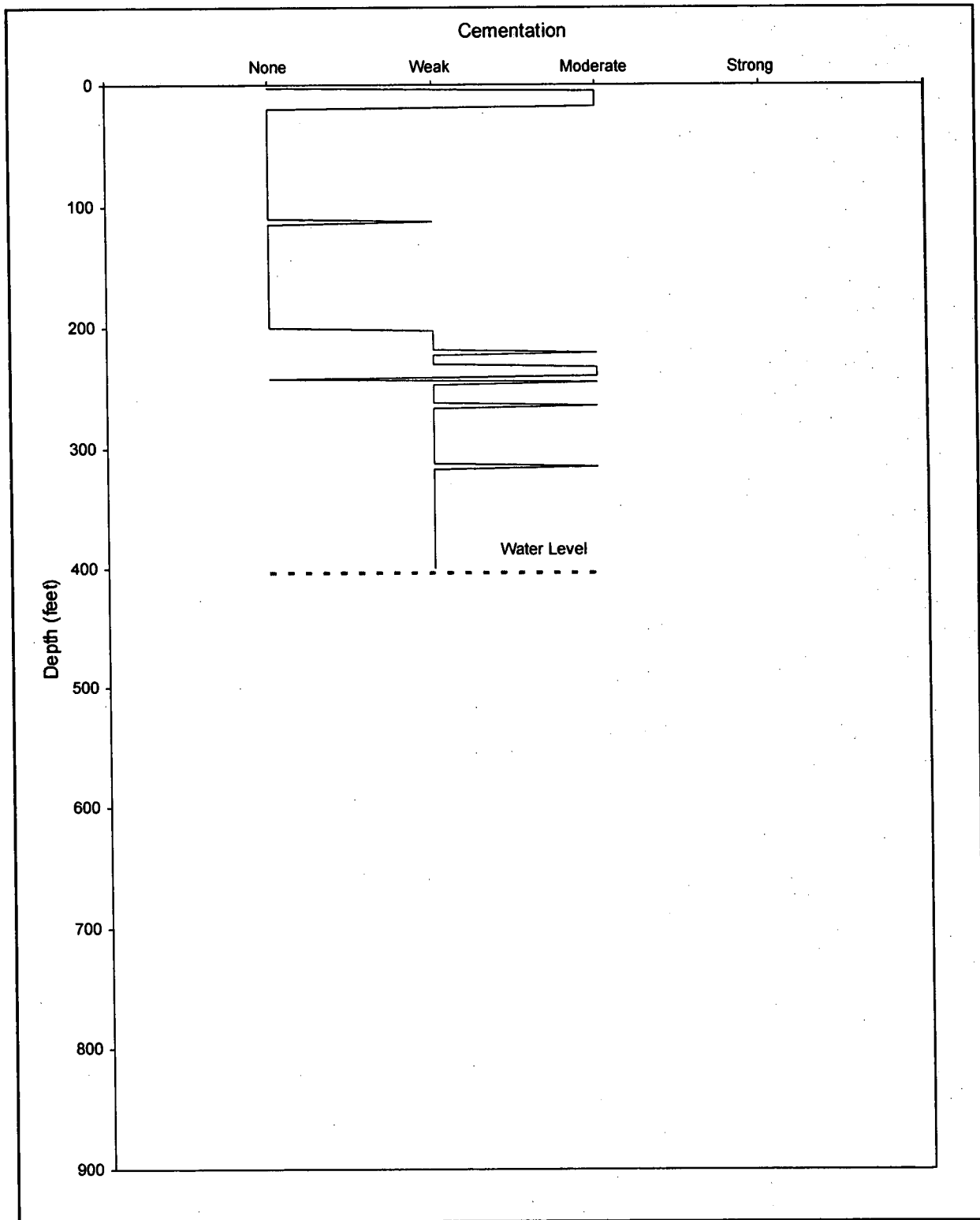
Appendix C-7 Cementation vs. Depth of Drill Cuttings in Alluvium for 24P
