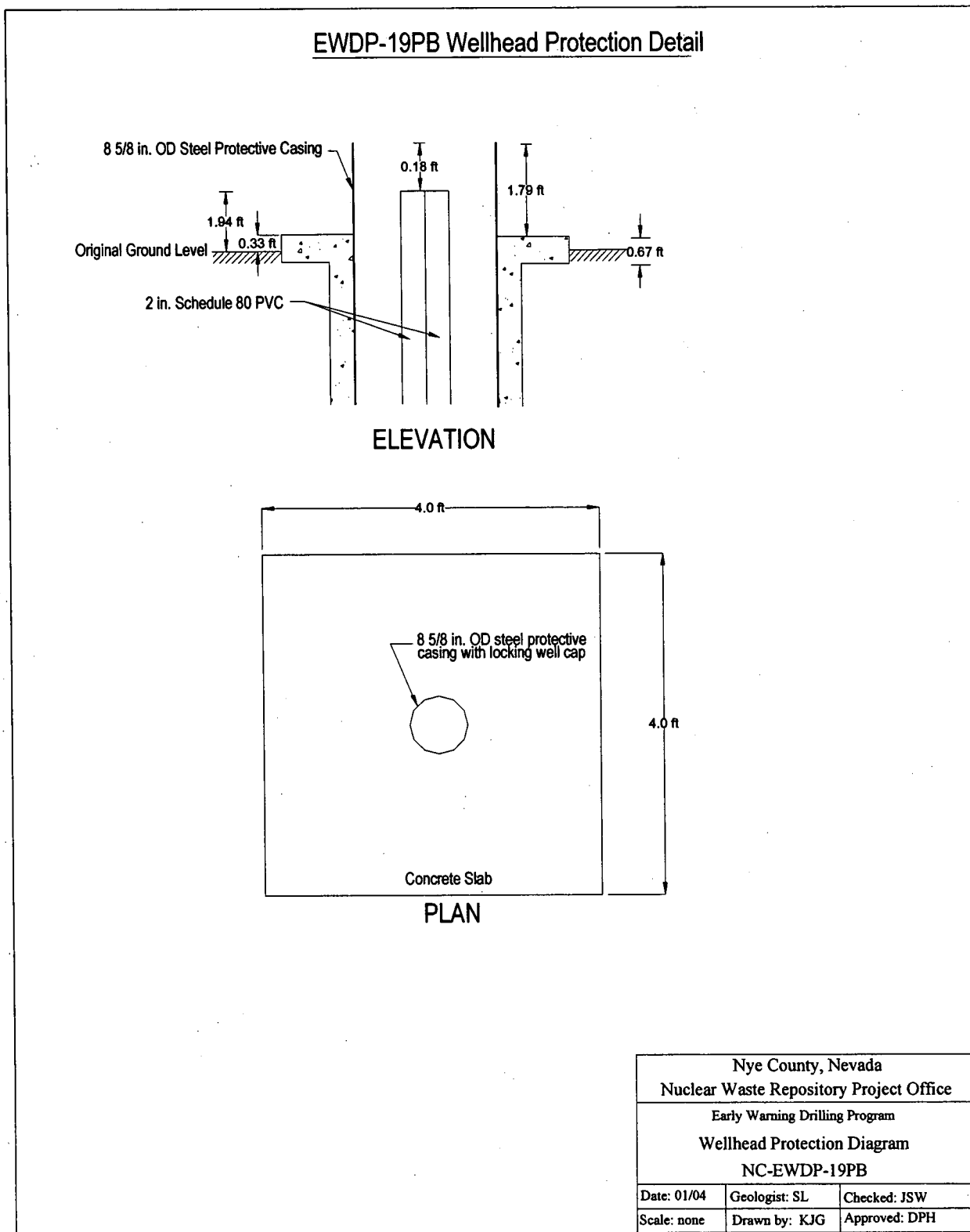
Wellhead Protection Diagram for 19PB
