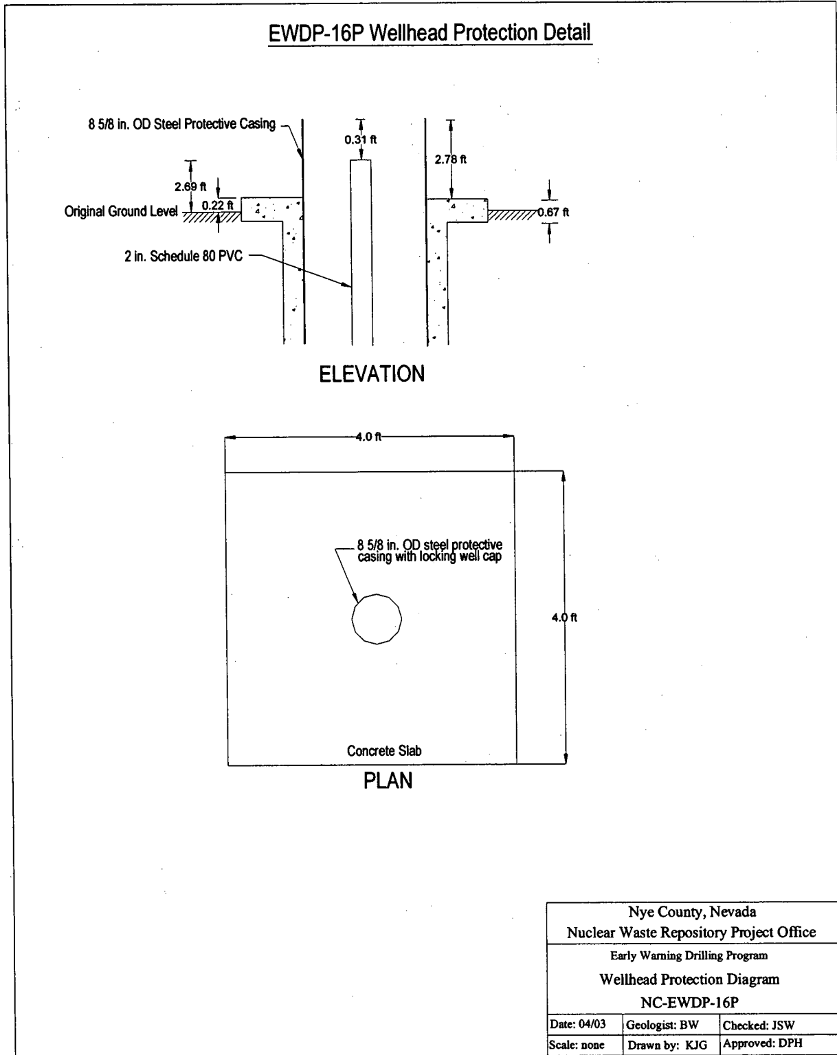
Wellhead Protection Diagram for 16P
