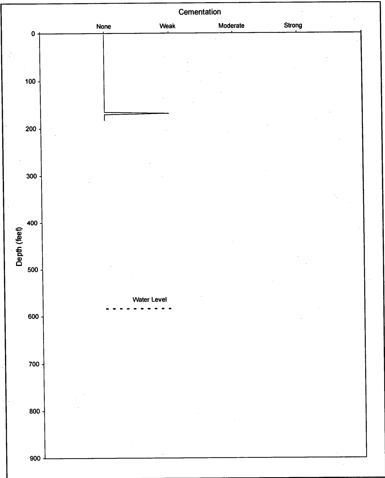
Appendix C-8 Cementation vs. Depth of Drill Cuttings in Alluvium for 27P
