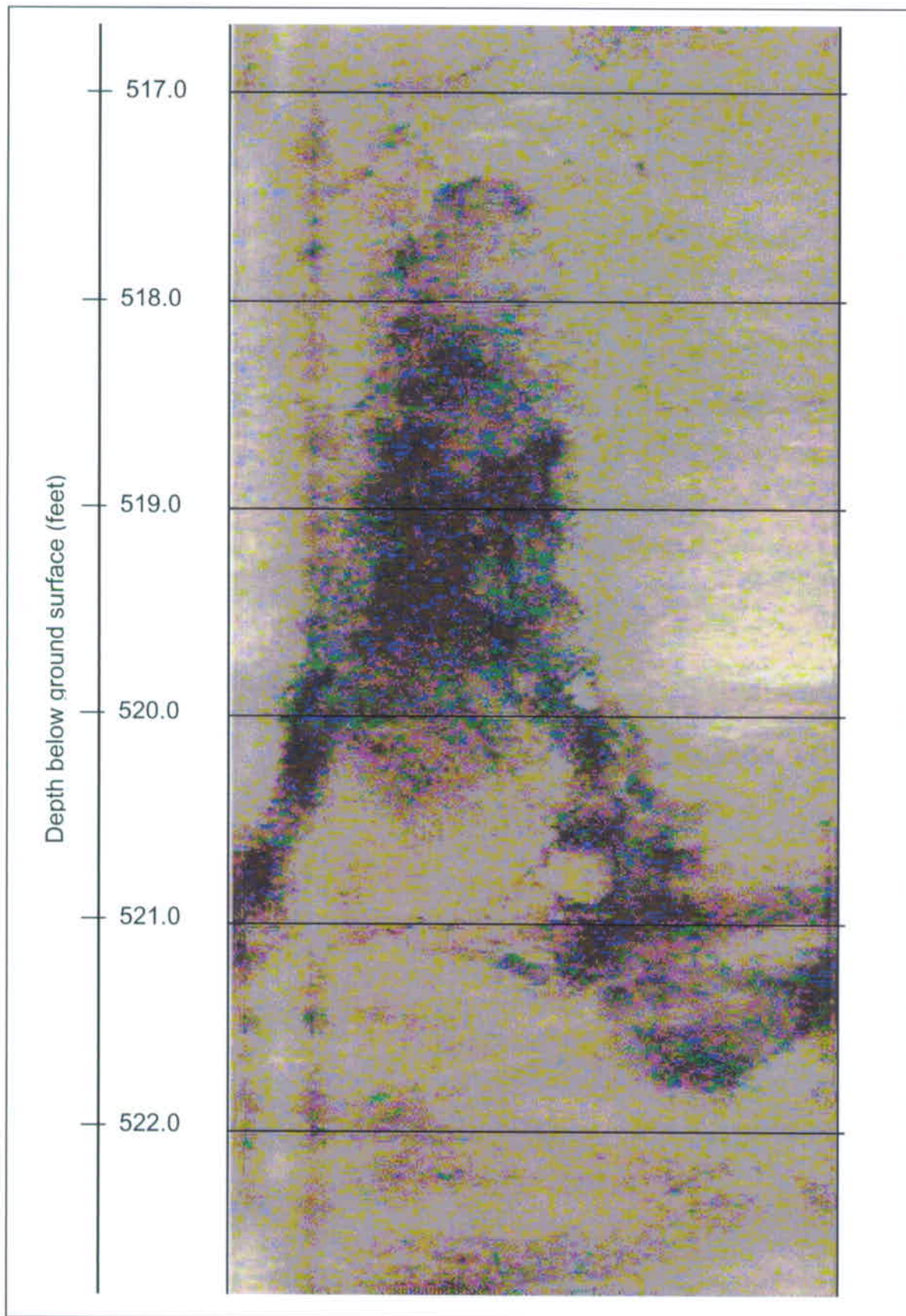
Figure 6.2-2 Optical Televiewer Image for 29P from 517 to 522 Feet Below Ground Surface
