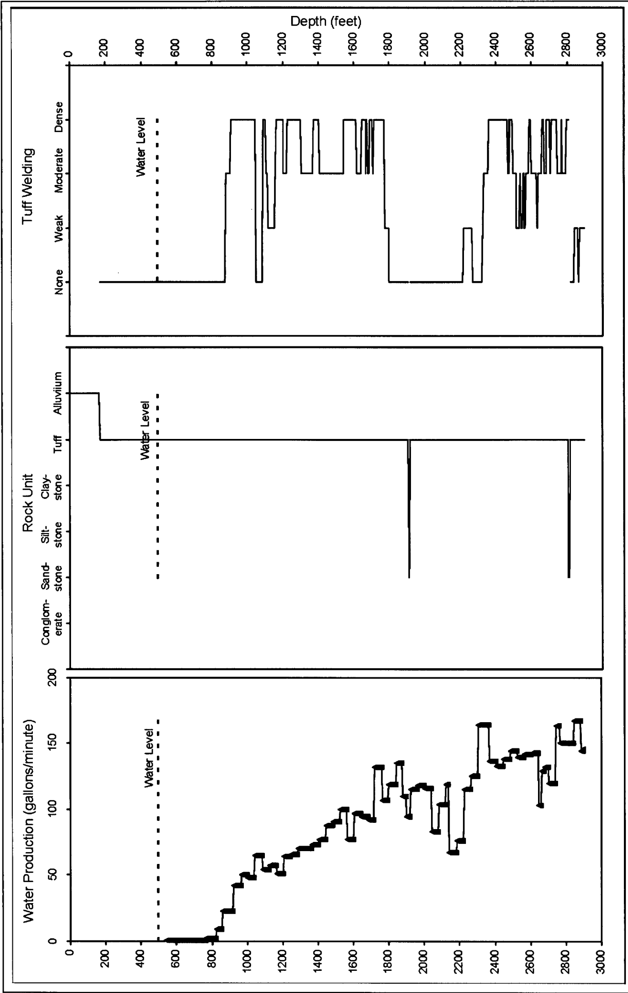
Figure 4.1-11 Water Production, Rock Unit, and Tuff Welding vs. Depth for 16P
