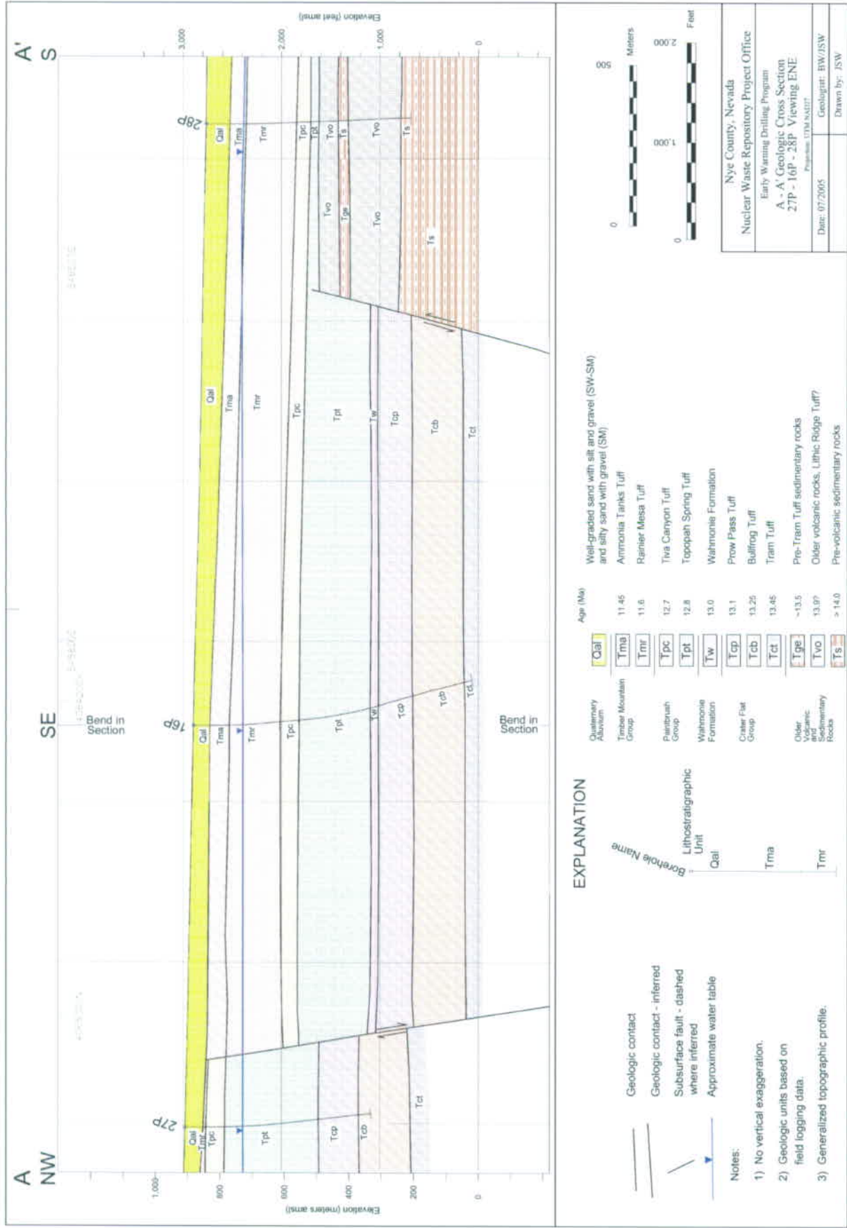
Figure 6.3-1 Cross Section A-A'
