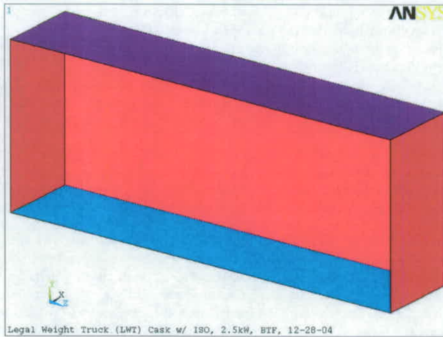
Figure 5.21. Zones for External Radiation Between ISO Container and Tunnel Surfaces
