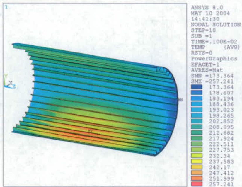
Figure F.6. Fin Structure Temperature Distribution - Normal Transport Conditions.
