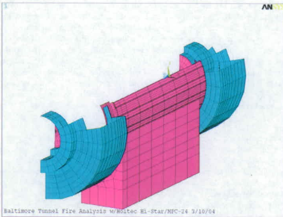
Figure 5.15. Surfaces Defined for Interaction with “Side” Gas Region
