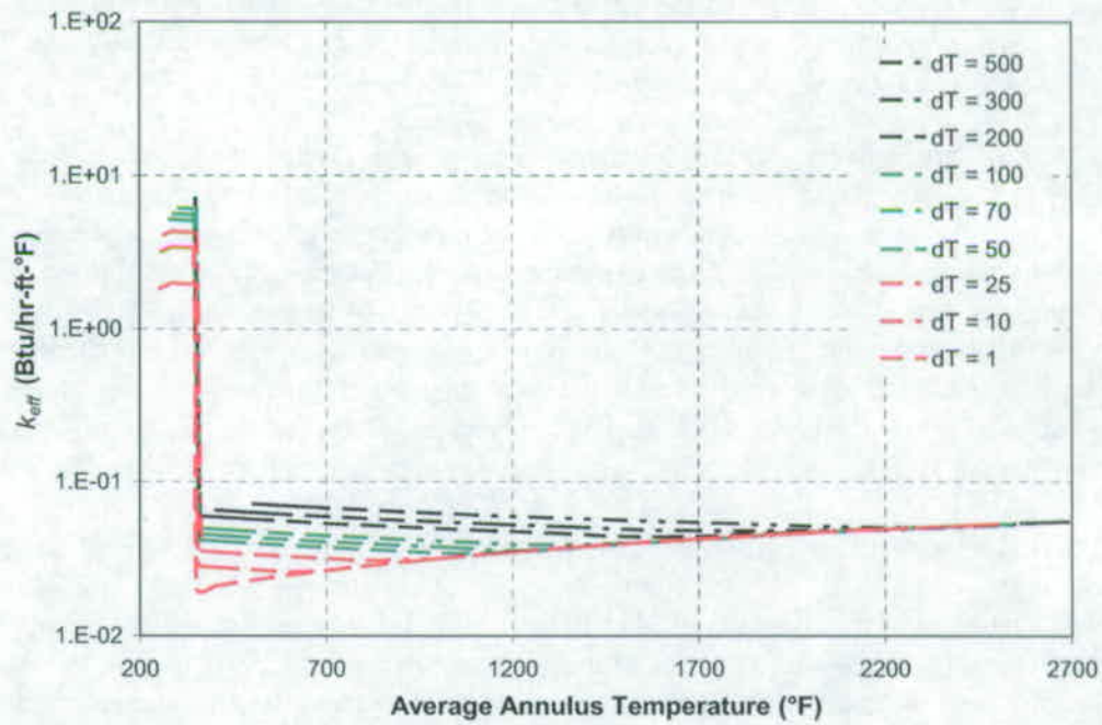
Figure 6.9. Effective Conductivity of Expansion Tank Contents
