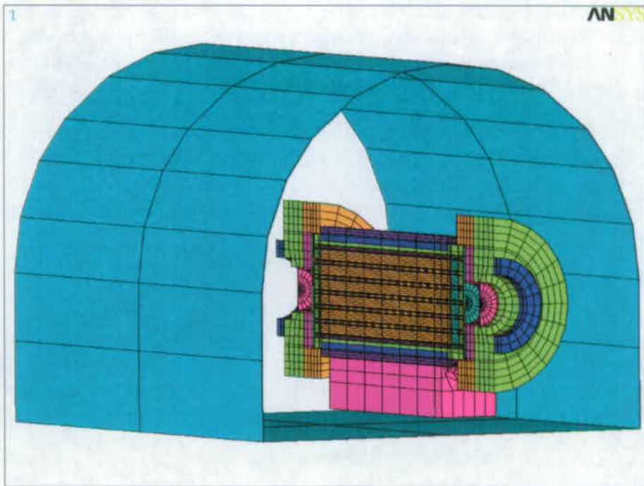
Figure 5.6. ANSYS HI-STAR 100 Package Analysis Model Element Plot
