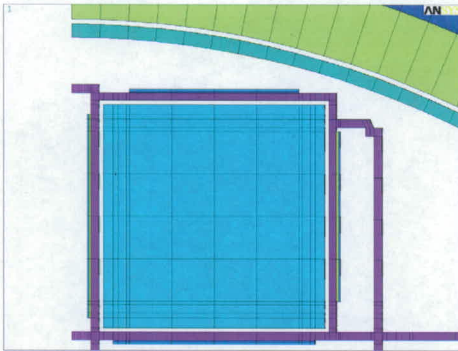
Figure 5.10. Close-up of Canister Basket and Fuel Compartment (without helium elements)
