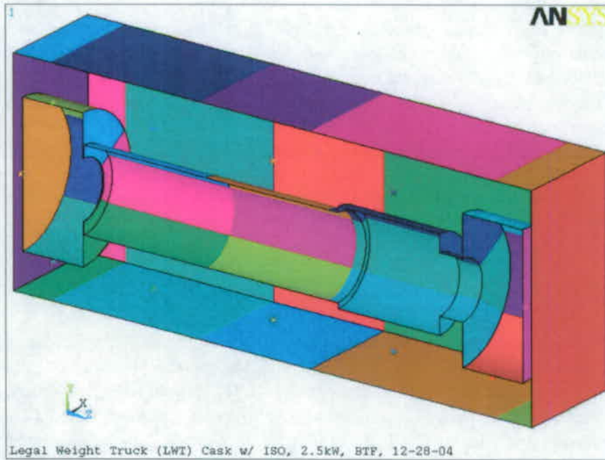
Figure 5.20. Zones for Convection Heat Transfer Within the ISO Container
