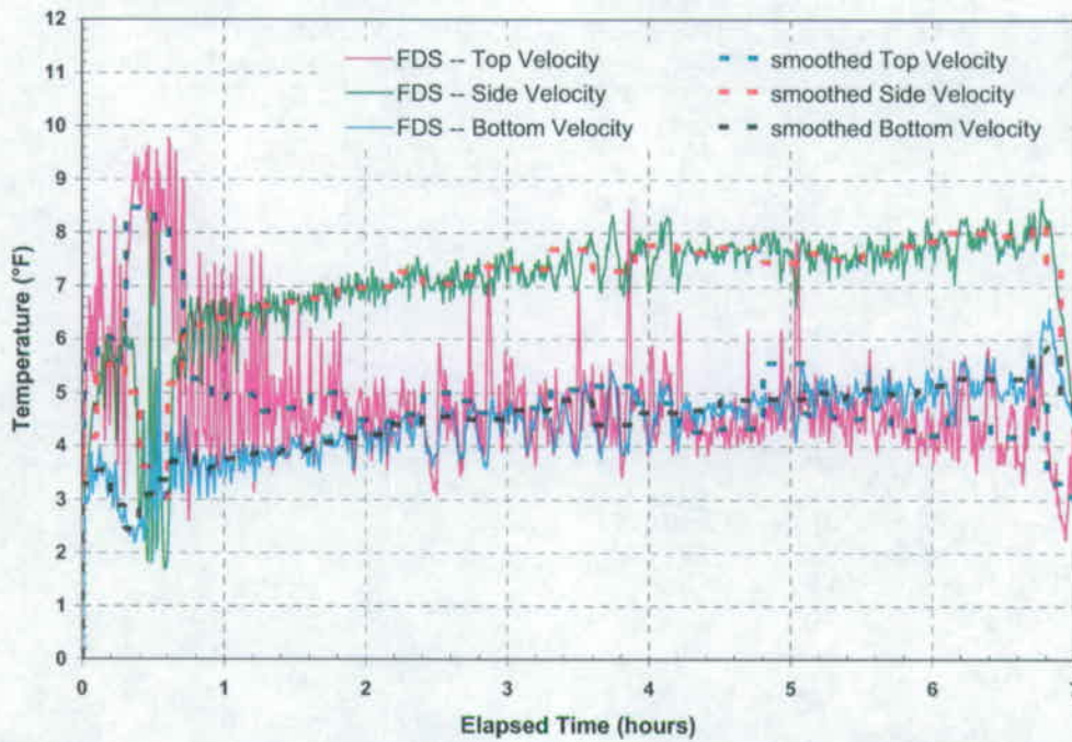
Figure D.5. Velocities at Peak Air Temperature Locations Calculated with FDS for Top, Side, and Bottom Regions at 20 meters from Fire Location during 7-hr Fire
