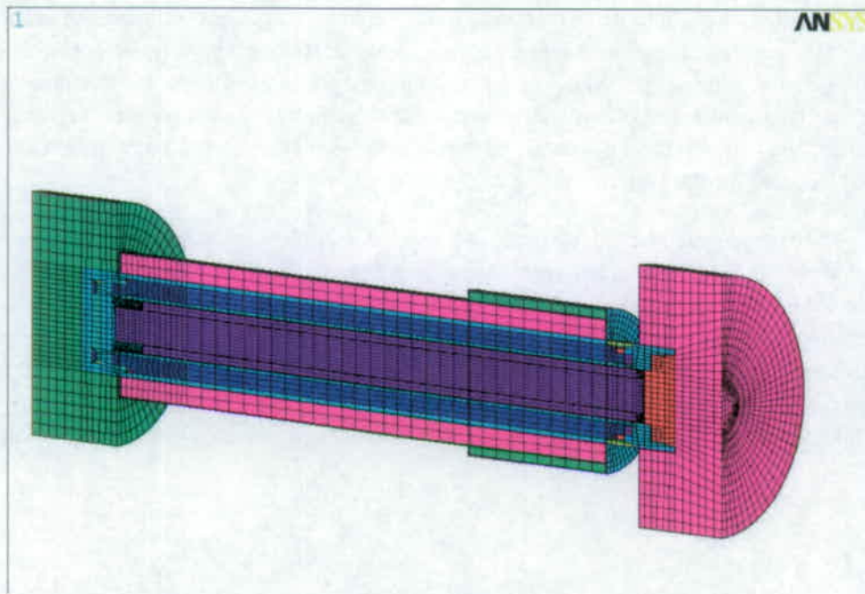
Figure 5.4. NAC LWT Package Geometry Model
