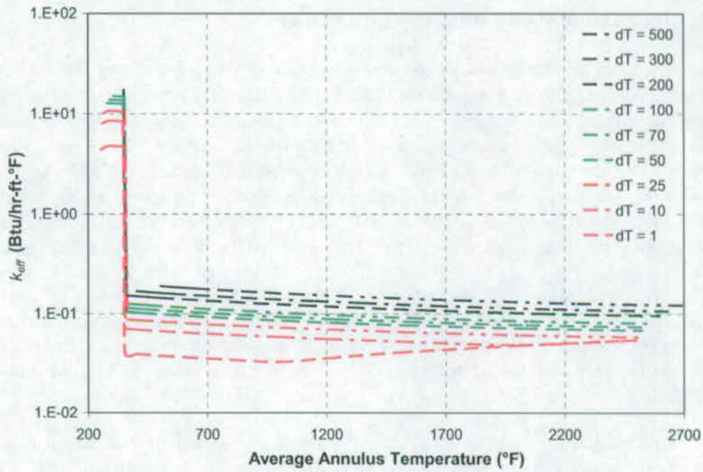
Figure 6.7. Effective Conductivity of Liquid Neutron Shield Tank
