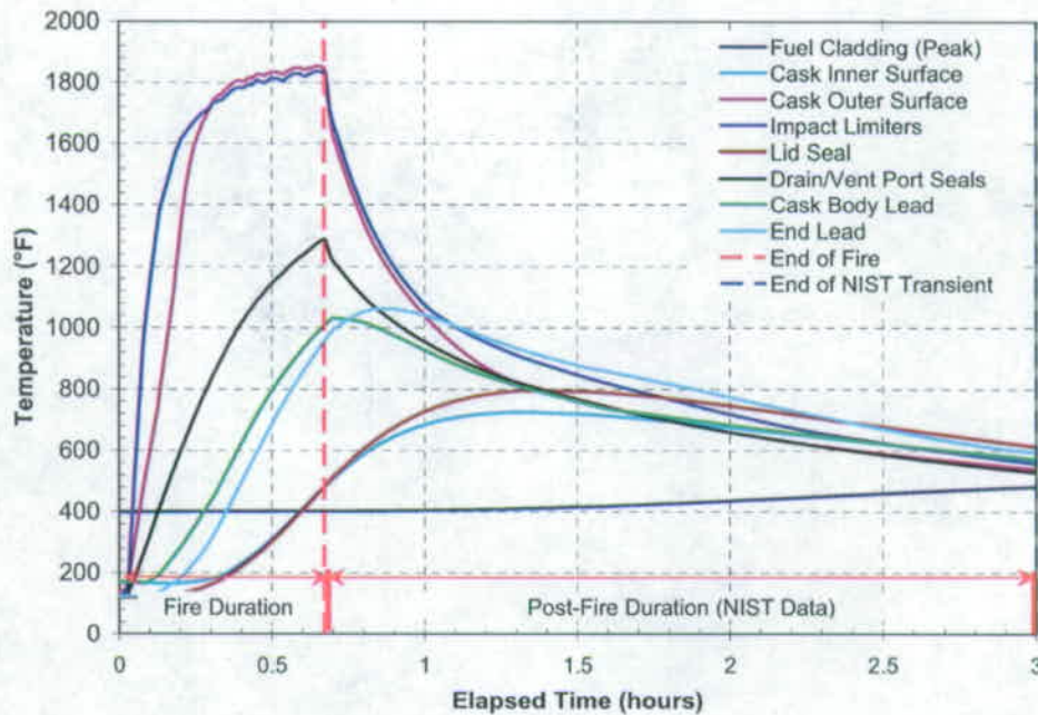
Figure 7.5. NAC LWT Package (without ISO Container): Maximum Temperature Histories for First 3 hours of Fire Transient
