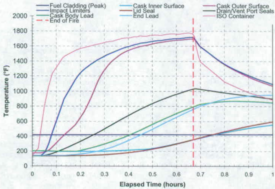
Figure 7.1. NAC LWT Package (with ISO Container): Component Maximum Temperature Histories During Fire Transient
