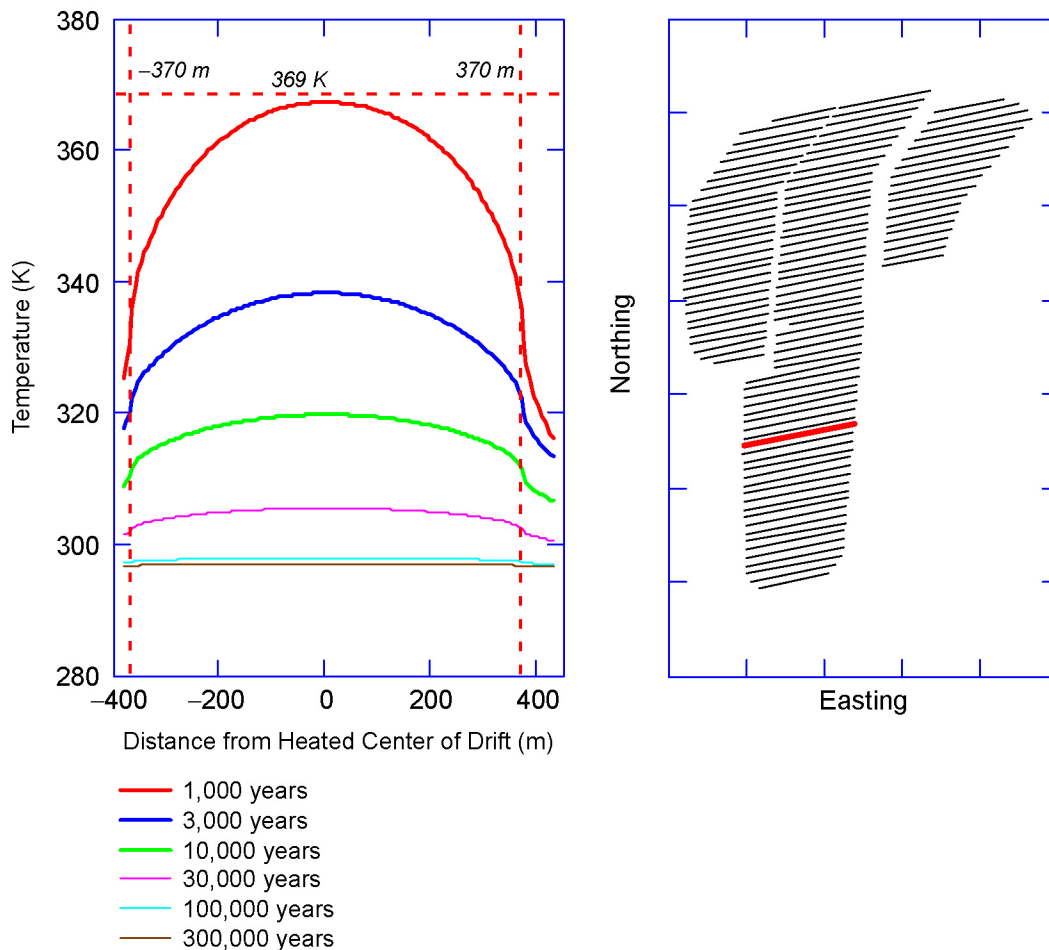
Figure 6-4[a]. Drift Wall Temperatures (Chosen Drift #7)
