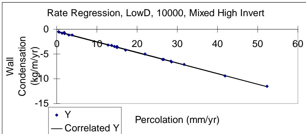
Figure H.2-5. Wall Rate Regression, Low D, 10,000 Years, Mixed High Invert Transport
