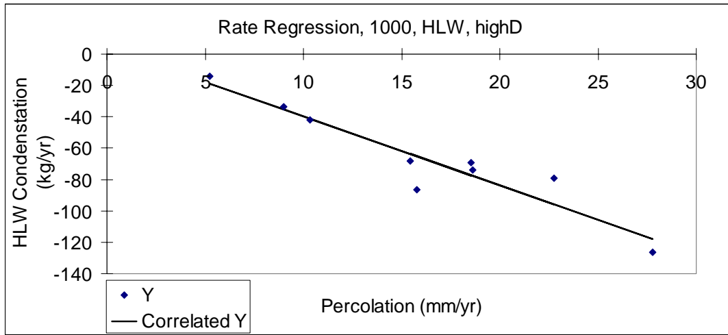
Figure I.2-9. HLW Rate Regression, High D, 1,000Years, Unmixed High Invert Transport
