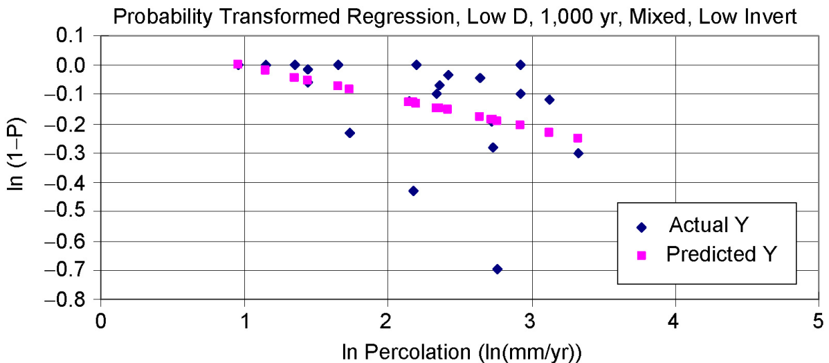
Figure 6-11[a]. Current Probability Regression Analysis (ventilated drip shield (mixed), low invert transport, low dispersivity, 1,000 years)
