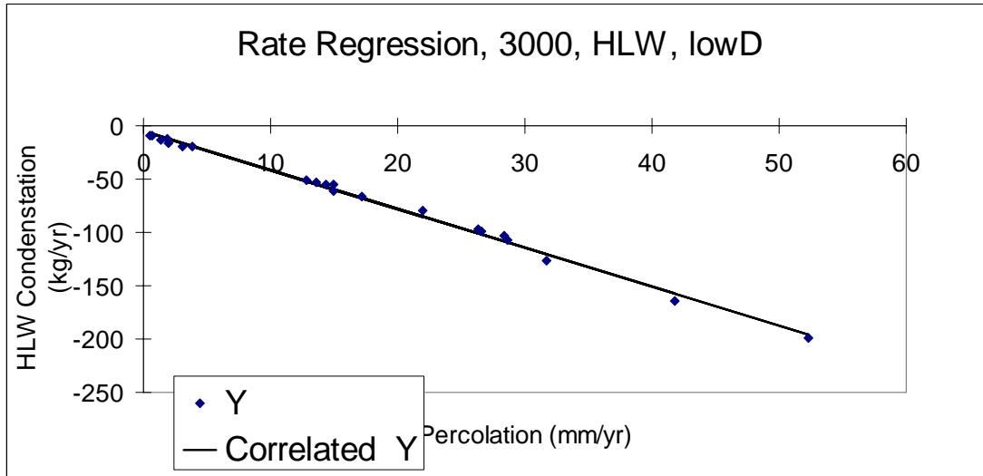
Figure I.2-5. HLW Rate Regression, Low D, 3,000 Years, Unmixed High Invert Transport
