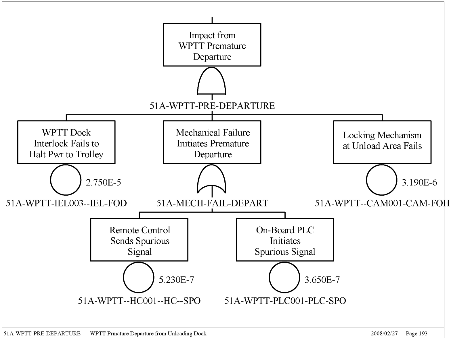
Figure B5.4-20. Fault Tree for Malfunction of WPTT or Waste Package Transfer Carriage (Continued)
