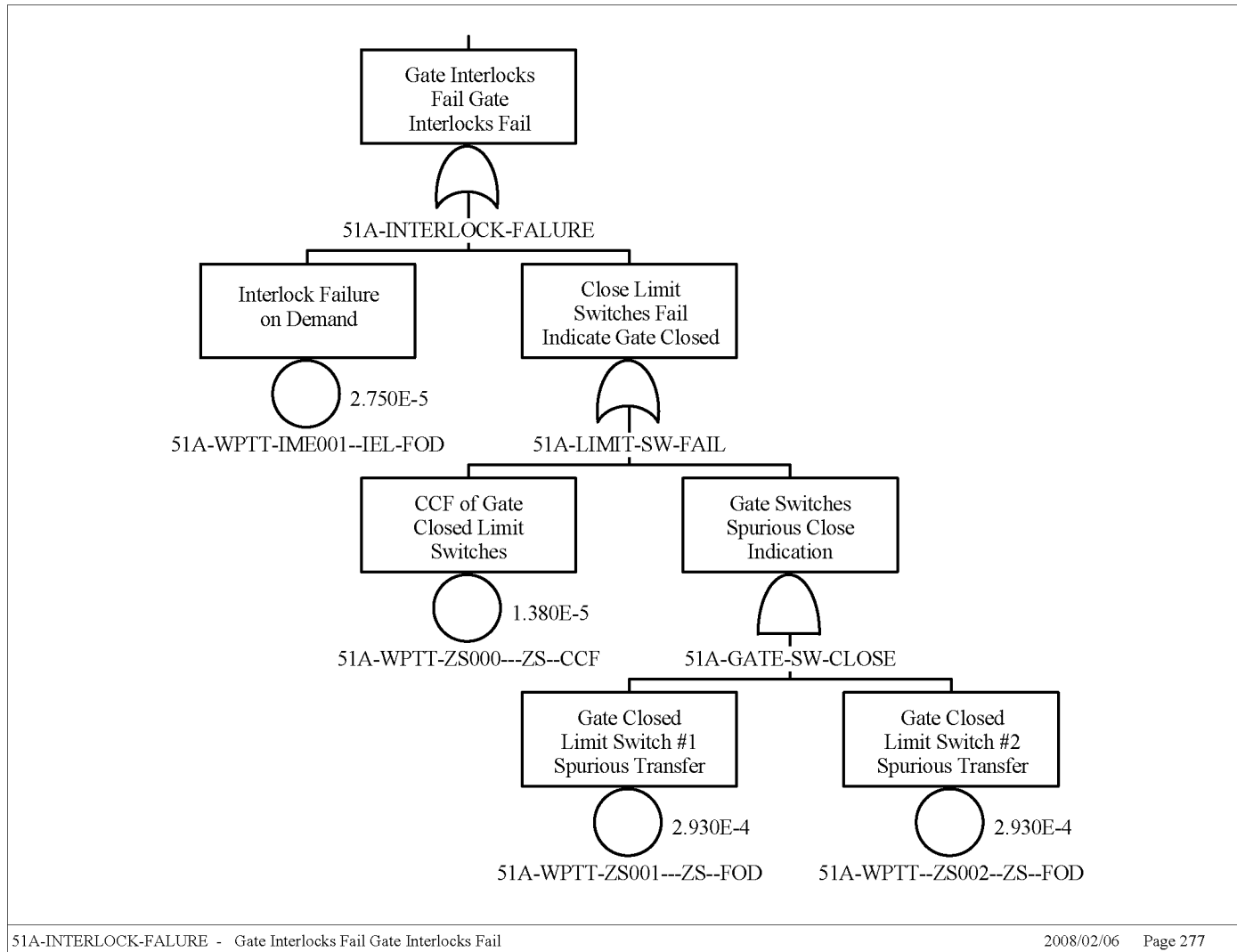
Figure B5.4-6. Fault Tree for Spurious Movement of the WPTT in the Loading Area While Loading the Waste Package with Canisters (Continued)
