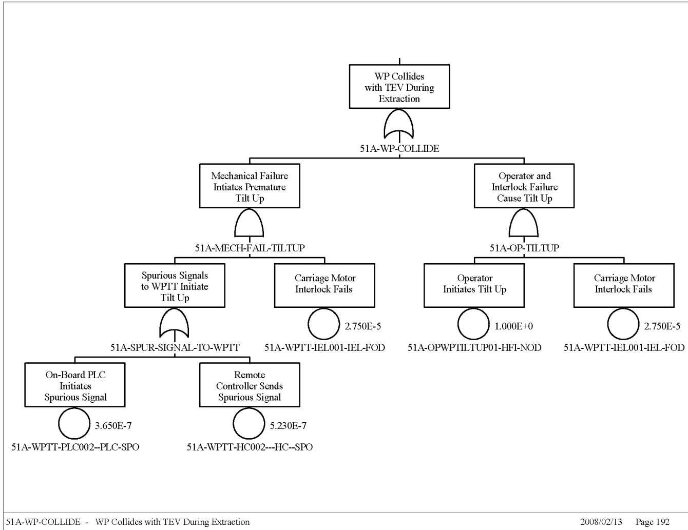
Figure B5.4-21. Fault Tree for Malfunction of WPTT or Waste Package Transfer Carriage (Continued)
