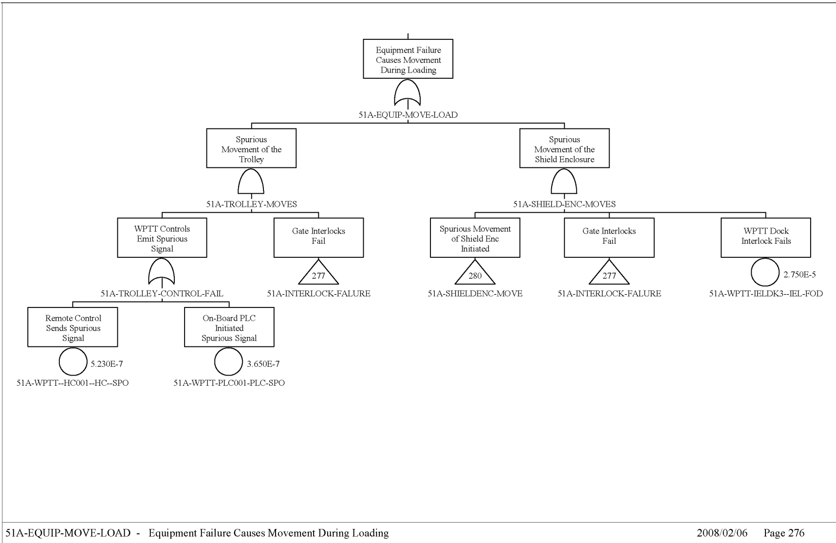
Figure B5.4-4. Fault Tree for Spurious Movement of the WPTT in the Loading Area While Loading the Waste Package with Canisters (Continued)
