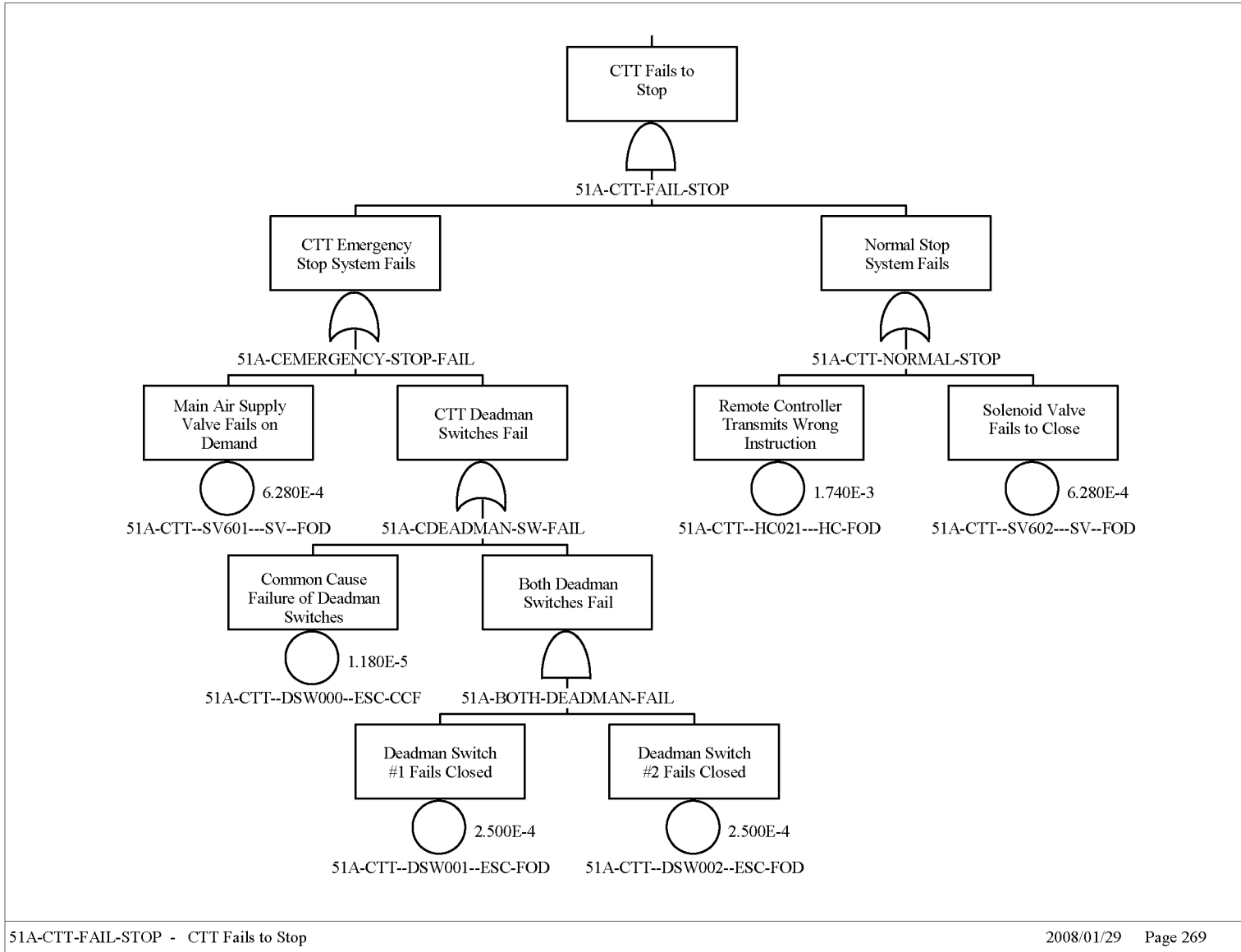
Figure B2.4-11. Fault Tree for Collision of the CTT During Cask Transfer (Page 2)
