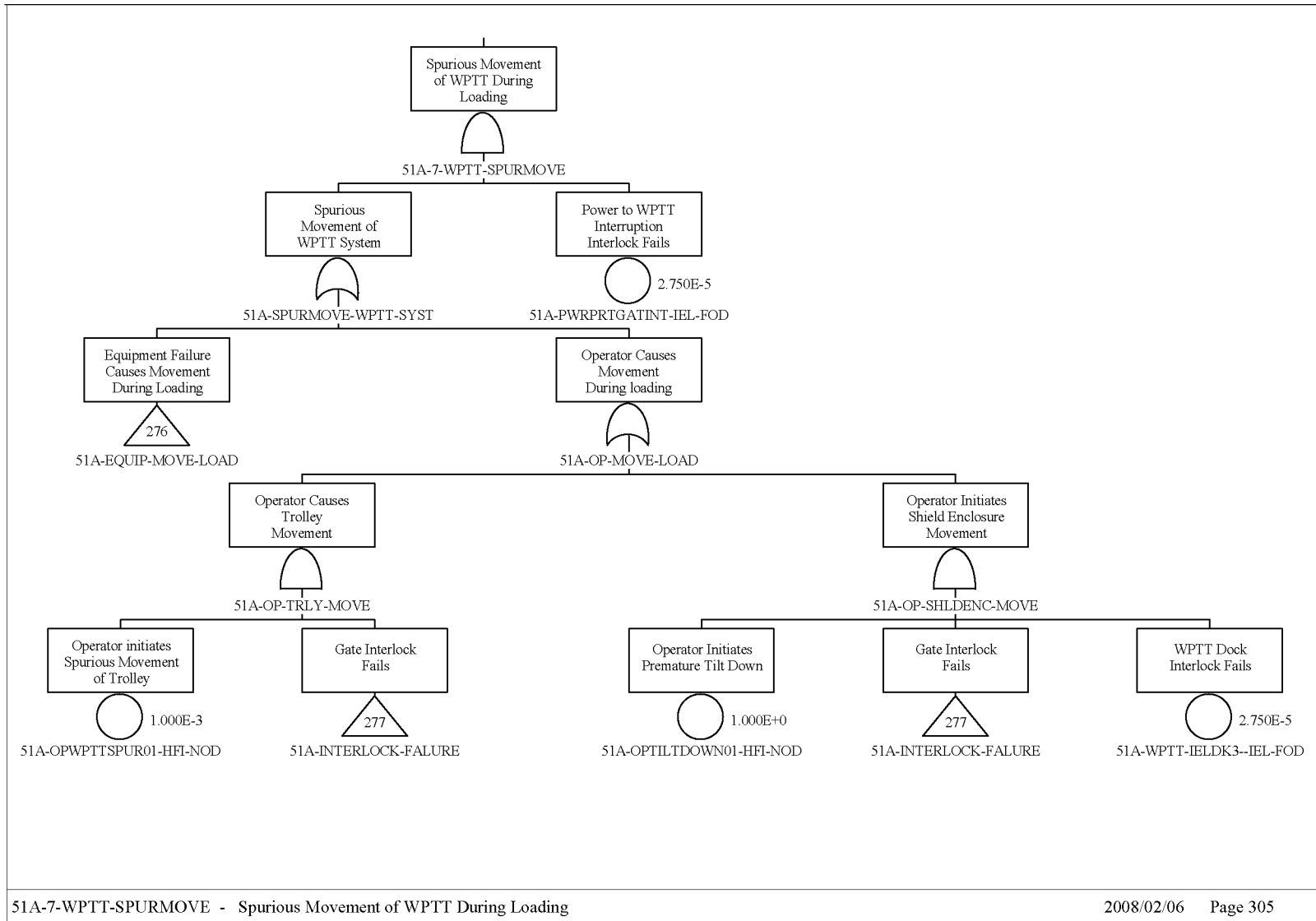
Figure B5.4-3. Fault Tree for Spurious Movement of the WPTT in the Loading Area While Loading the Waste Package with Canisters
