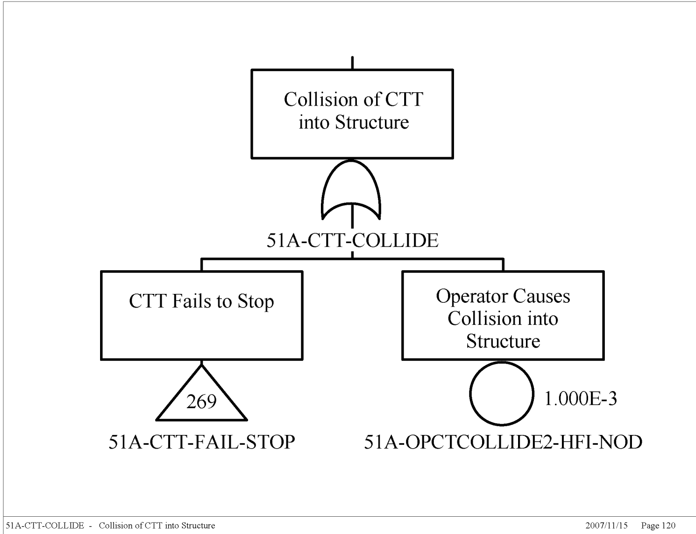
Figure B2.4-10. Fault Tree for Collision of the CTT During Cask Transfer (Page 1)
