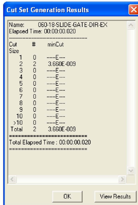
Figure B3.4-4. Uncertainty Results for the Inadvertent Opening of Slide Gate Causing Direct Exposure Fault Tree
