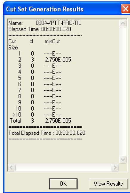
Figure B5.4-15. Cut Set Generation Results for the for Premature Tilt-down of the WPTT Fault Tree
