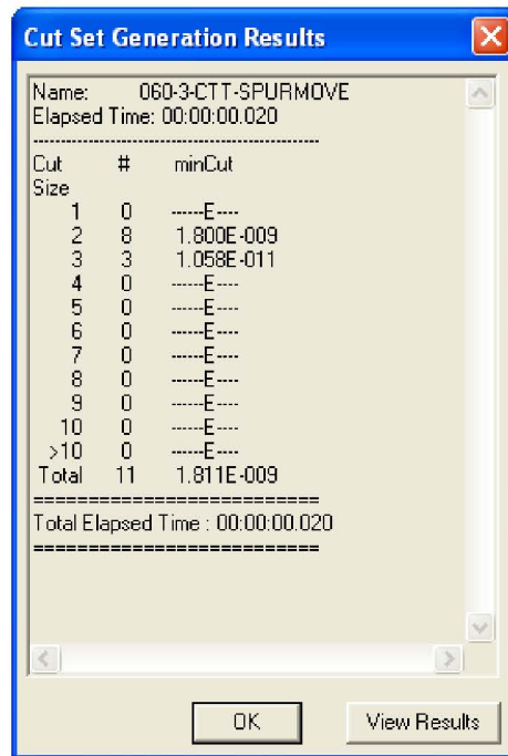
Figure B2.4-2. Cut Set Generation Results for “Spurious Movement of the CTT in the Cask Preparation Area during Cask Loading”
