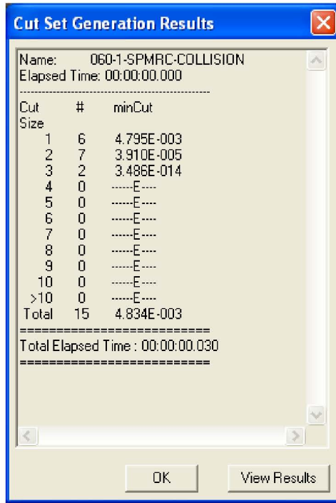
Figure B1.4-2. Cut Set Generation Results for the SPMRC Collides with CRCF Structures Fault Tree
