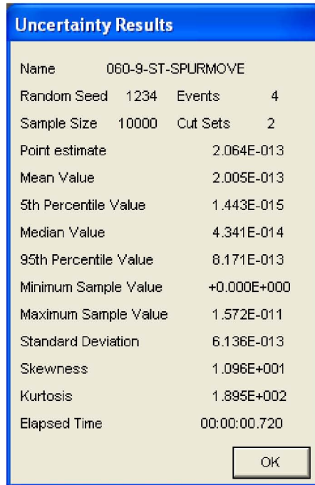
Figure B6.4-23. Uncertainty Results Site Transporter Spurious Movement Fault Tree
