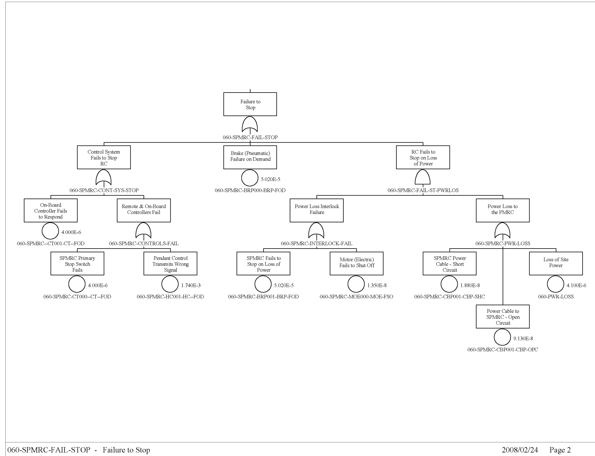
Figure B1.4-4. SPMRC Fail to Stop
