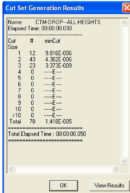
Figure B4.4-1. Uncertainty Results of the “Canister Drop from Below the Canister Design-Limit Drop Height” Fault Tree
