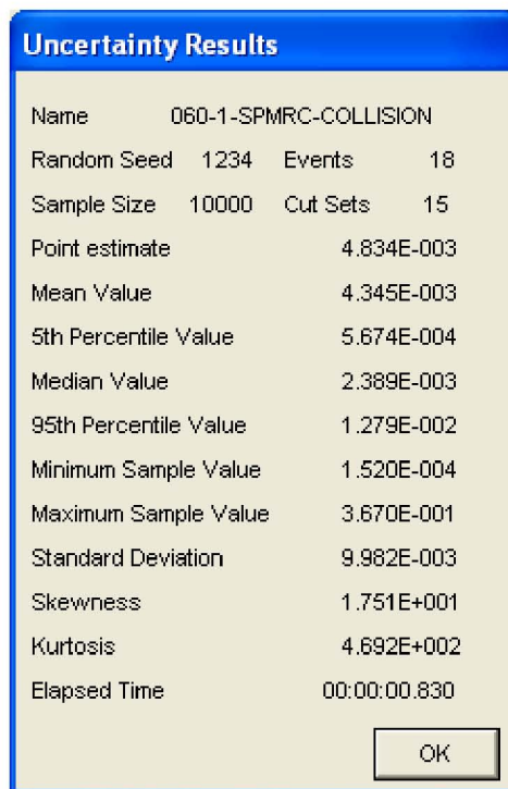
Figure B1.4-1. Uncertainty Results of the SPMRC Collides with CRCF Structures Fault Tree
