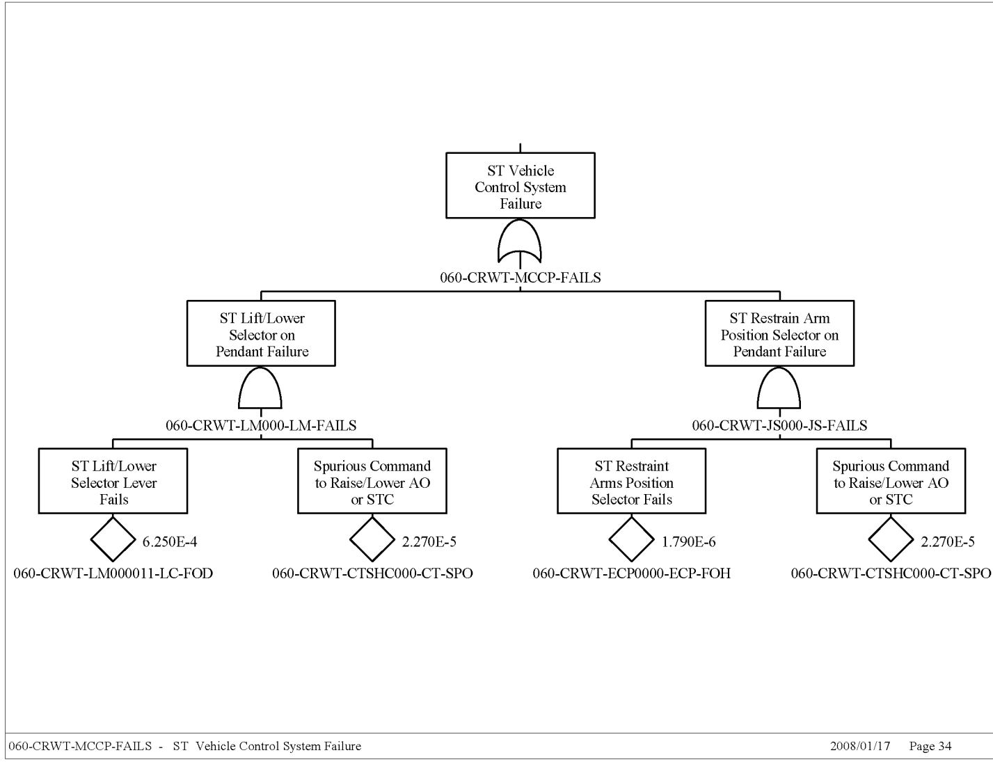
Figure B6.4-14. Site Transporter Vehicle Control System Failure
