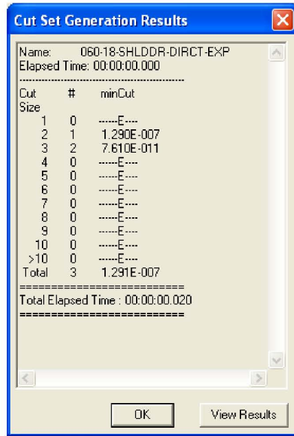
Figure B3.4-2. Cut Set Generation Results for Inadvertent Opening of the Shield Door
