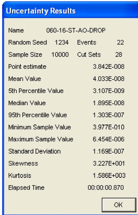
Figure B6.4-6. Uncertainty Results for Site Transporter Load Drop during Lift and Movement Fault Tree
