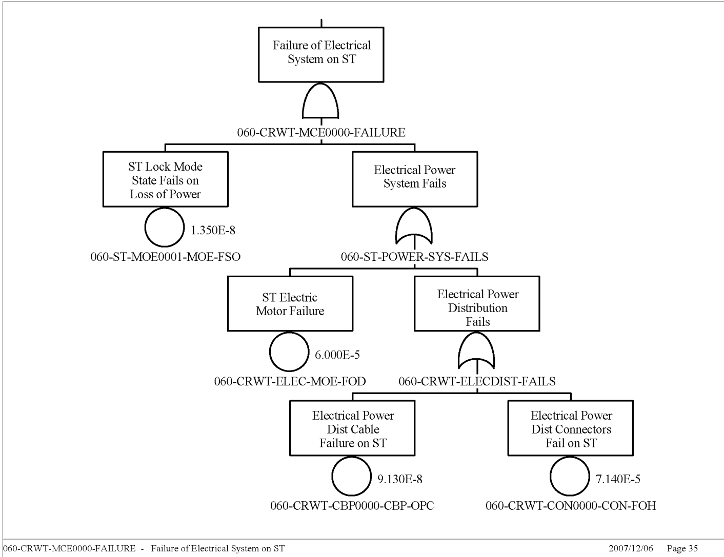
Figure B6.4-15. Failure of Electrical System on Site Transporter
