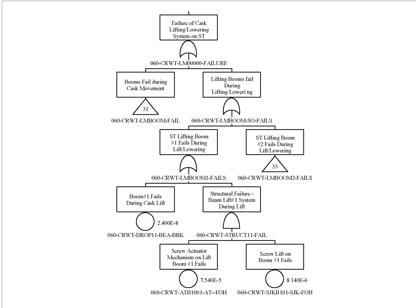
060-CRWT-LM00000-FAILURE - Failure of Cask Lifting/Lowering System on ST
