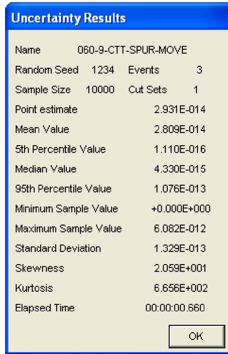
Figure B2.4-12. Uncertainty Results for the Spurious Movement of the CTT in the Canister Transfer Room Fault Tree
