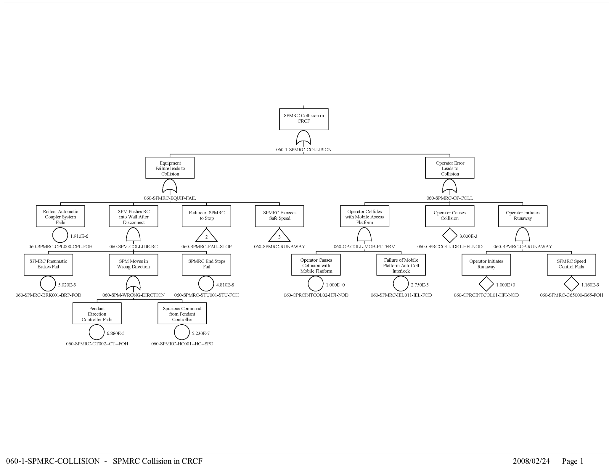
Figure B1.4-3. SPMRC Collision in CRCF
