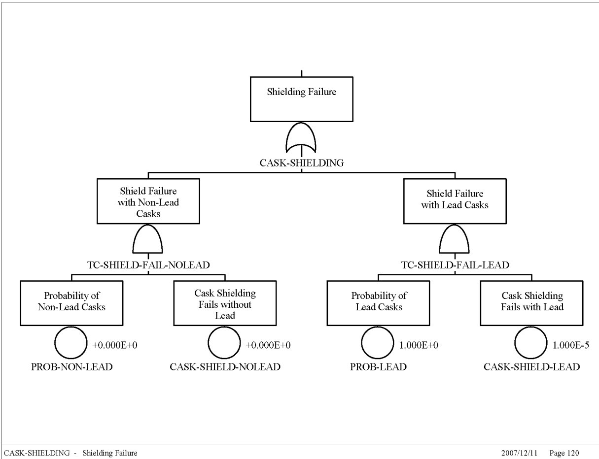
Figure B9.7-3. Cask Shielding Failure
