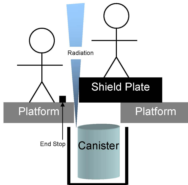
Figure E6.3-2. 060-OpDPCShield1-HFI-NOW Operator Failure Scenario
