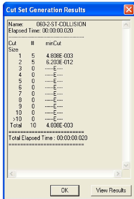
Figure B6.4-1. Uncertainty Results for Site Transporter Collides with CRCF Structures Fault Tree
