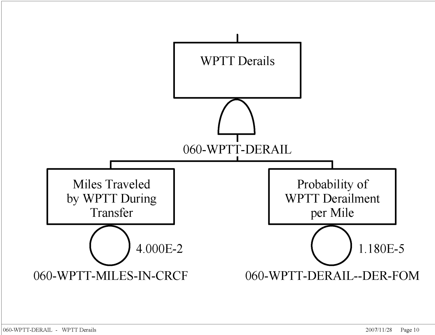
Figure B5.4-13. Fault Tree for Derailment of the WPTT during WP Transfer
