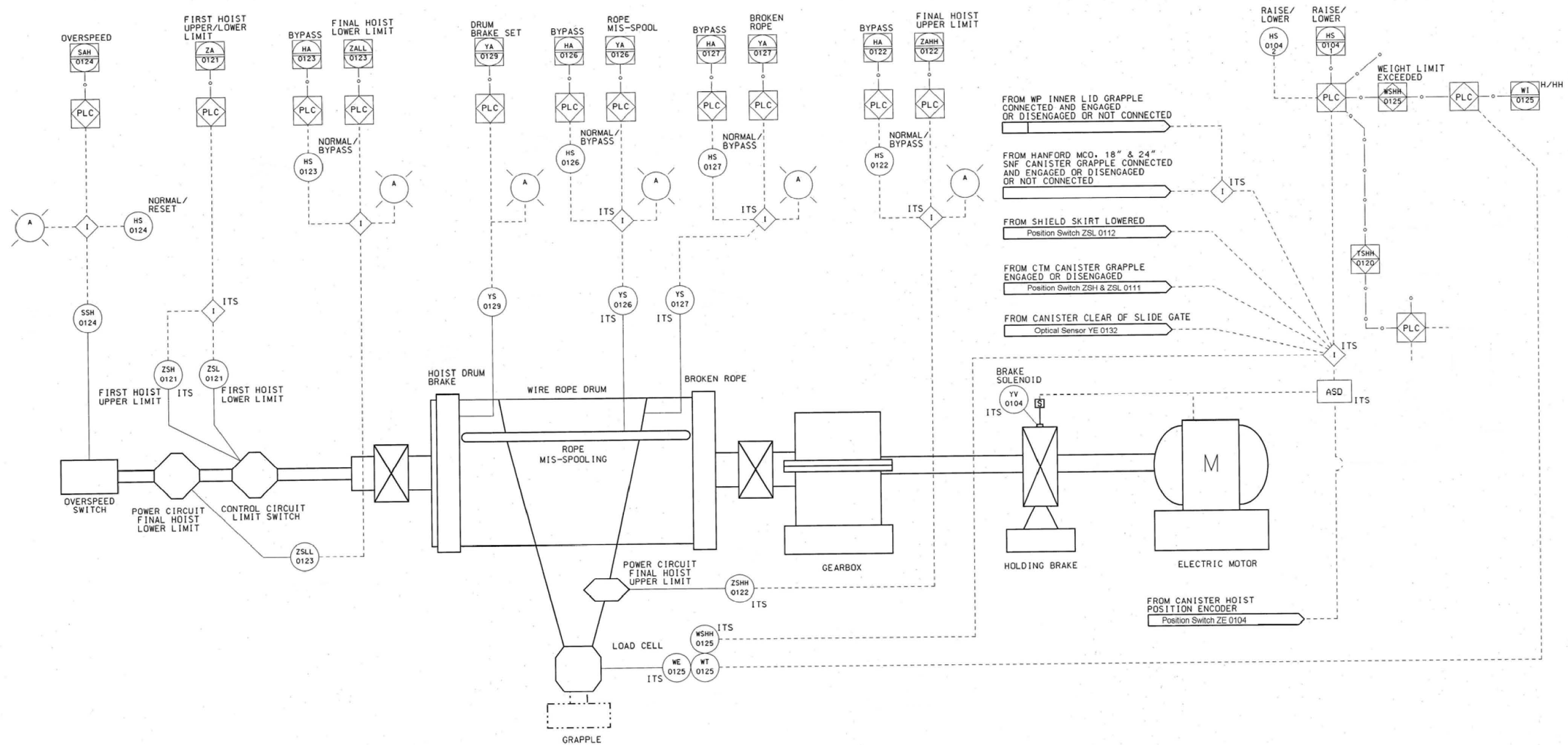
Figure B4.2-3. Canister Hoist Instrumentation
