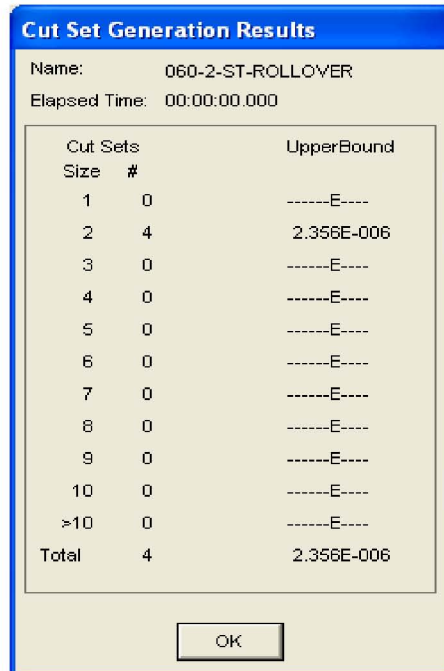
Figure B6.4-20. Uncertainty Results for the Site Transporter Rollover (Tipover) Fault Tree
