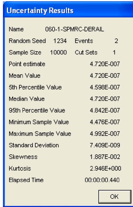
Figure B1.4-11. Uncertainty Results of the SPMRC Derailment Fault Tree
