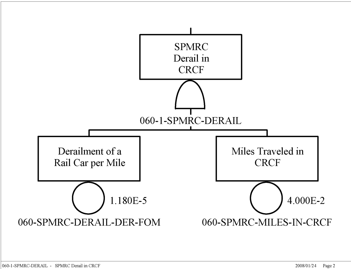
Figure B1.4-13. SPMRC Derailment in CRCF
