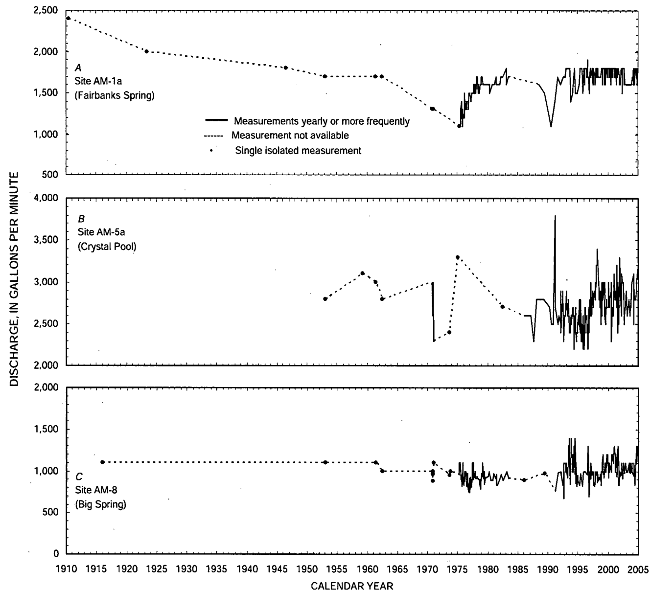
Figure 7. Discharge at sites (A) AM-1a (Fairbanks Spring), (B) AM-5a (Crystal Pool), and (C) AM-8 (Big Spring), 1910–2004.
