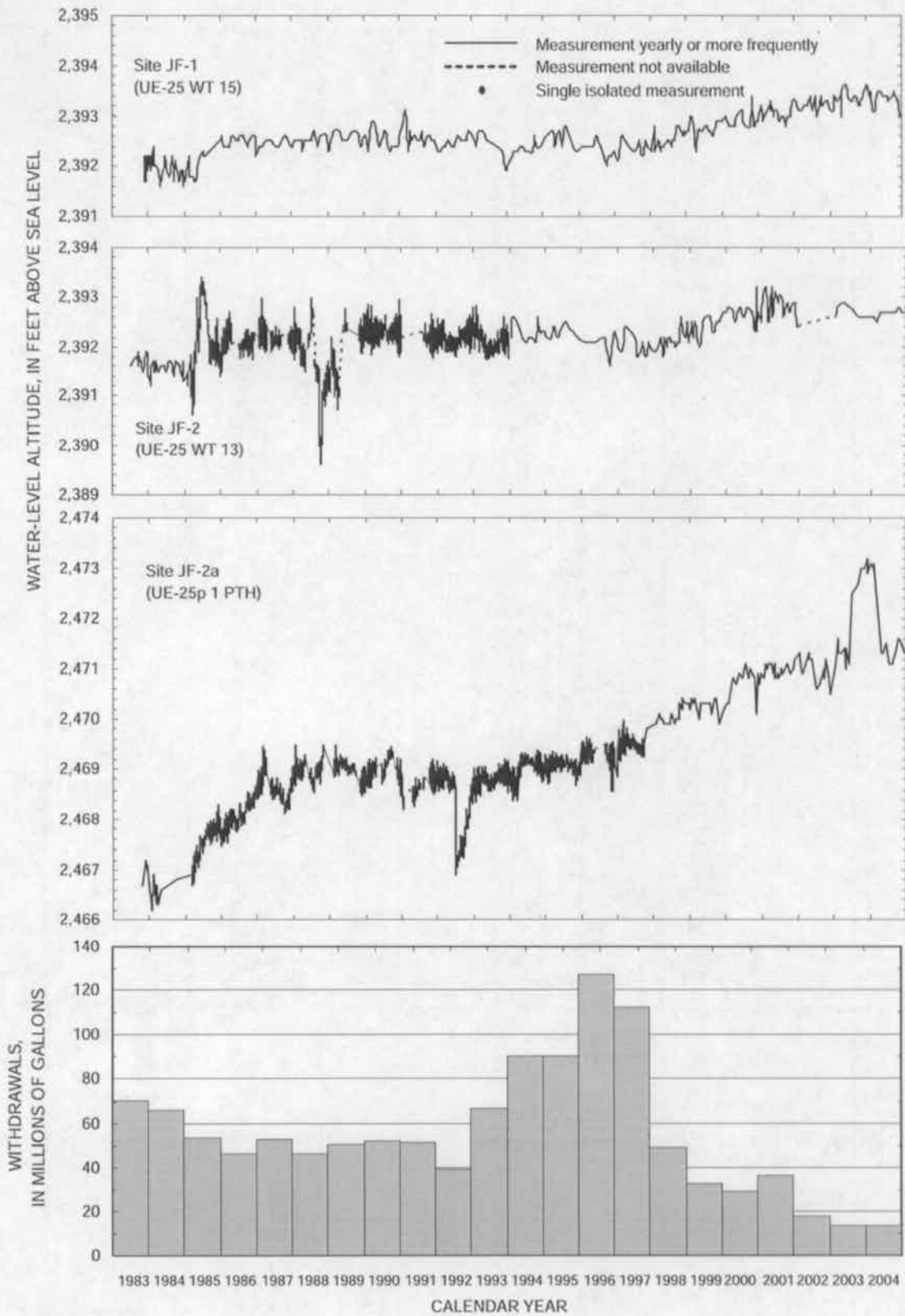
Figure 13. Water-level altitudes in boreholes JF-1, JF-2, JF-2a, J-13, J-11, J-12, and JF-3 and estimated annual groundwater withdrawals from Jackass Flats, 1983–2004. Periodic measurements that may reflect short-term conditions at a site have been excluded.
