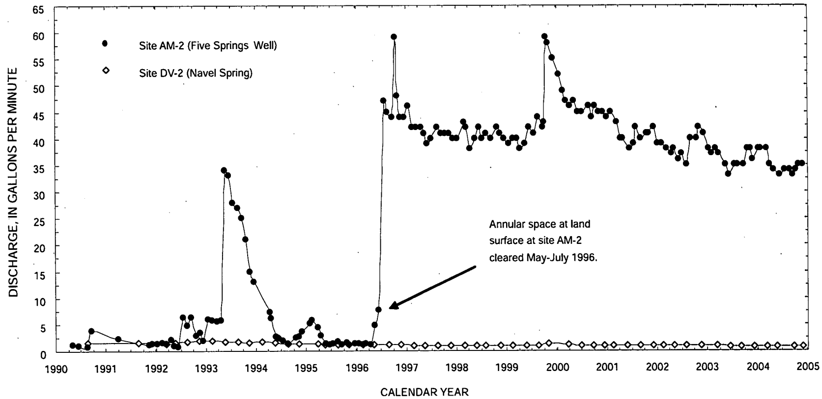
Figure 8. Discharge at sites AM-2 (Five Springs Well) and DV- 2 (Navel Spring), 1990–2004. Symbols shown on lines indicate periodic measurements presented in this and previous reports on selected ground-water data for Yucca Mountain region.
