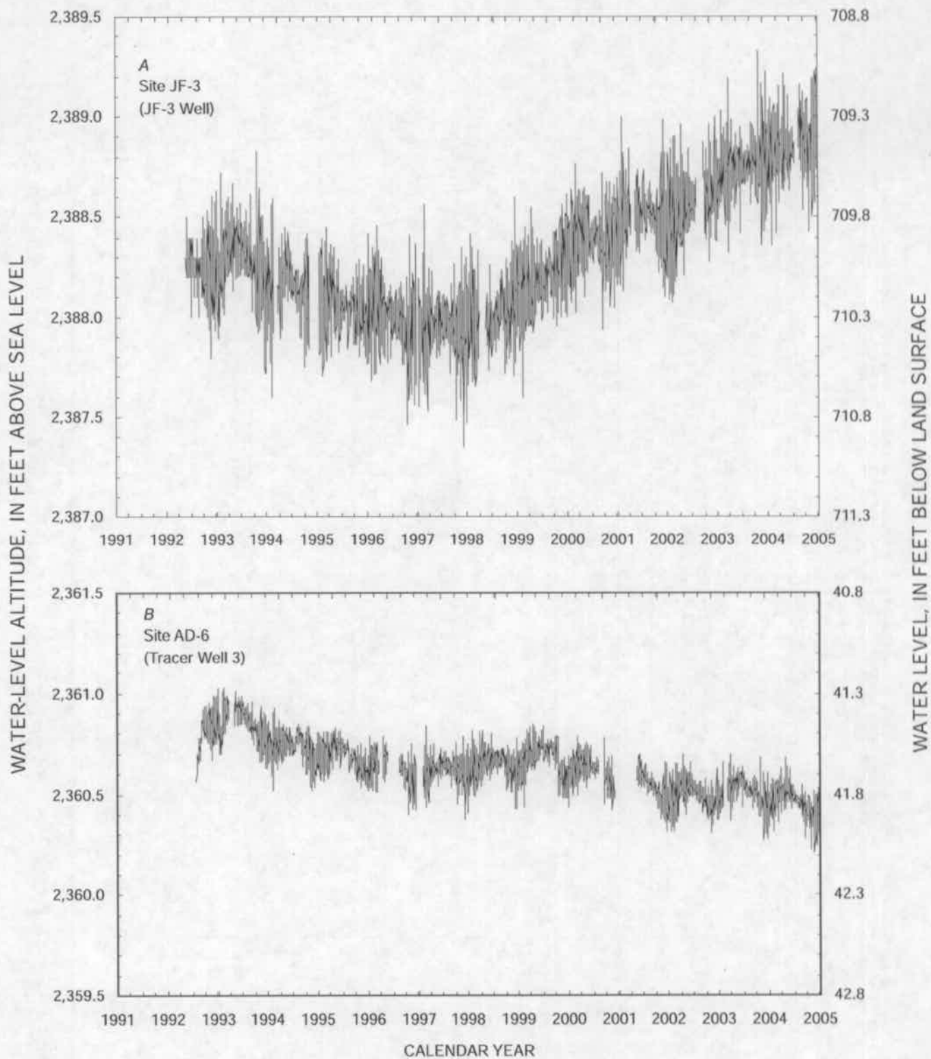
Figure 6. Daily mean water levels in (A) borehole JF-3, May 1992–December 2004 and in (B) borehole AD-6, July 1992–December 2004.
