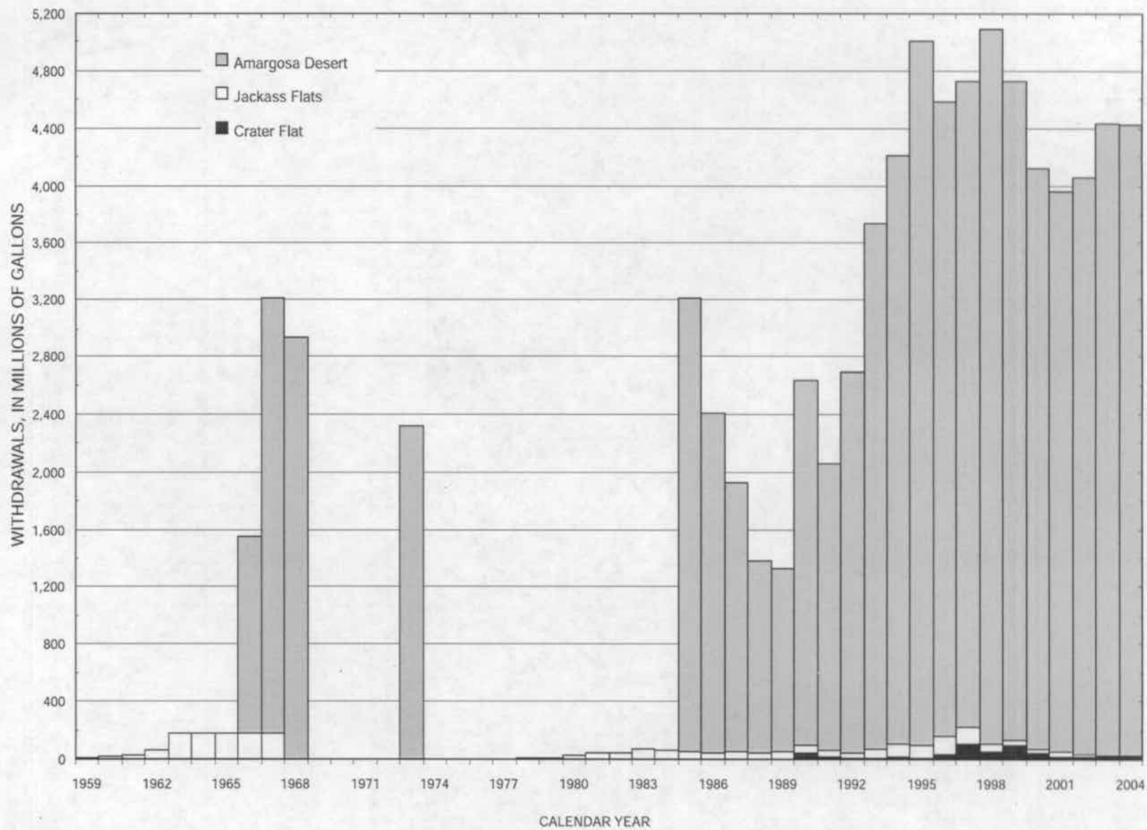
Figure 11. Available estimates of annual ground-water withdrawals for selected areas within Alkali Flat–Furnace Creek Ranch ground-water subbasin, 1959–2004.
