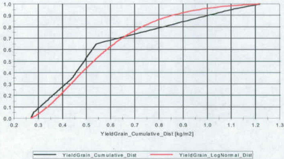
Figure 18. Comparison of Distributions for Grain Yield
