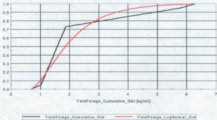
Figure 19. Comparison of Distributions for Forage Yield
