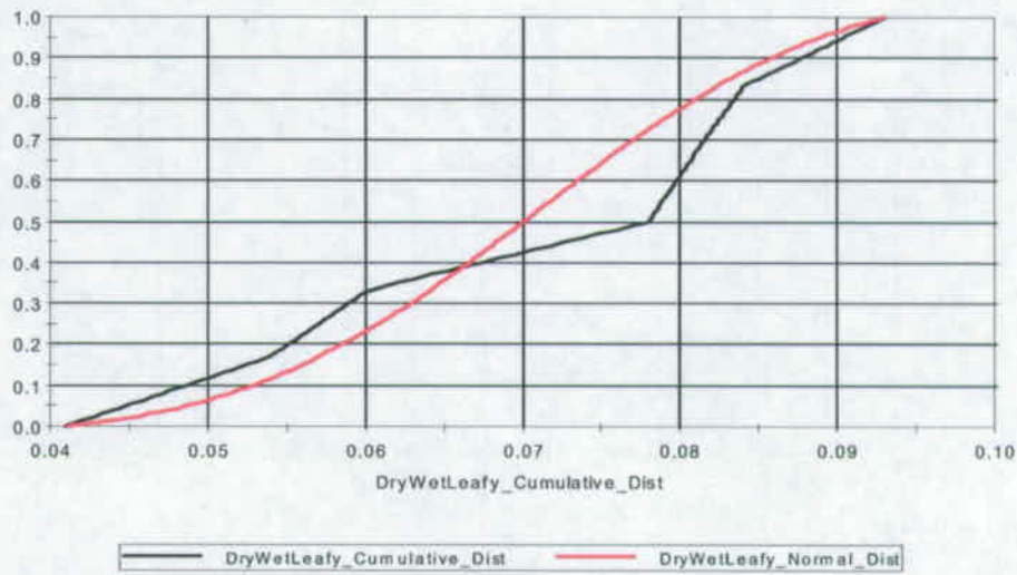
Figure 10. Comparison of Distributions for Dry/Wet Ratio for Leafy Vegetables
