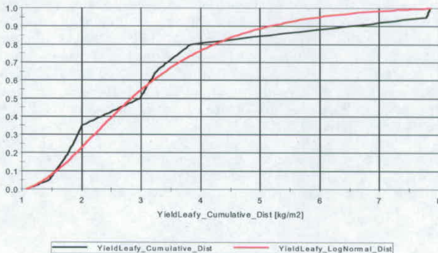
Figure 15. Comparison of Distributions for Leafy Vegetables Yield
