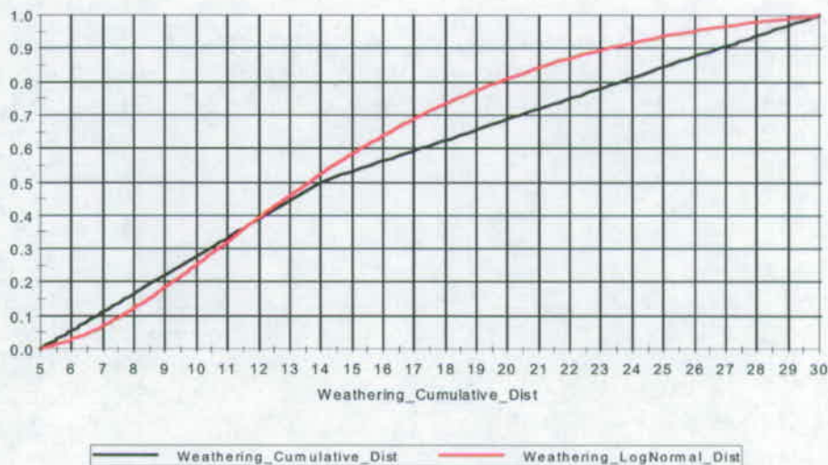
Figure 2. Comparison of Distributions for Weathering Rate Constant
