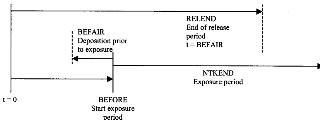
Figure 22. Exposure and Release Time Parameters
