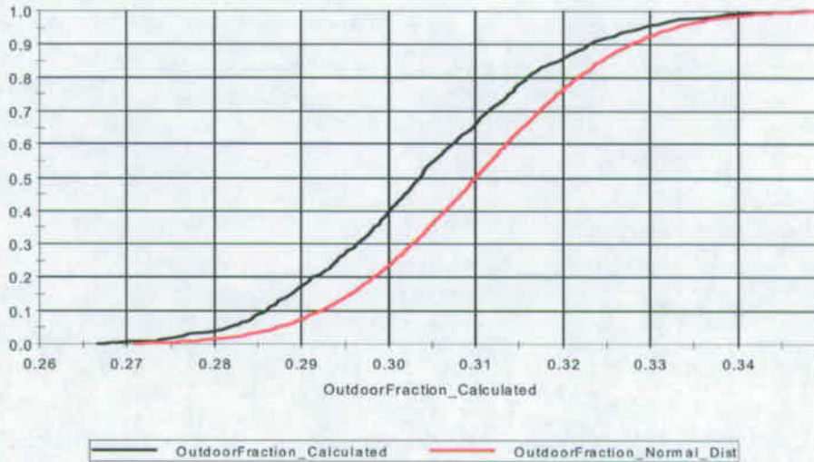
Figure 24. Comparison of Distributions for Outdoor Fraction
