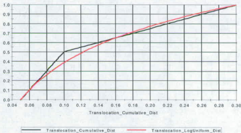
Figure 1. Comparison of Distributions for Translocation Factors
