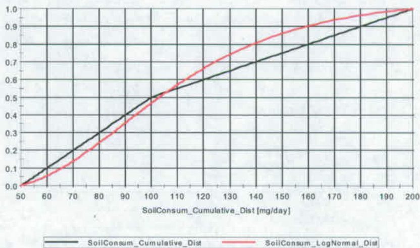
Figure 27. Comparison of Distributions for Inadvertent Soil Ingestion Rate
