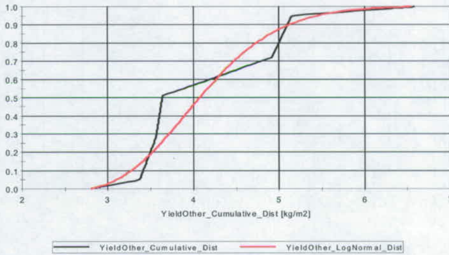
Figure 16. Comparison of Distributions for Root Vegetables Yield
