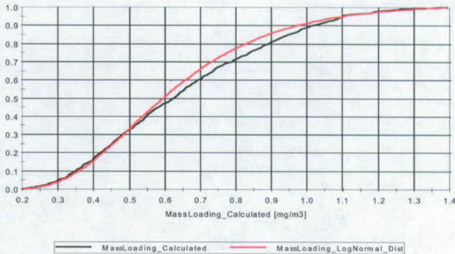
Figure 21. Comparison of Distributions for Mass Loading factor
