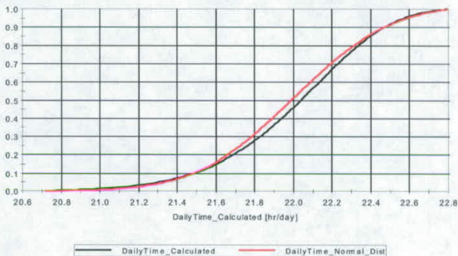
Figure 23. Comparison of Distributions for Daily Exposure Time
