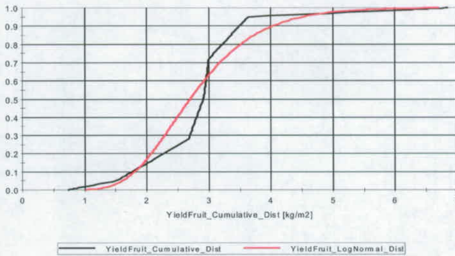
Figure 17. Comparison of Distributions for Fruit Yield
