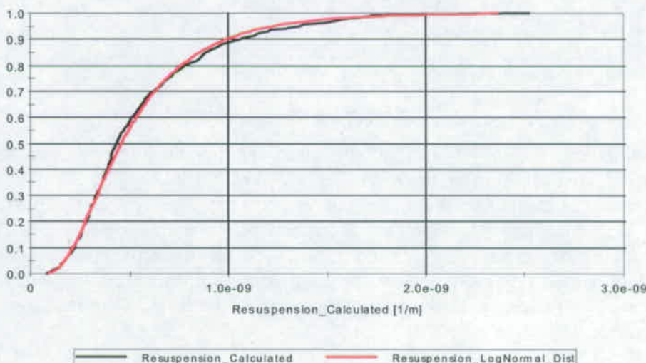
Figure 20. Comparison of Distributions for Resuspension Factor
