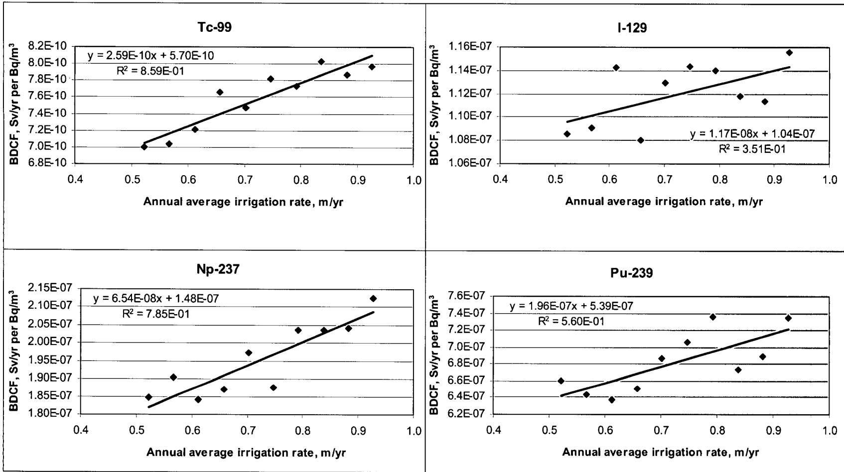
Figure 6.11-1. Graphical Representation of Dependence BDCFs for 99 Tc, 129 I, 237 Np, and 239 Pu on Annual Average Irrigation Rate
