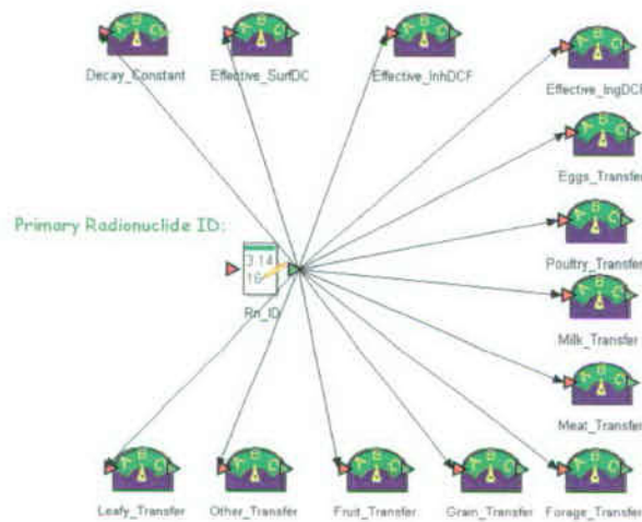
Figure 6.9-2. Biosphere Model for the Volcanic Ash Scenario
