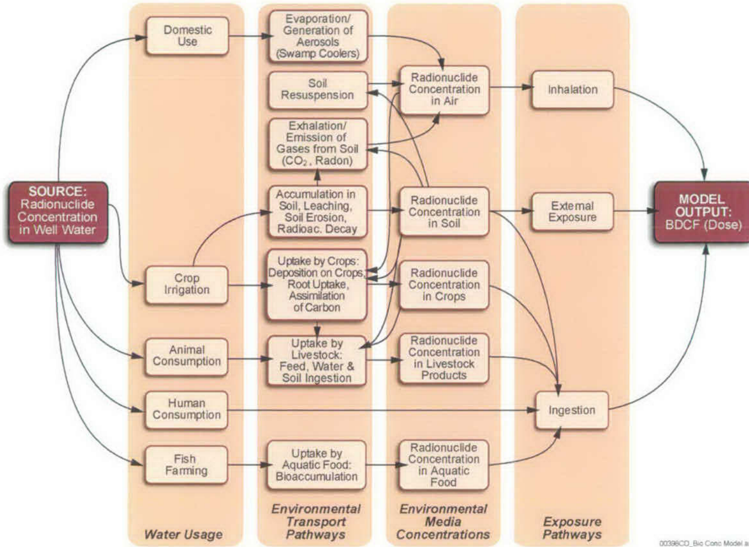
Figure 6.3-3. Conceptual Representation of the Biosphere Model for the Groundwater Exposure Scenario
