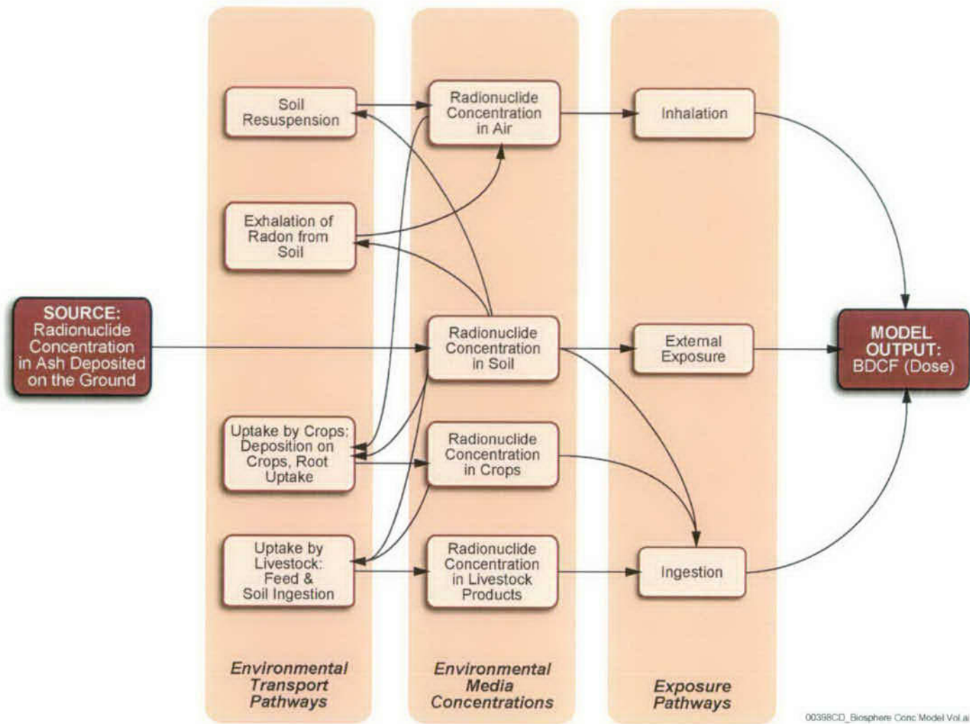
Figure 6.3-6. Conceptual Representation of the Biosphere Model for the Volcanic Ash Exposure Scenario
