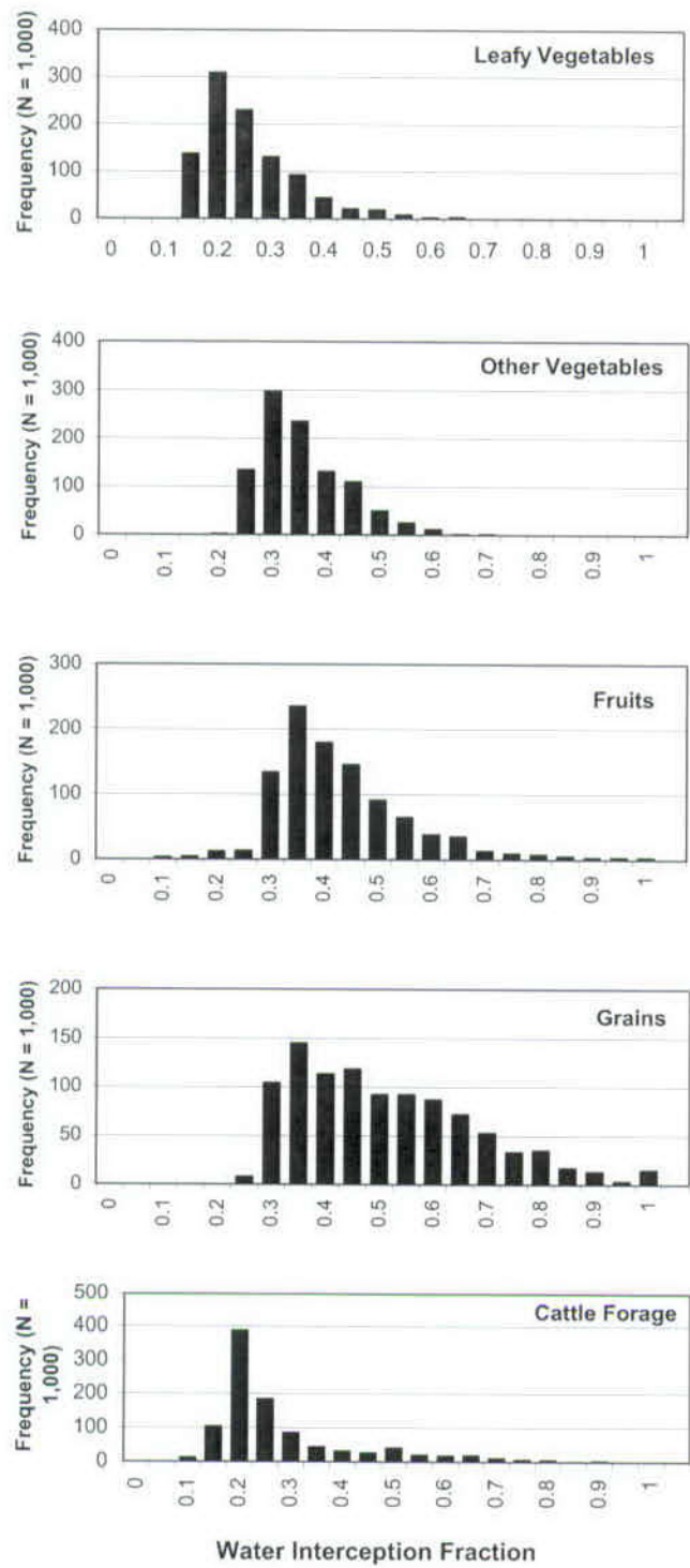
Figure 6.13-23. Water Interception Fraction Histograms by Crop Type Resulting from 1,000 Realizations of the Biosphere Model
