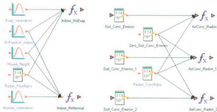
Figure 6.8-17. C14_Air Container of the Air Submodel
