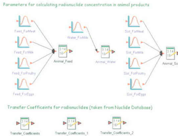
Figure 6.8-22. Input Parameter Container ( AnimalModel_Input ) for the Animal Submodel
