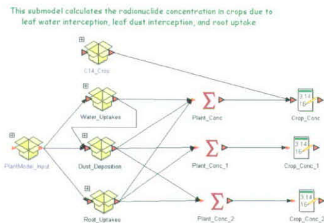
Figure 6.8-18. Plant Submodel Container
