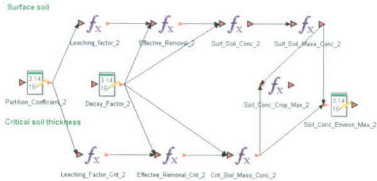
Figure 6.8-13. Soil Concentration Container for the Second Decay Product ( Soil_Conc_2 ) for the Soil Submodel
