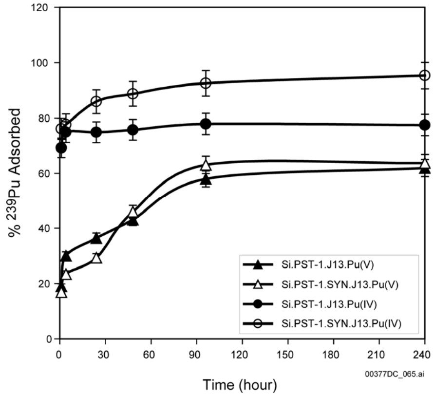
Figure 5-76. Sorption of 239 Pu onto Silica-PST-1 Colloids as a Function of Time in Natural and Simulated Groundwater
