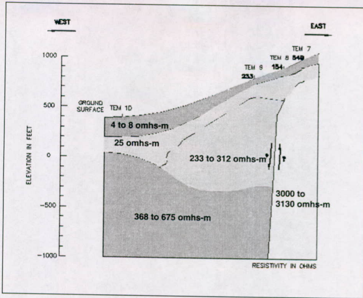
Figure 5.2-4 Nevares Springs Time Domain Electromagnetic Profile
