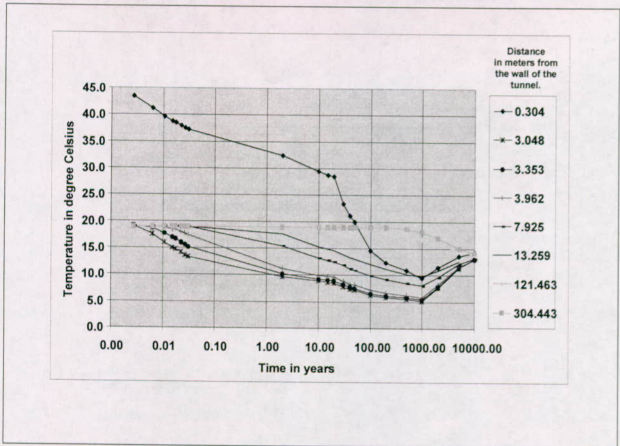
Figure 3.2-4 Reduction in Temperature versus Time and Distance from Tunnel Wall with a Decayed Heat Load, Assuming an Eddy Diffusivity Value of 0.01 and an Infiltration Rate of 4 mm/yr.
