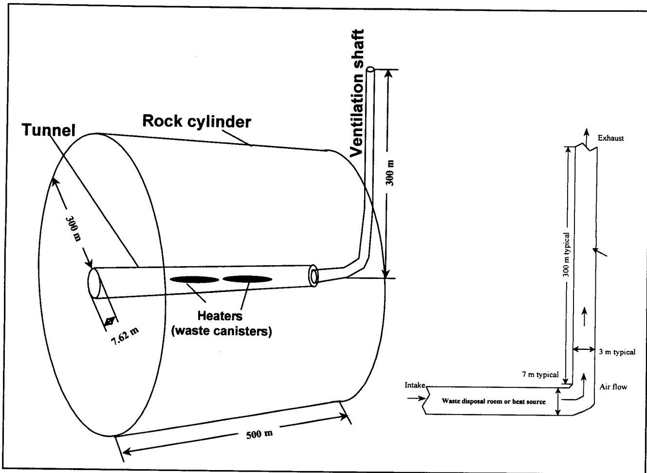
Figure 3.2-1 Three-Dimensional and Cross-Sectional View of the Axisymmetric Tunnel Model
