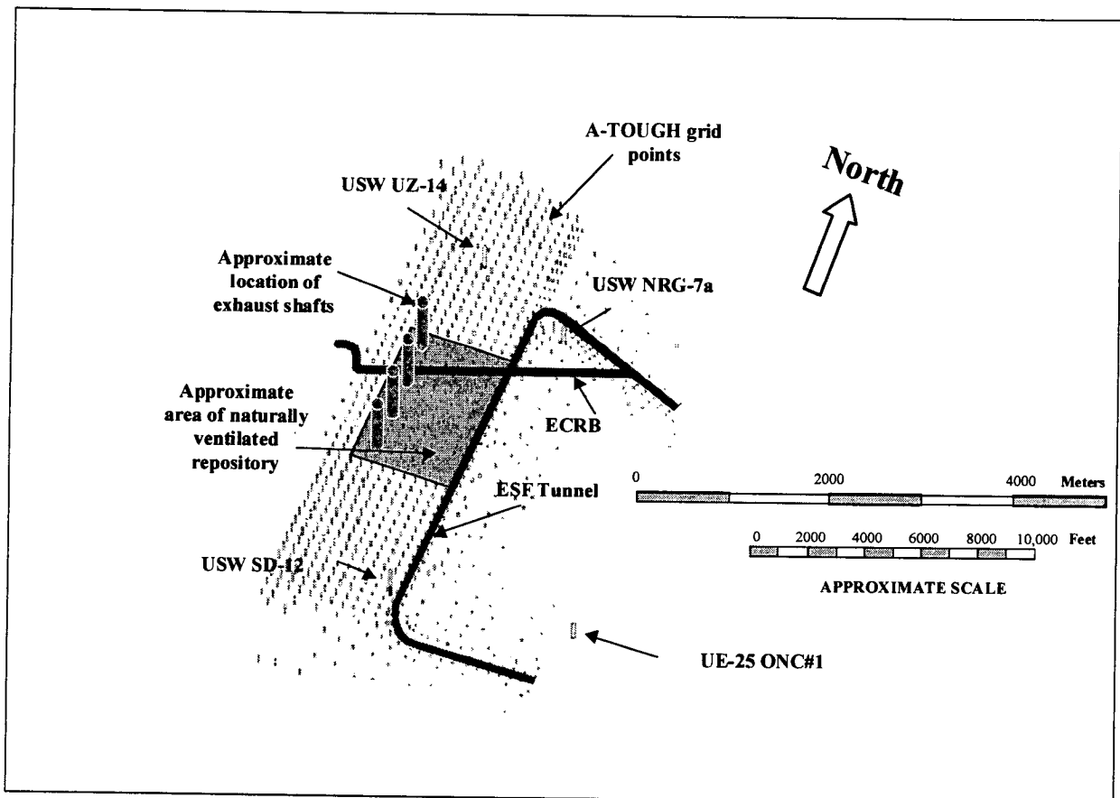
Figure 3.2-2 Oblique View of Modified Site-Scale Unsaturated Zone Model
