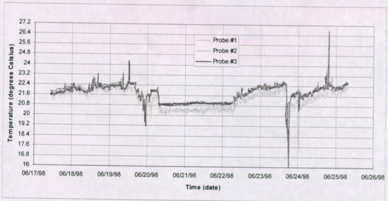
Figure 3.1-6b Temperature at Three Cross-Sectional Points in the Enhanced Characterization of the Repository Block
