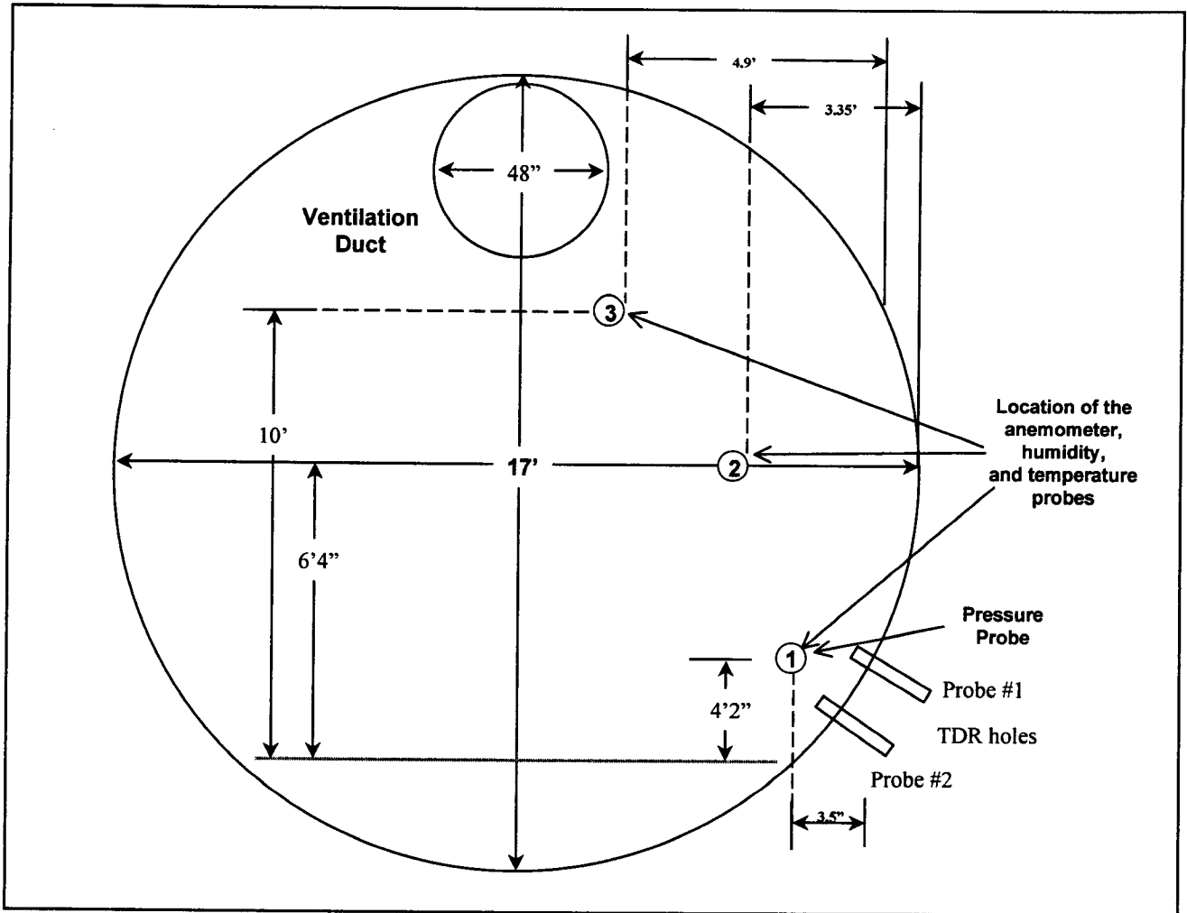
Figure 3.1-5 Location of Temperature, Pressure, Humidity, Anemometer, and Time-Domain Reflectometry Probes in the Enhanced Characterization of the Repository Block
