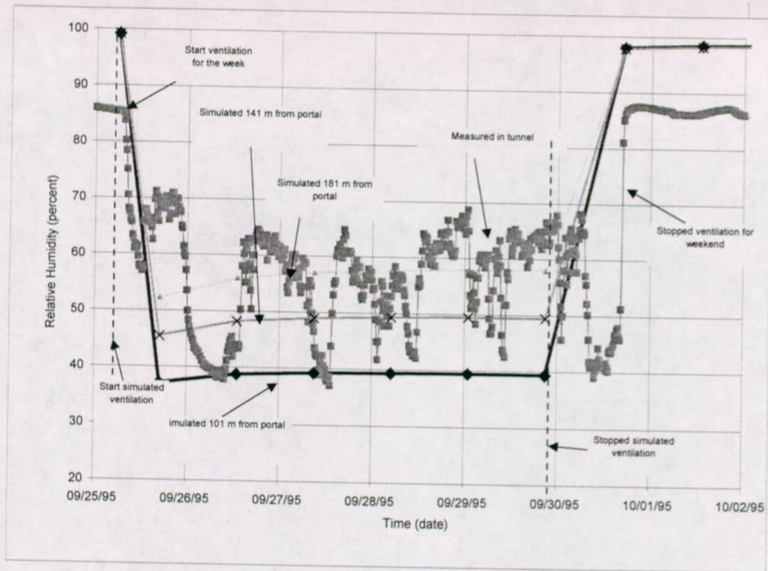
Figure 3.2-5 Comparison between Measured and Simulated Relative Humidity in the Exploratory Studies Facility Tunnel during Construction, Assuming an Eddy Diffusivity Value of 0.01
