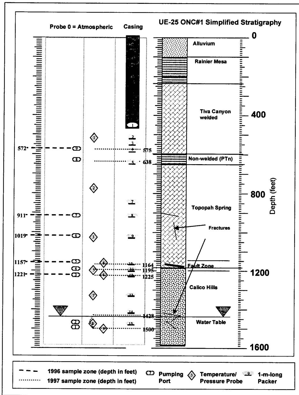
Figure 3.1-3 Schematic Diagram of the Instrumentation and Simplified Stratigraphy in UE-25 ONC#1
