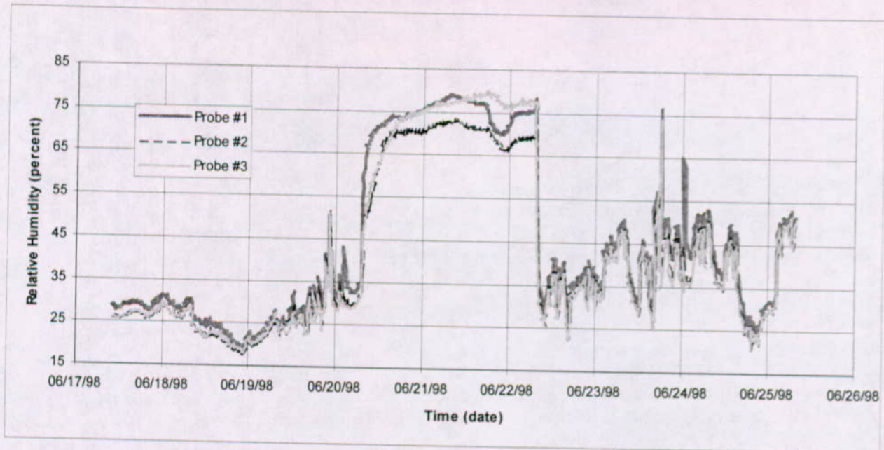
Figure 3.1-6a Relative Humidity at Three Cross-Sectional Points in the Enhanced Characterization of the Repository Block
