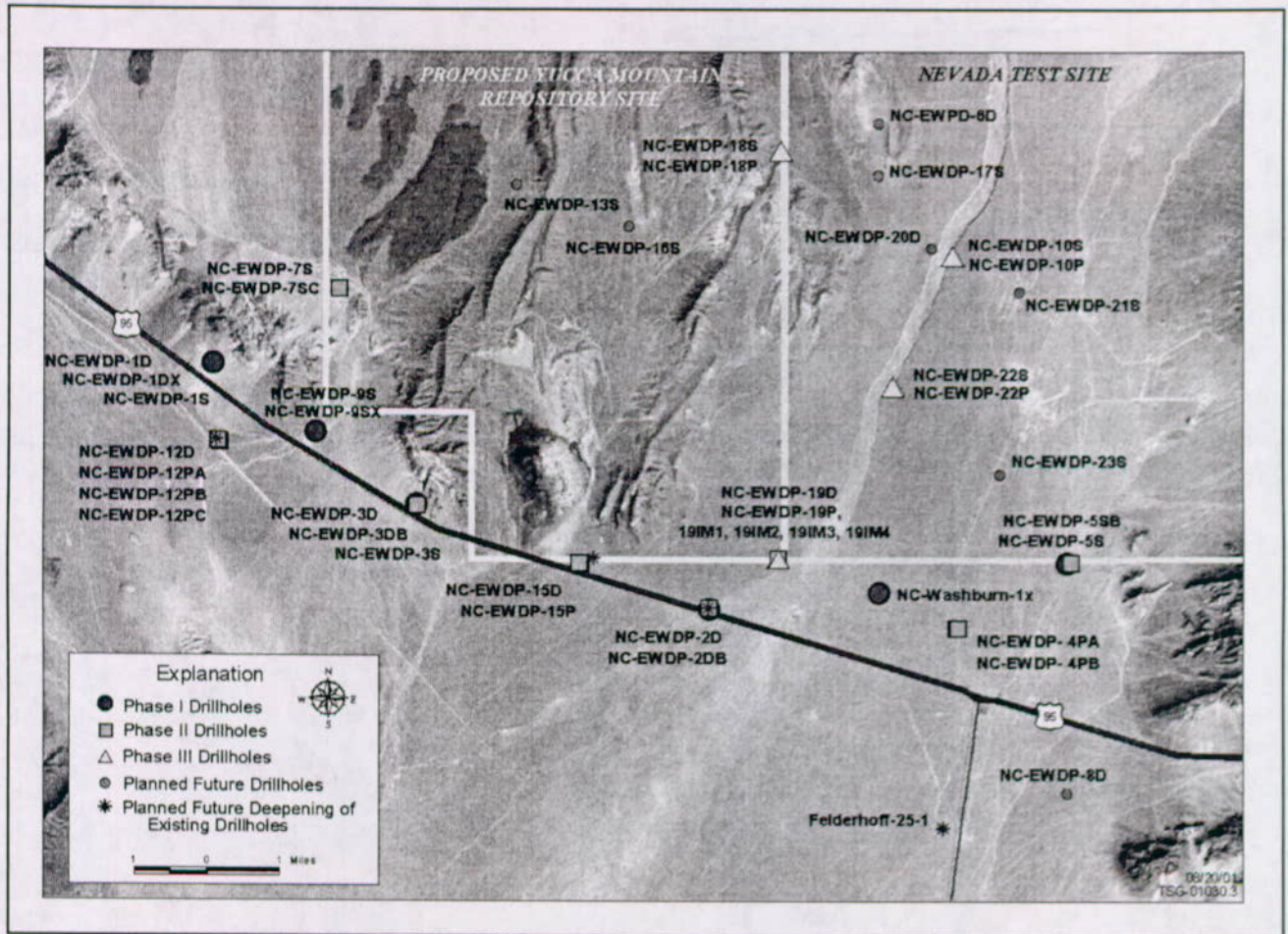
Figure 4.1-1 Location of Early Warning Drilling Program Drillholes
