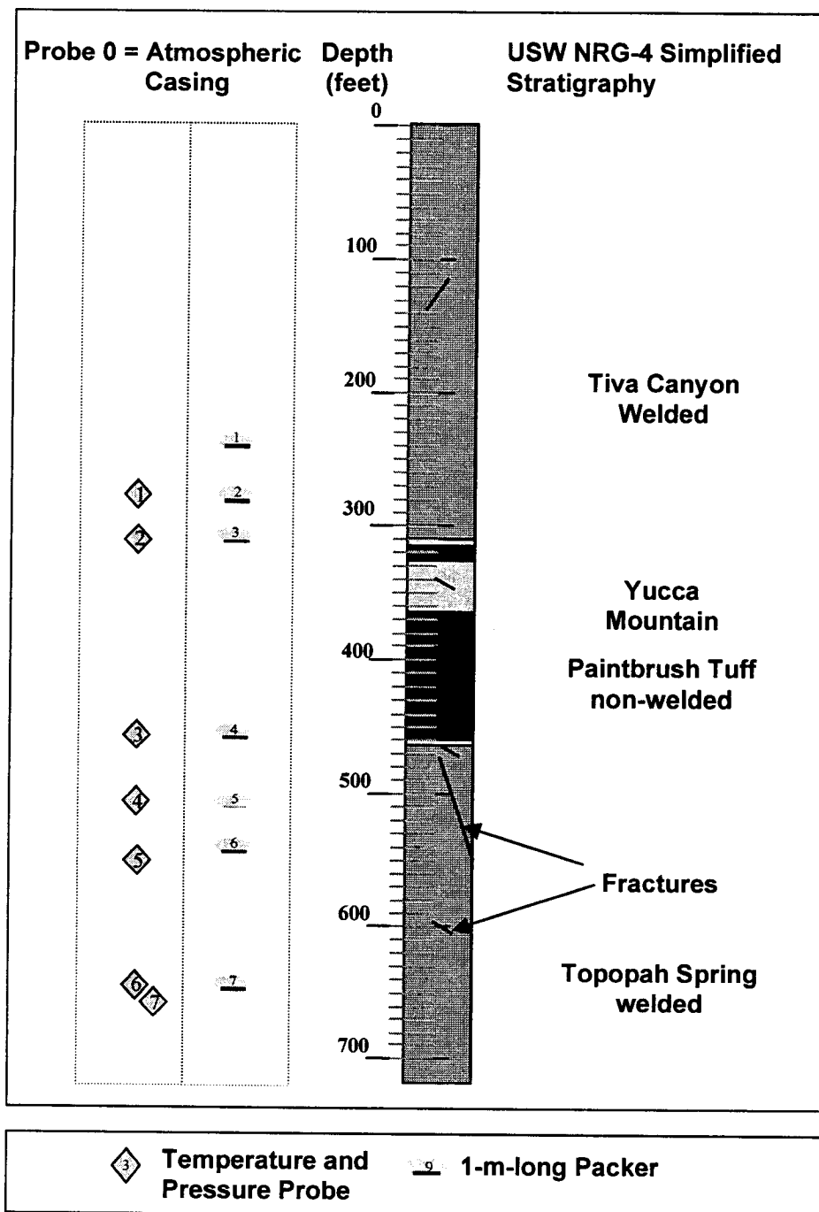
Figure 3.1-2 Schematic Diagram of the Instrumentation and Simplified Stratigraphy in USW NRG-4
