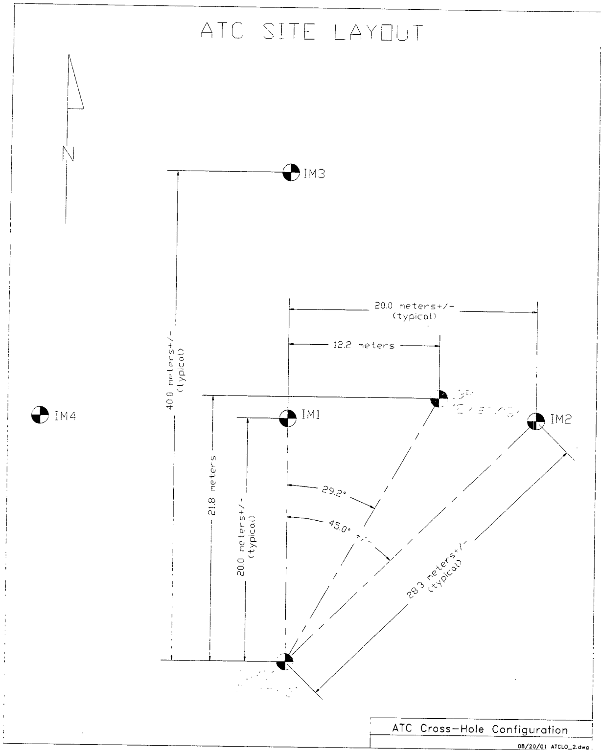
Figure 4.2-7 Proposed Alluvial Testing Complex Configuration for Cross-Hole Testing
