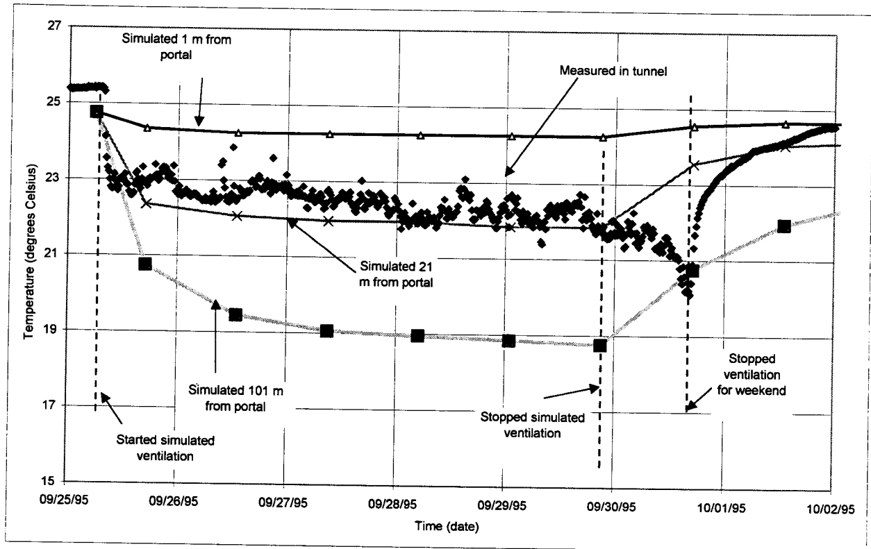
Figure 3.2-6 Comparison between Measured and Simulated Temperature in the Exploratory Studies Facility during Construction, Assuming an Eddy Diffusivity Value of 0.01
