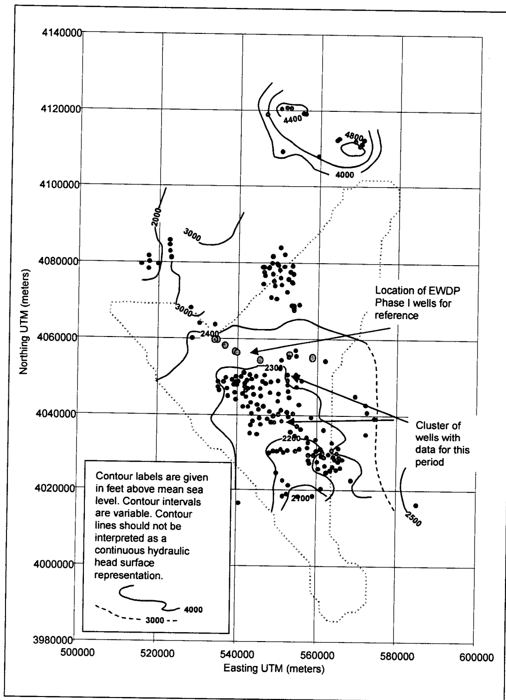
Figure 4.3-2b Water Level Elevations in Feet Averaged for the Period 1990 to 1997 (5,651 water level measurements at 325 locations)
