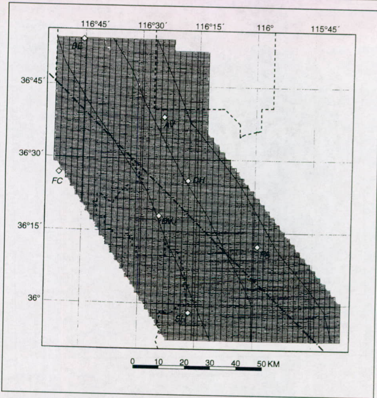
Figure 2.1-1 Location of Flight Lines for Magnetic Survey
