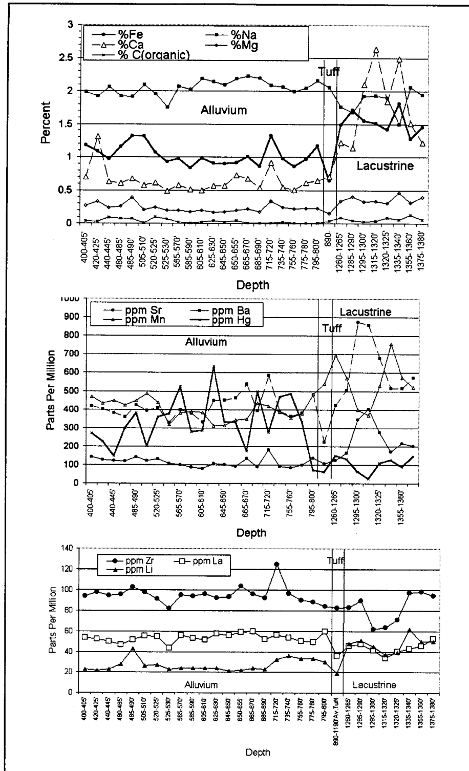
Figure 4.1-19 Trace Element Distribution, NC-EWDP-19D
