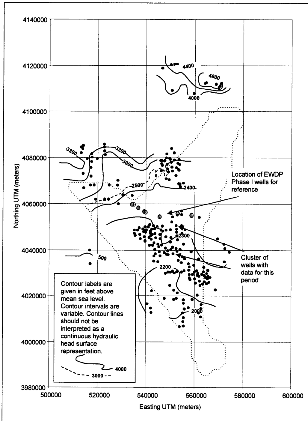
Figure 4.3-2a Water Level Elevations in Feet Averaged for the Period 1980 to 1989 (11,310 water level measurements at 503 locations)
