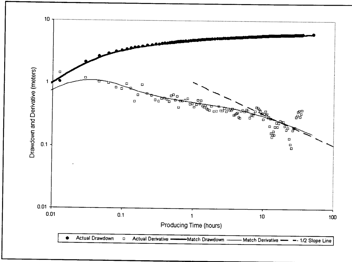
Figure 4.1-12 Log-Log Diagnostic Plot for NC-EWDP-3D Showing -1/2 Slope in Derivative Characteristic of Spherical Flow
