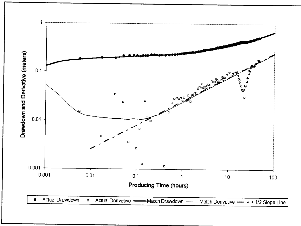
Figure 4.1-14 Log-Log Diagnostic Plot for NC-EWDP-1S Showing + \frac{1}{2} Slope in Derivative Characteristic of Parallel Boundaries
