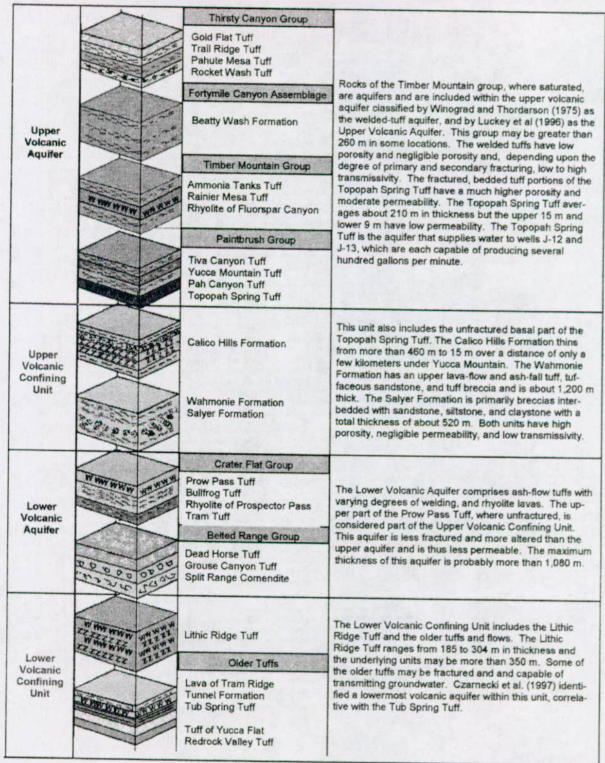
Figure 4.1-9 Major Volcanic Rock Units of the Yucca Mountain Region
