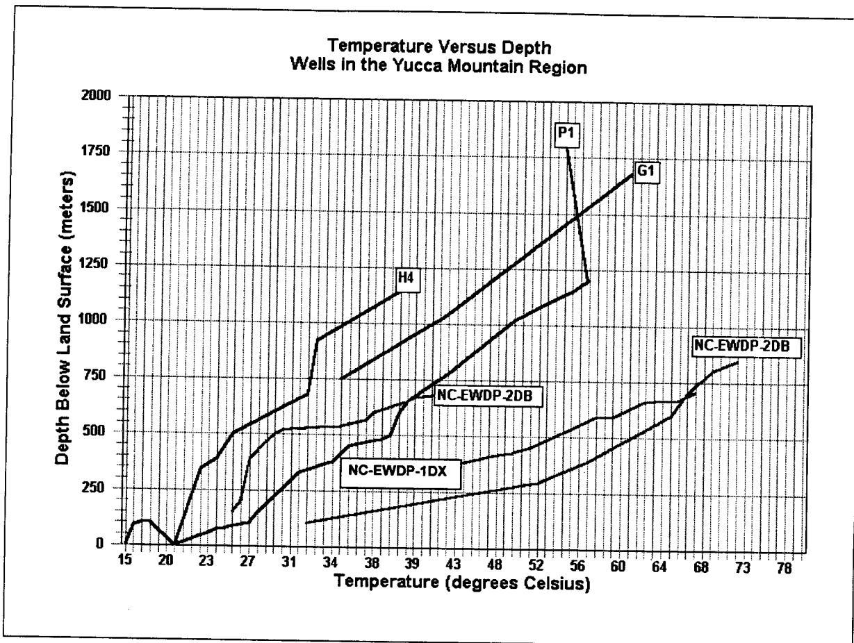
Figure 4.1-5 Temperature Logs for Selected Early Warning Drilling Program and Yucca Mountain Project Boreholes
