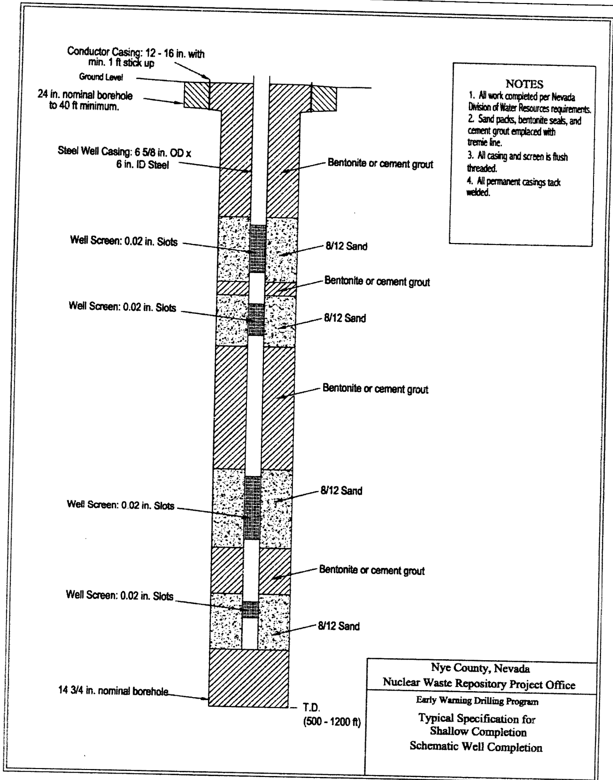
Figure 4.1-3 Typical Specification for Shallow Completion, Schematic Well Completion
