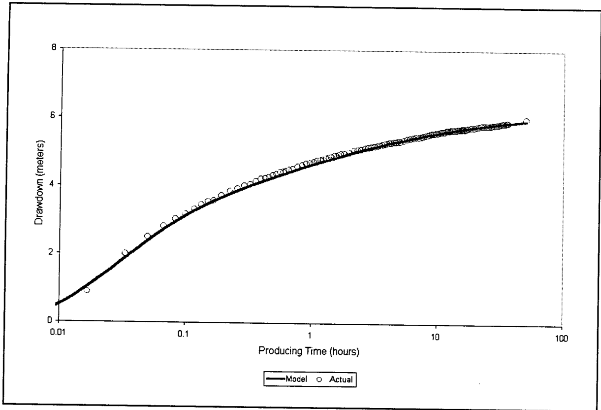
Figure 4.1-13 Semilog Cooper-Jacob Plot for NC-EWDP-3D
