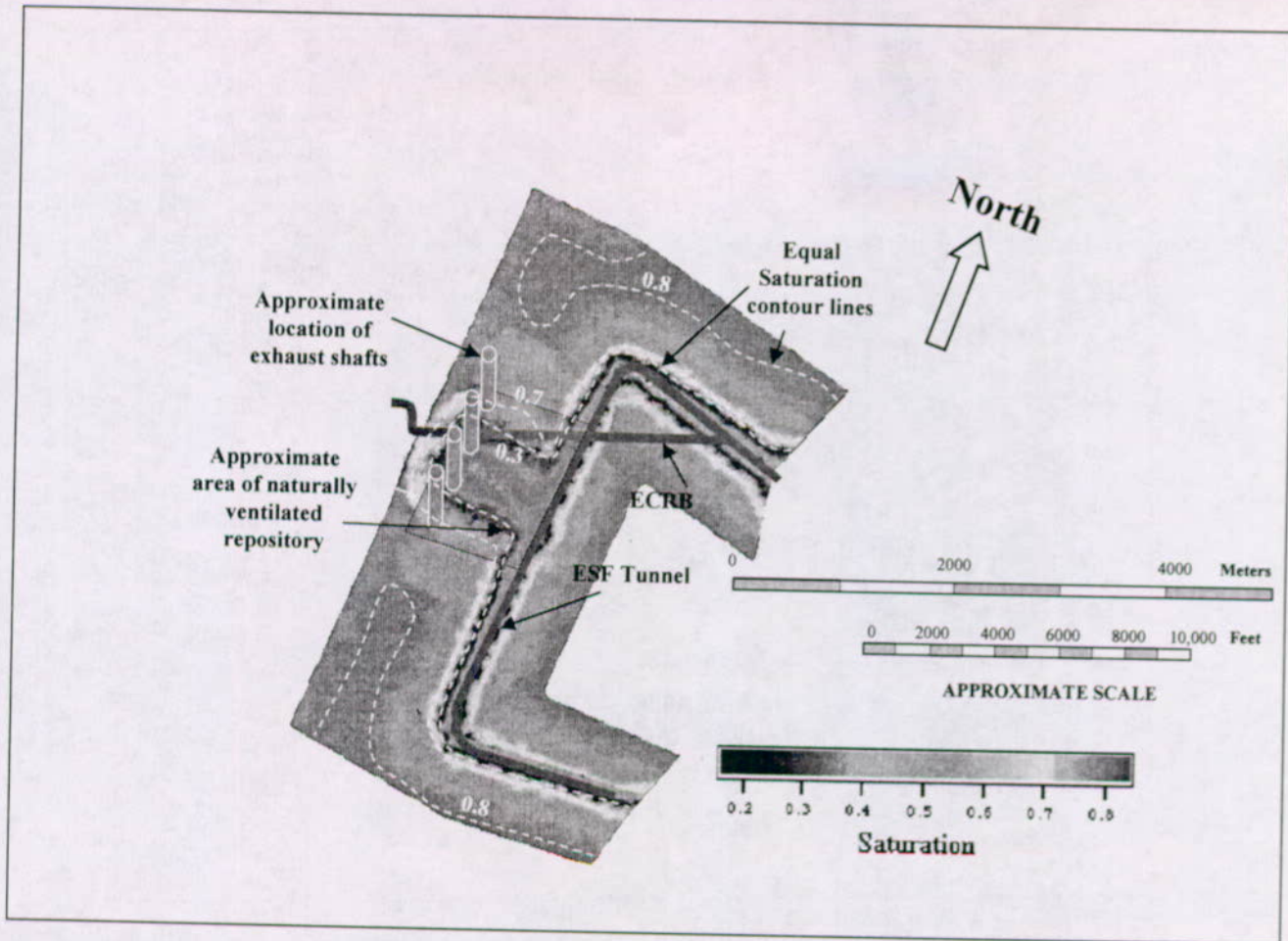
Figure 3.2-3 Reduction in Water Saturation at the Repository Horizon after 1,000 Years of Ventilation, Assuming an Eddy Diffusivity Value of 0.01 and an Infiltration Rate of 4 mm/yr.
