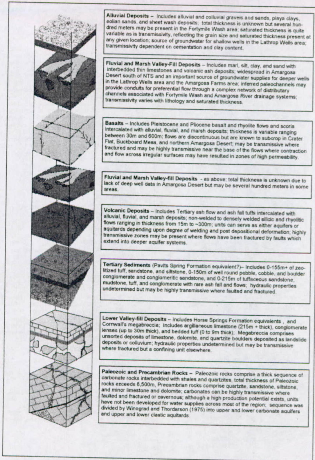
Figure 4.1-8 Major Valley-Fill and Older Units of the Yucca Mountain Region
