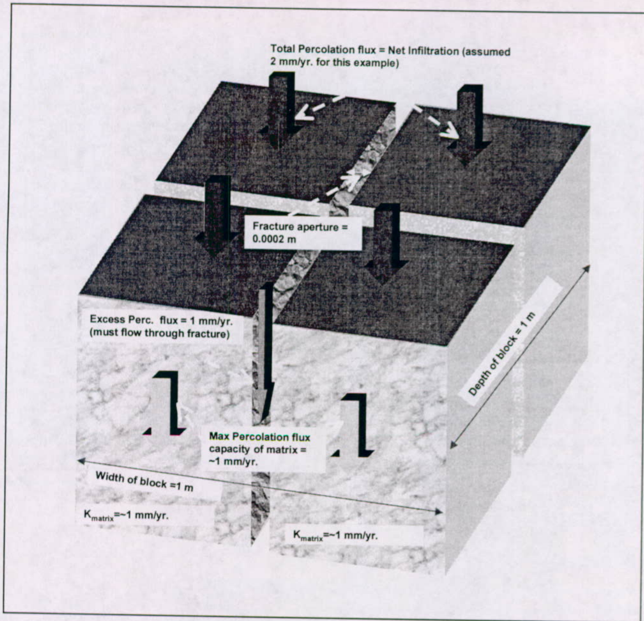
Figure 3.3-1 Conceptual Example Illustrating Assumptions Used for Calculating Percolation through a Fractured Tuff
