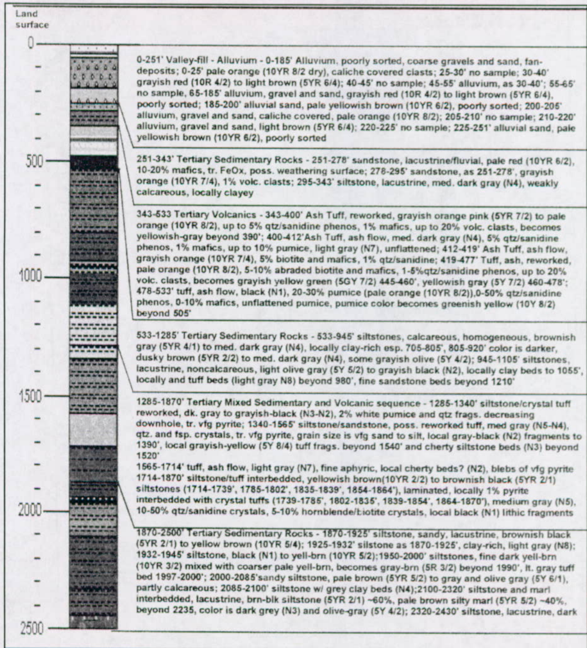
Figure 4.1-7 NC-EWDP-3D Summary Lithologic Log
