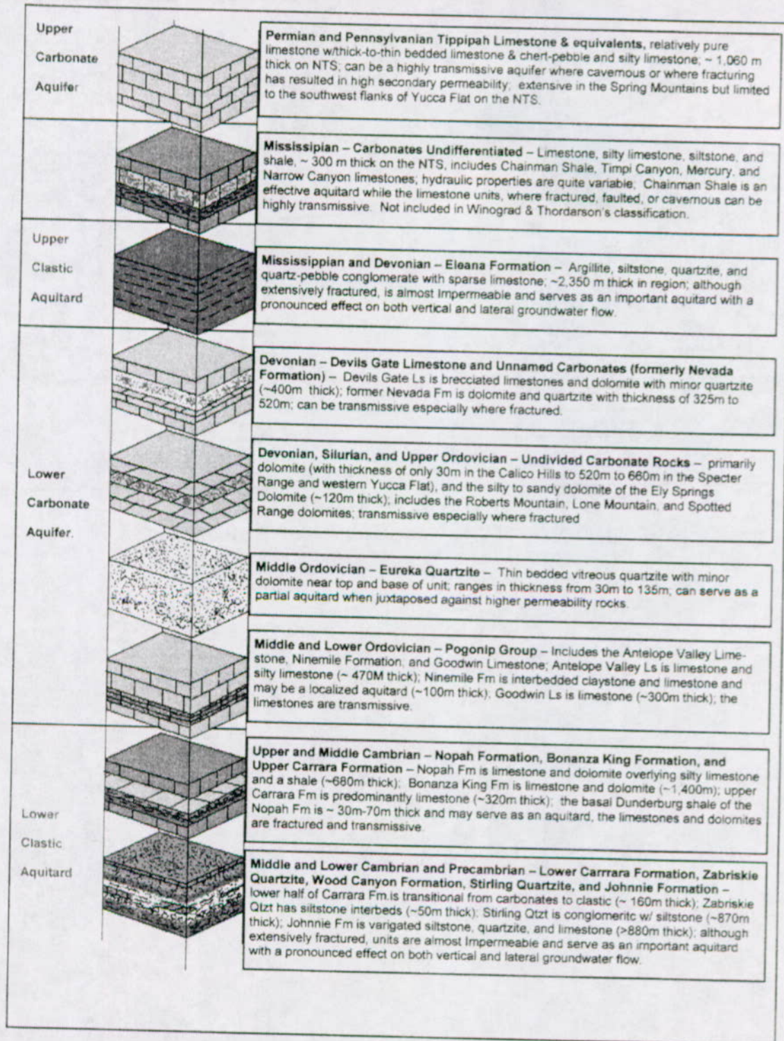
Figure 4.1-10 Major Paleozoic and Precambrian Rock Units of the Yucca Mountain Region
