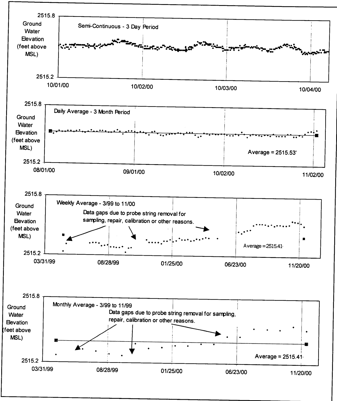
Figure 4.1-18 Water Level Variations in NC-EWDP-9SX for Various Time Periods
