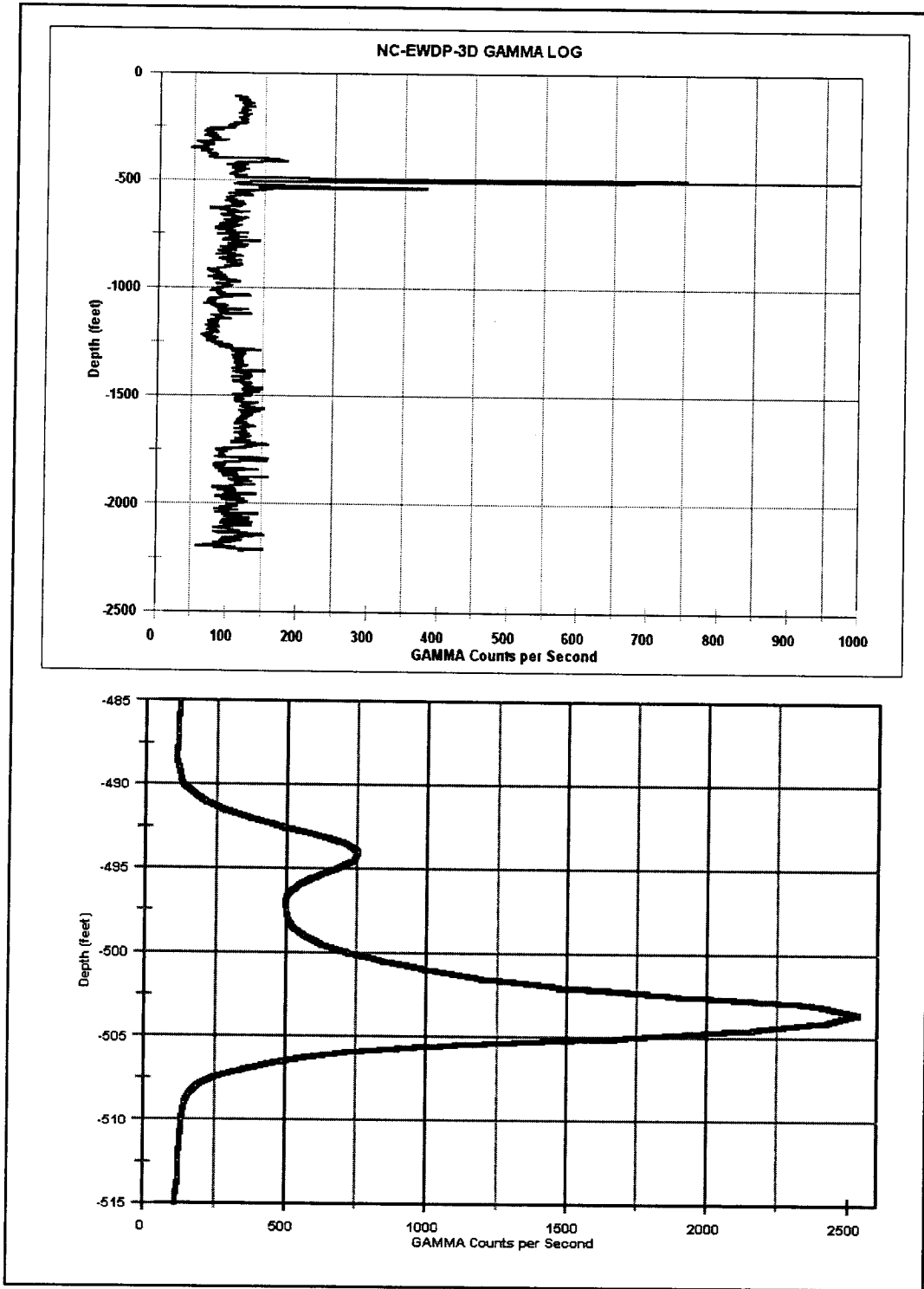
Figure 4.1-6 Natural Gamma Log for NC-EWDP-3D Showing the Gamma Spike
