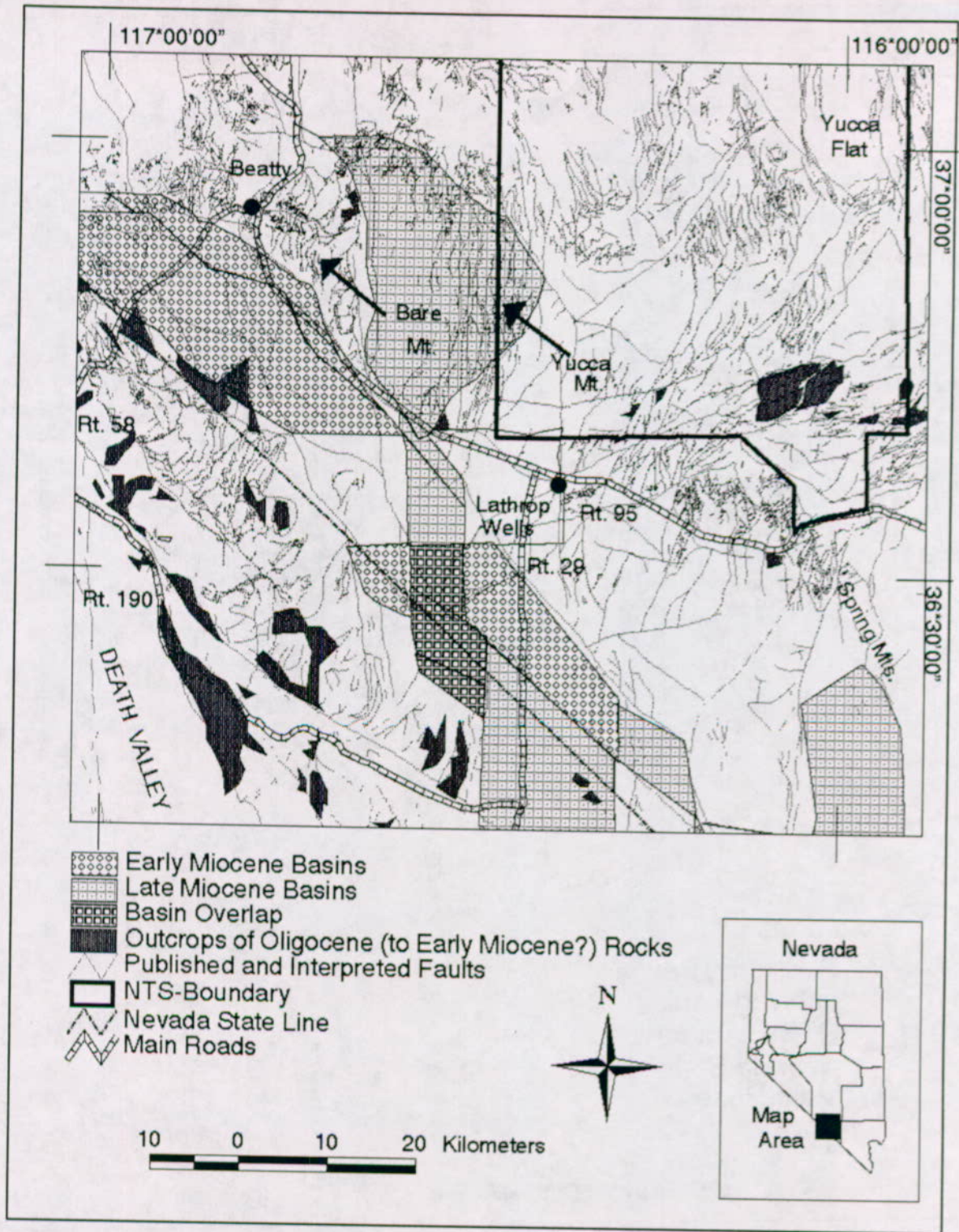
Figure 2.2-1 Structural Basins in the Yucca Mountain Region
