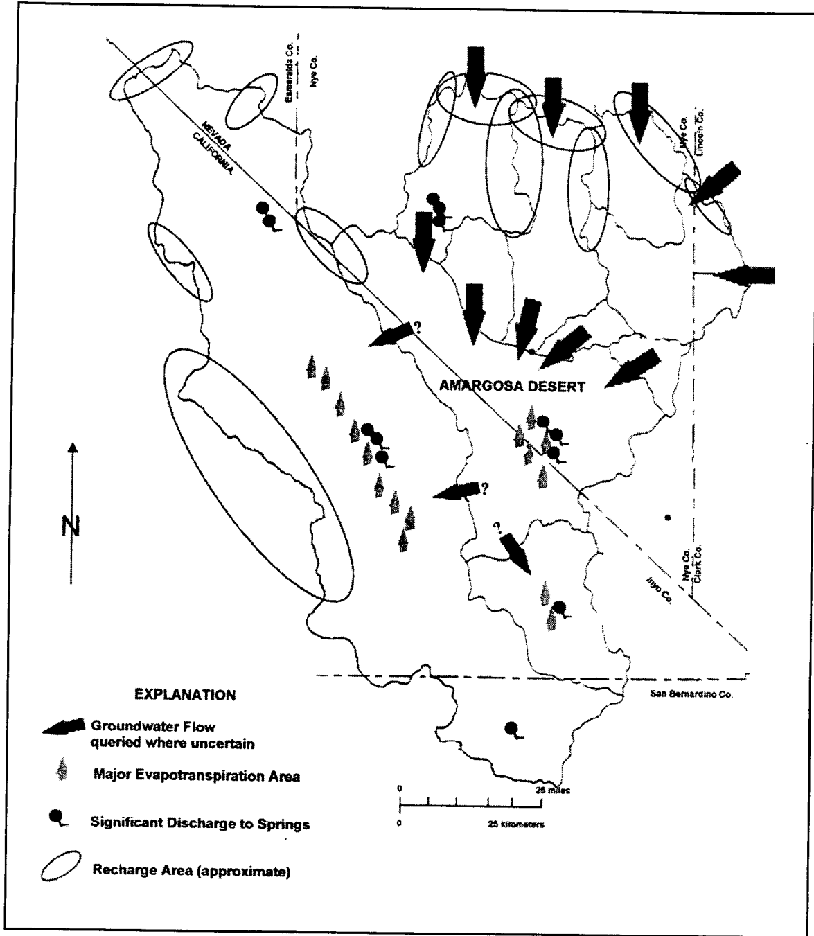
Figure 4.1-21 Recharge to and Discharge from Amargosa Desert
