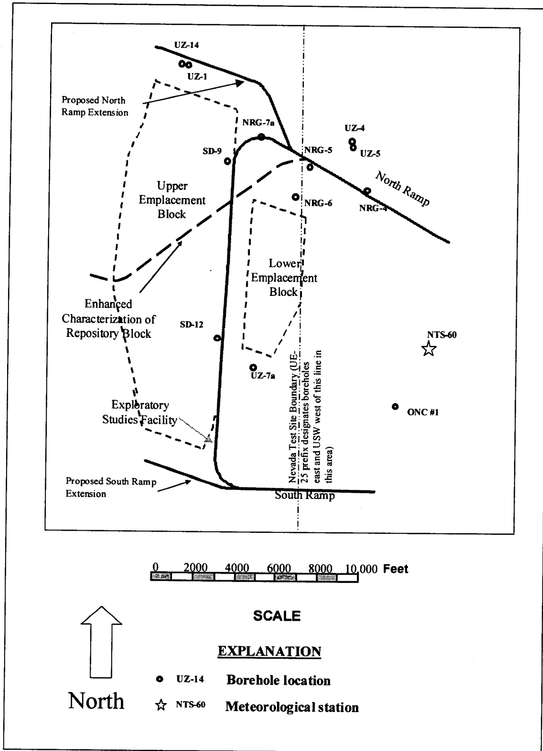
Figure 3.1-1 Location of Selected Boreholes, the Exploratory Studies Facility, and the Enhanced Characterization of the Repository Block at the Yucca Mountain Site
