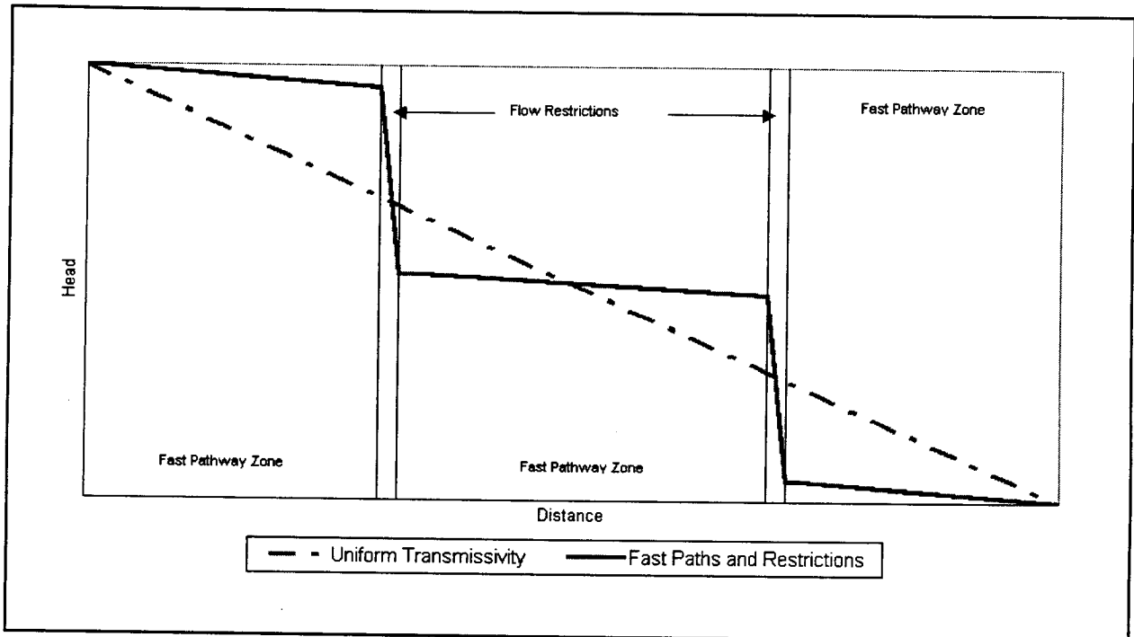
Figure 4.1-11 Conceptual Head Changes along a Flow Pathline
