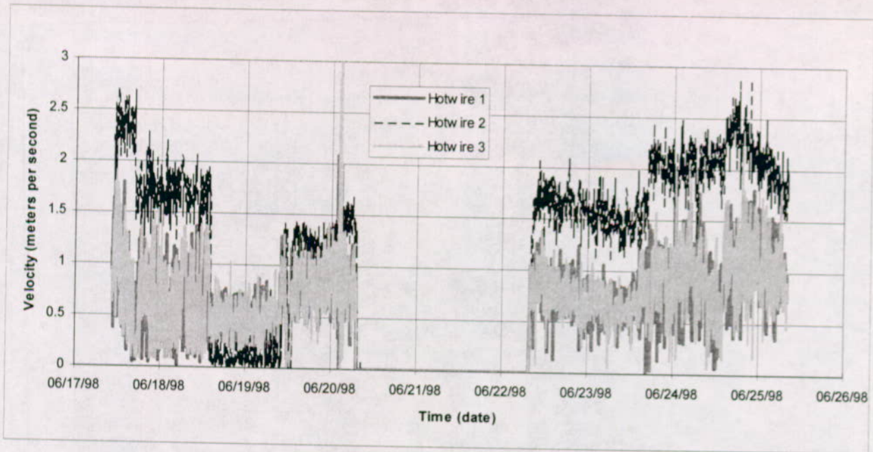
Figure 3.1-6c Relative Air Velocity Measured at Three Cross-Sectional Points in the Enhanced Characterization of the Repository Block
