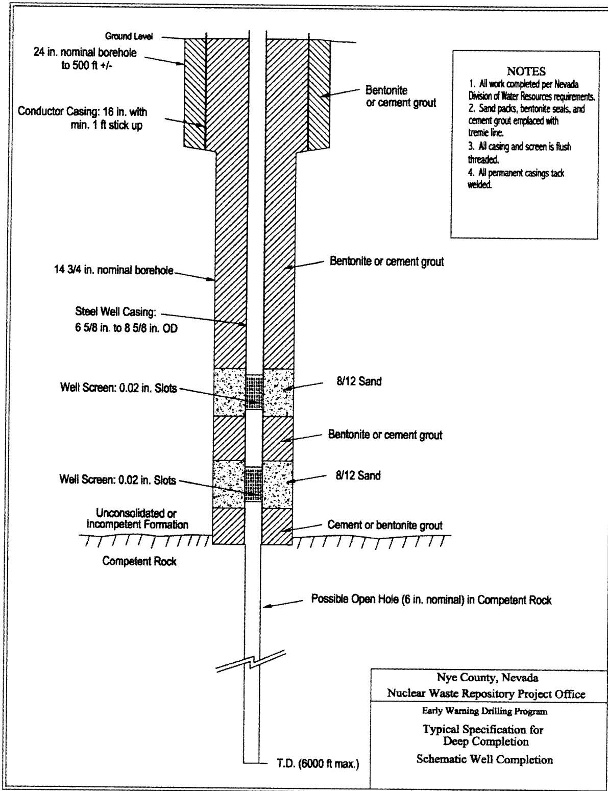
Figure 4.1-4 Typical Specification for Deep Completion, Schematic Well Completion
