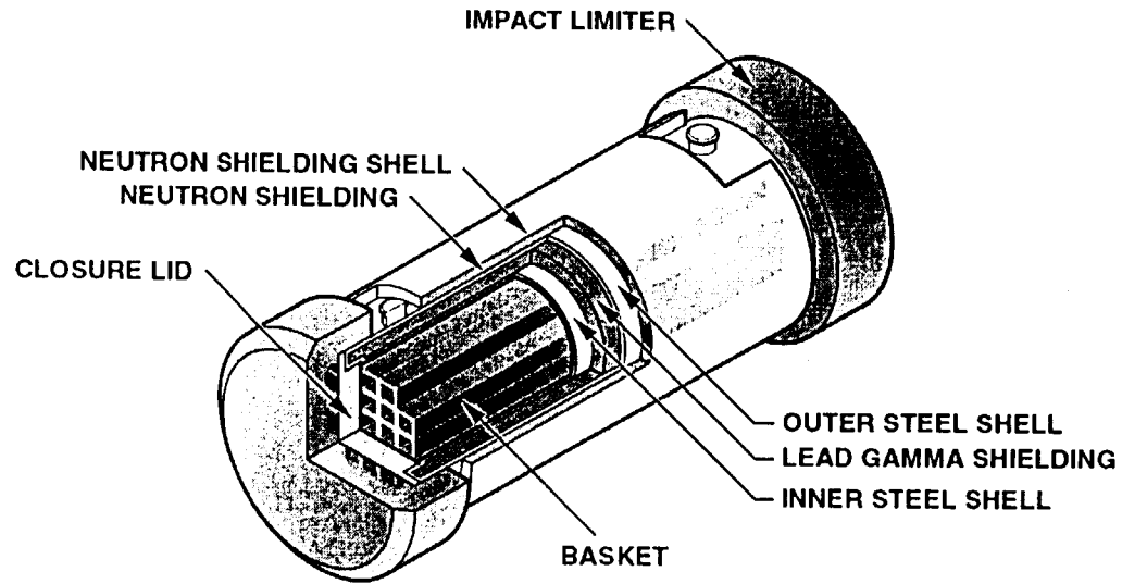
Figure 4.3 Conceptual design of a generic steel-lead-steel rail cask.
