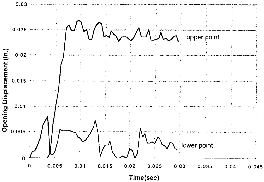
Figure A-56 Steel-DU-steel truck cask following a 30 mph corner impact
