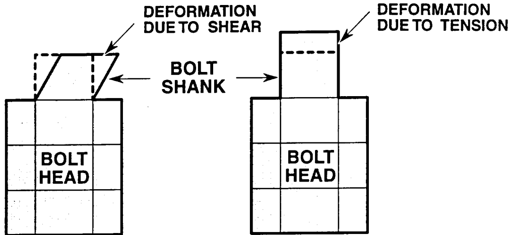
Figure 5.5 Modeling of the deformation in the bolts. The solid lines indicate the bolt position after being deformed and the dashed lines indicate the initial bolt position.
