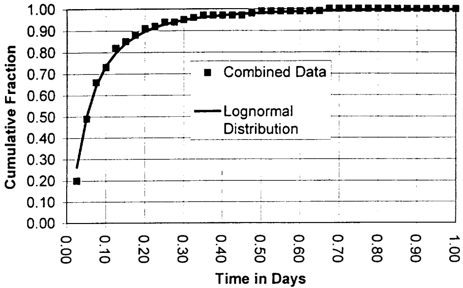
Figure 3.13 Distribution of response team arrival plus evacuation times.
