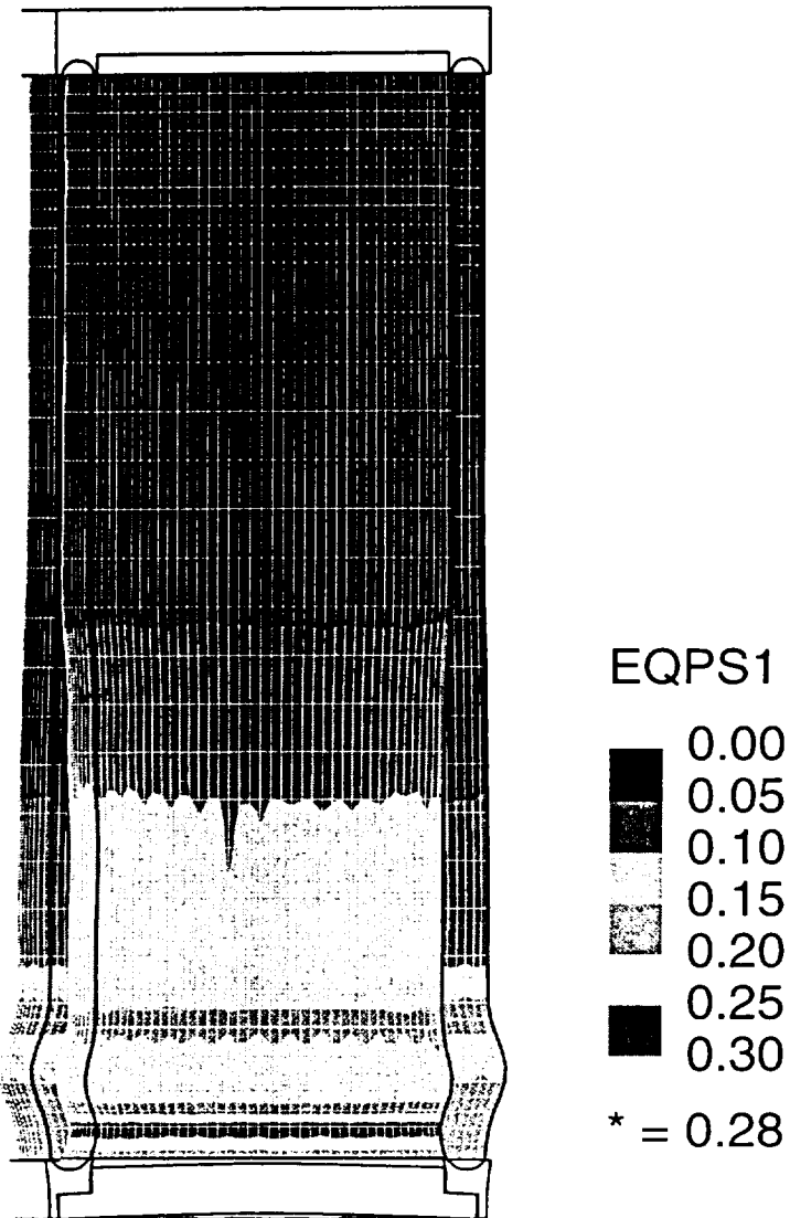
Figure A-29 Steel-lead-steel rail cask following a 120 mph end impact
