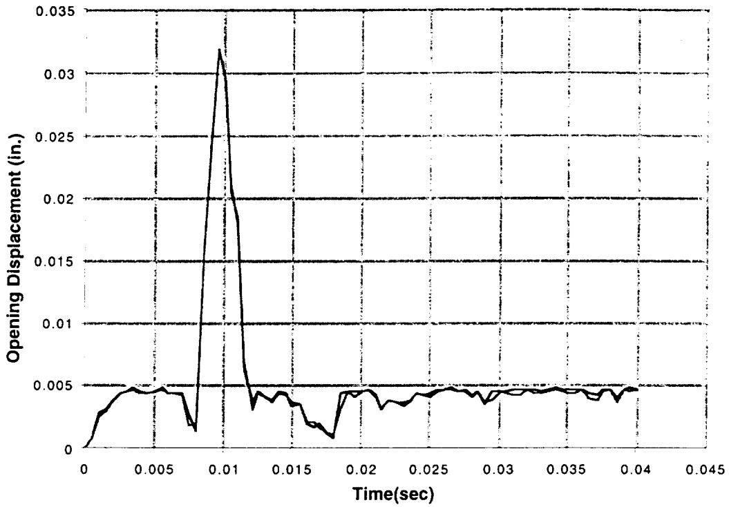
Figure A-73 Steel-lead-steel rail cask following a 90 mph end impact
