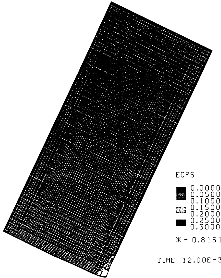
Figure A-33 Monolithic-steel rail cask following a 30 mph corner impact
