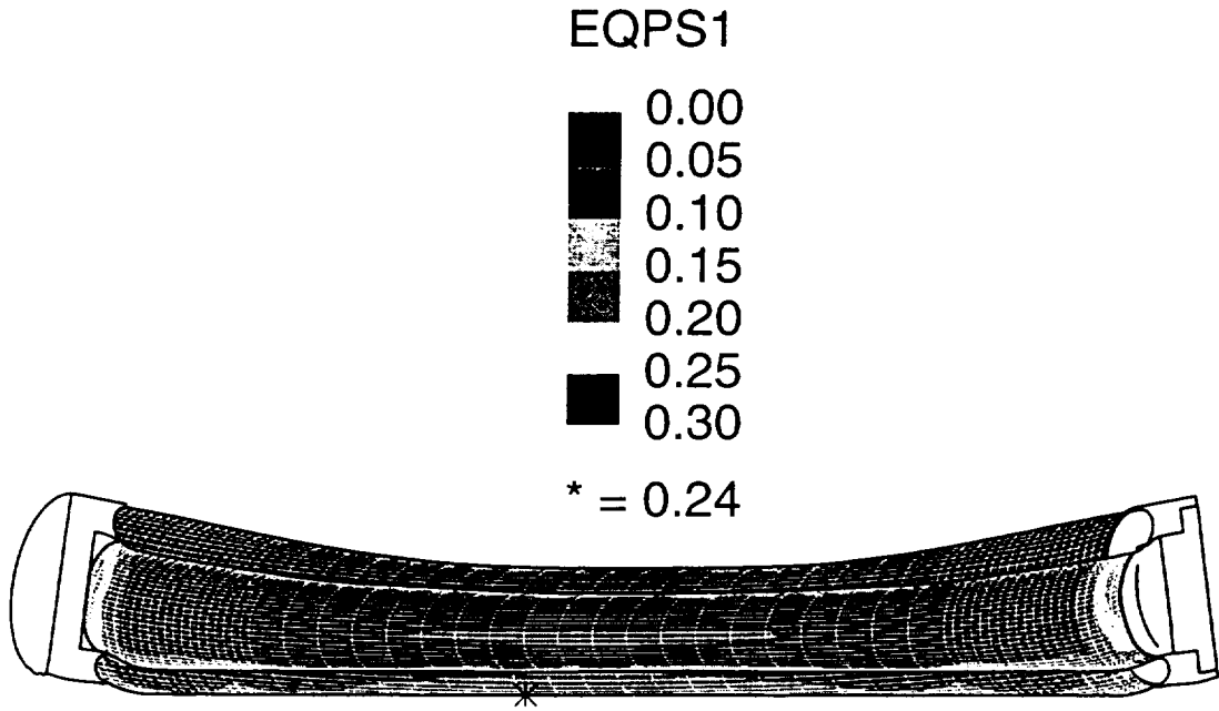
Figure A-21 Steel-DU-steel truck cask following a 90 mph side impact
