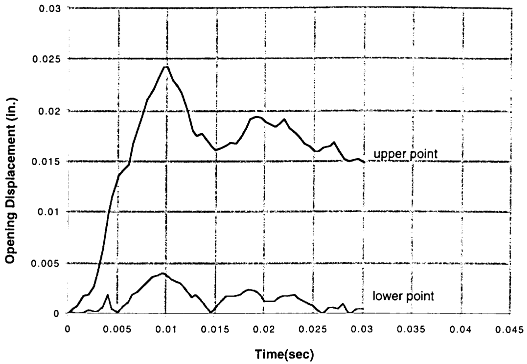
Figure A-45 Steel-lead-steel truck cask following a 30 mph corner impact
