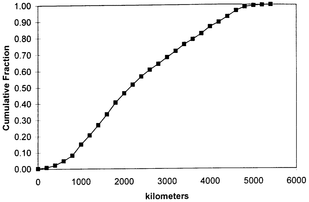
Figure 3.4a Cumulative distribution of truck route lengths.
