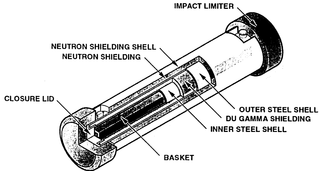
Figure 4.2 Conceptual design of a generic steel-DU-steel truck cask.
