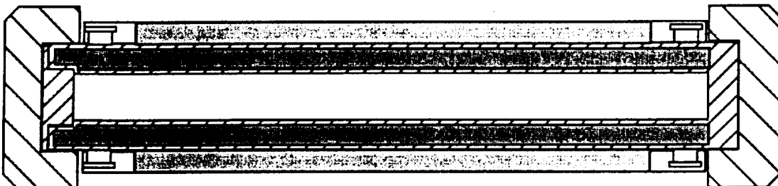
Figure 6.2 A generic, steel-DU-steel truck cask.
