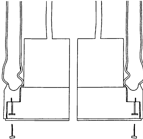
Figure 4. Predicted SETU deformed shape for a 30 m/s (85 mph) impact.
