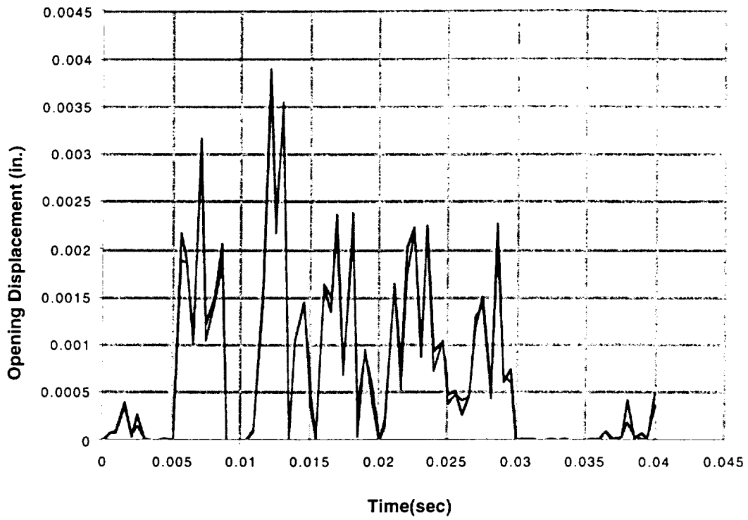
Figure A-49 Steel-lead-steel truck cask following a 30 mph end impact
