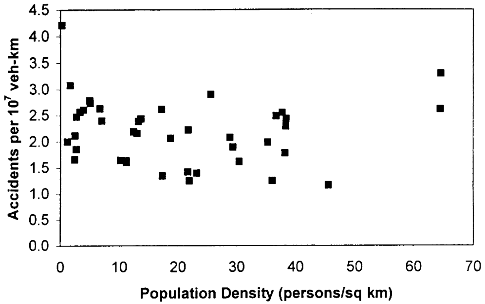
Figure 3.9a Accident rate versus rural population density.
