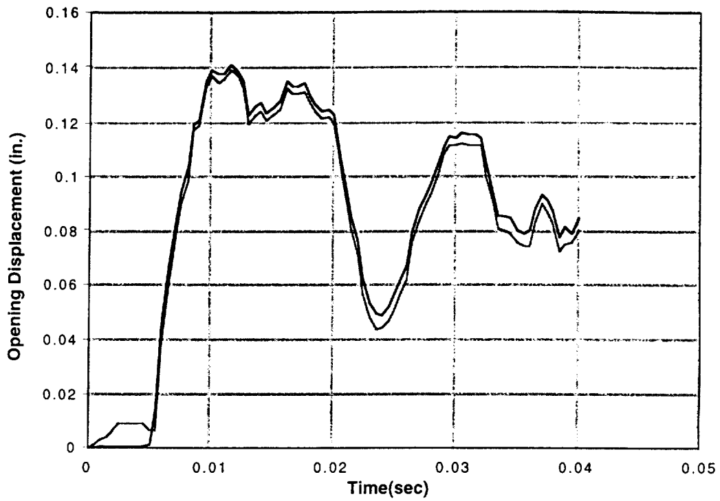
Figure A-83 Monolithic-steel rail cask following a 60 mph end impact
