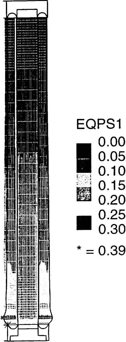
Figure A-7 Steel-lead-steel truck cask following a 90 mph end impact
