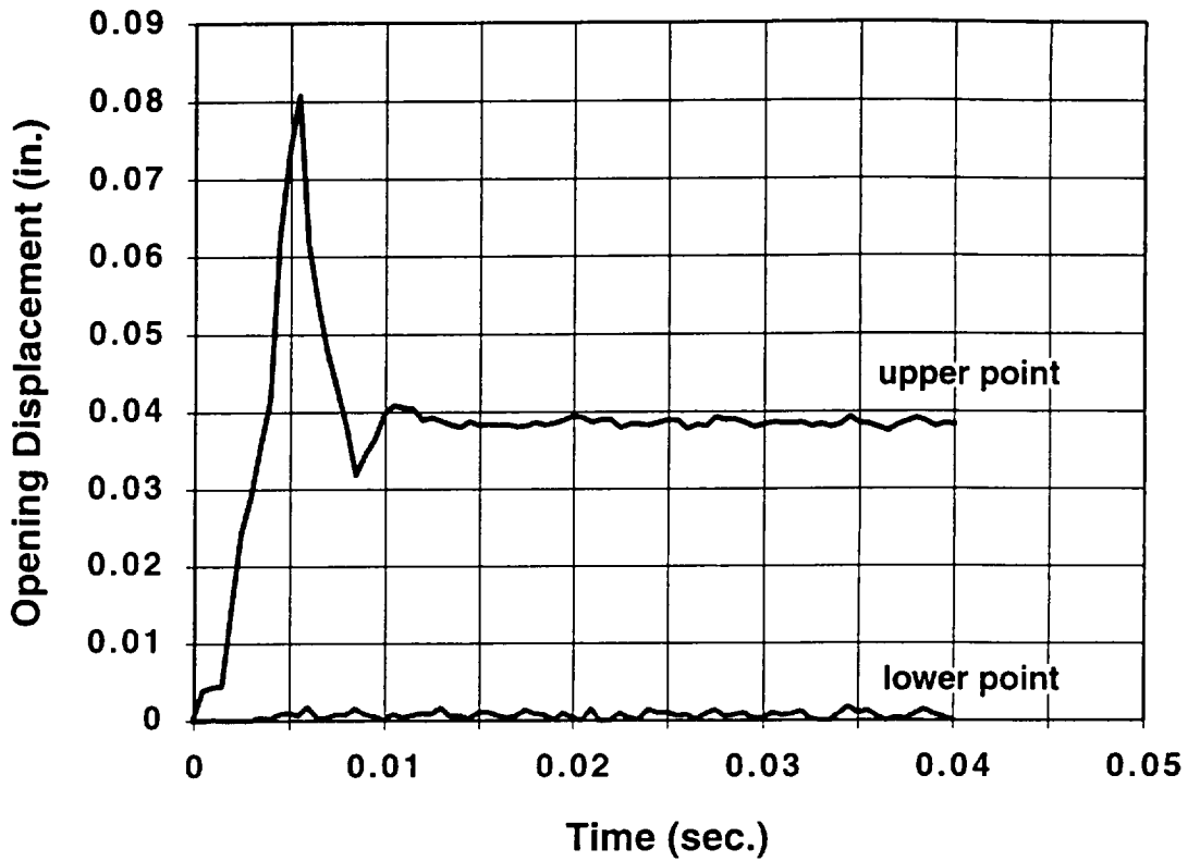
Figure 5.8 Time history for lid opening displacement for the 60 mph side-impact of the monolithic steel rail cask.
