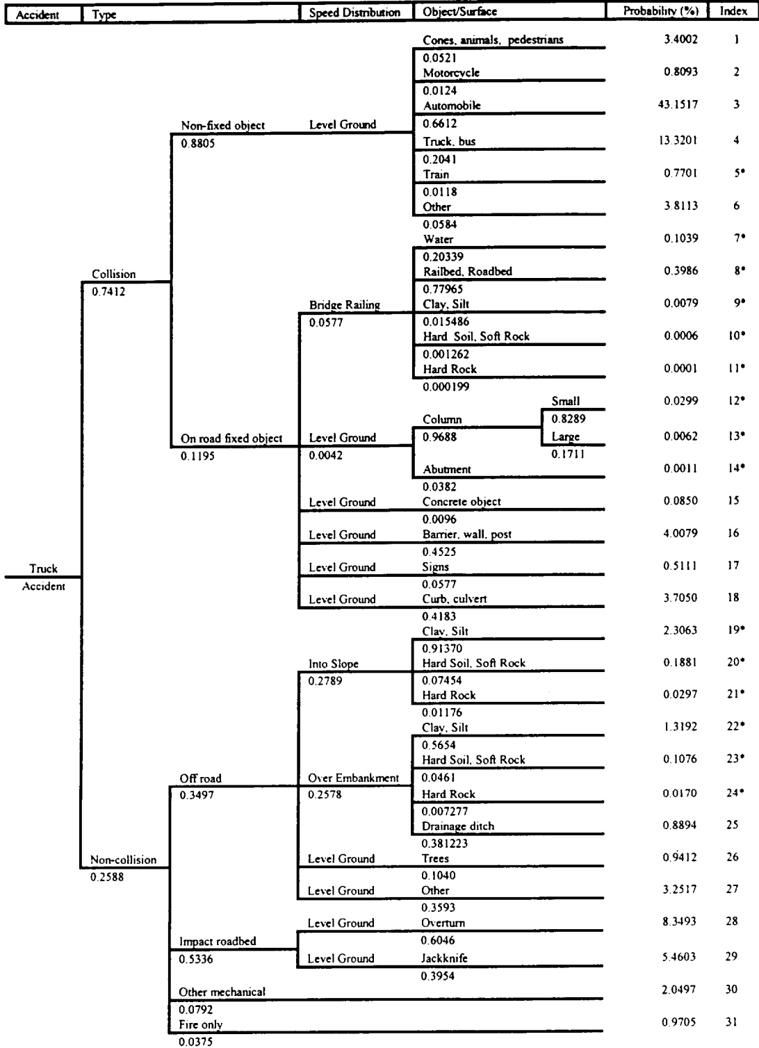
Figure 7.1 Modal Study truck accident event tree.
