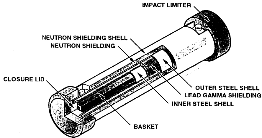
Figure 4.1 Conceptual design of a generic steel-lead-steel truck cask.
