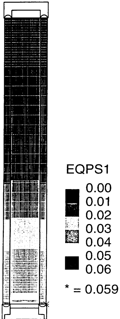
Figure A-17 Steel-DU-steel truck cask following a 60 mph end impact
