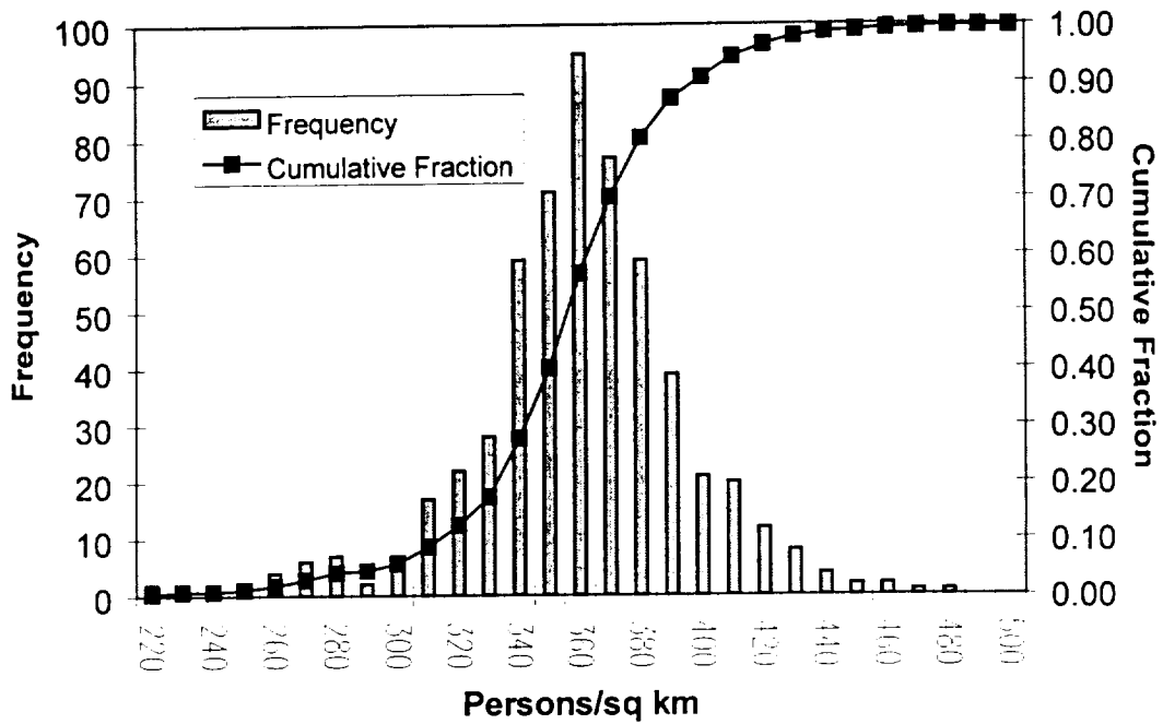
Figure 3.8b Histogram and cumulative distribution for suburban population density for suburban rail route segments.
