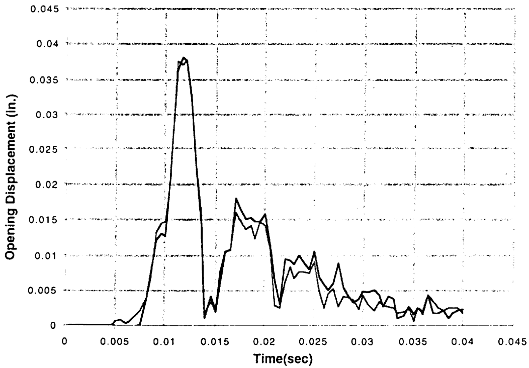
Figure A-74 Steel-lead-steel rail cask following a 120 mph end impact
