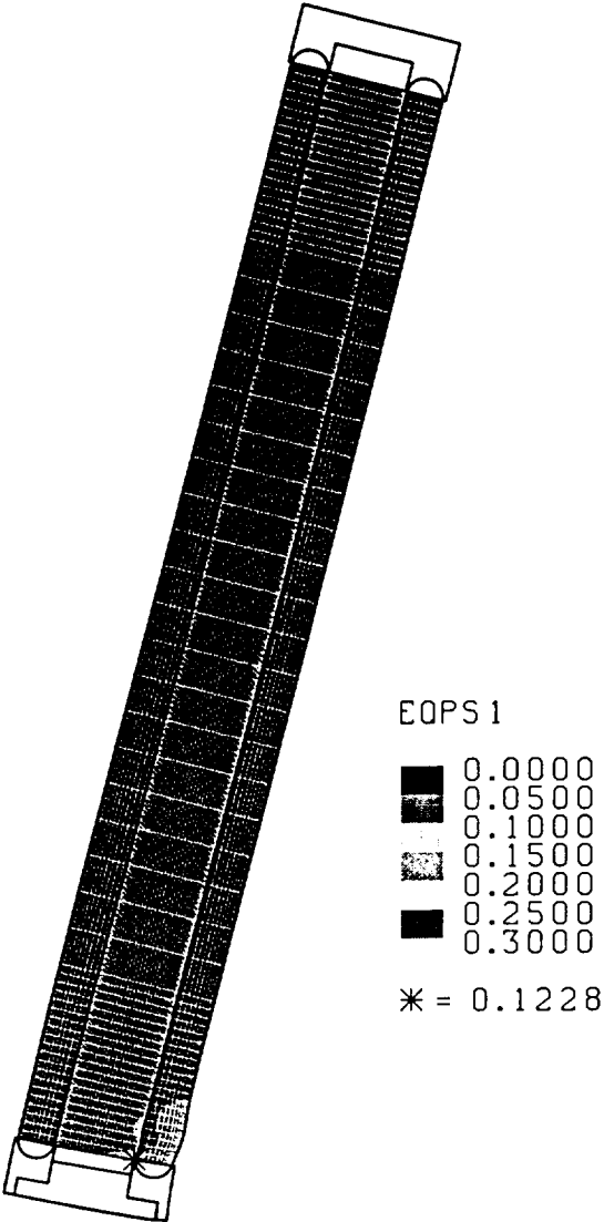
Figure A-1 Steel-lead-steel truck cask following a 30 mph corner impact
