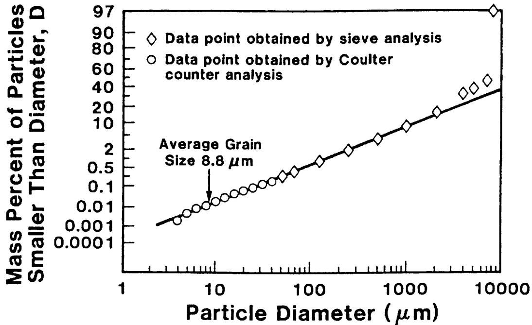
Figure 7.5 Fracture particle size distribution for depleted UO_2 .
