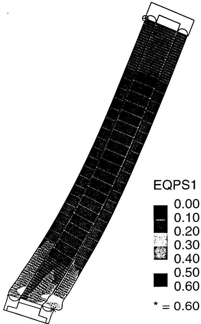
Figure A-3 Steel-lead-steel truck cask following a 90 mph corner impact
