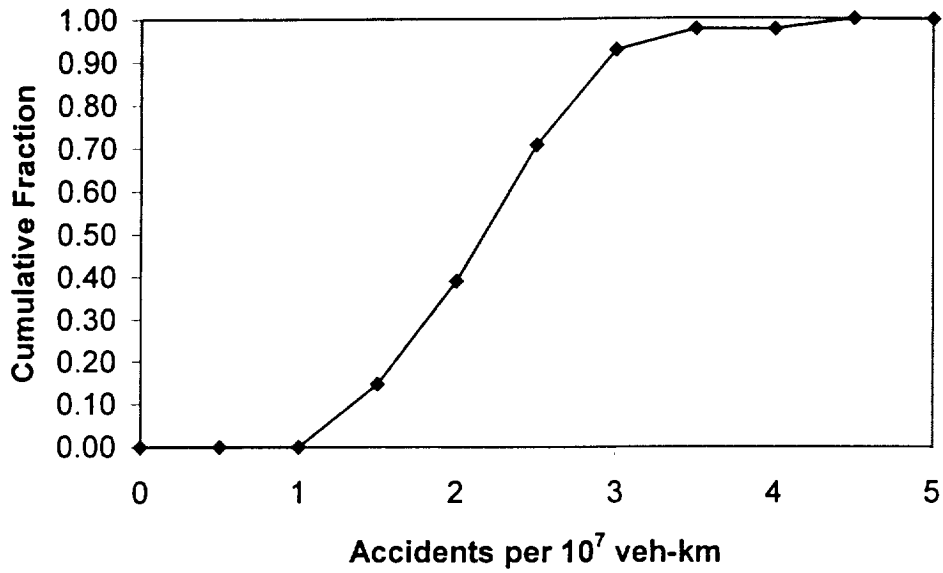
Figure 3.10a Cumulative distribution of rural accident rates.
