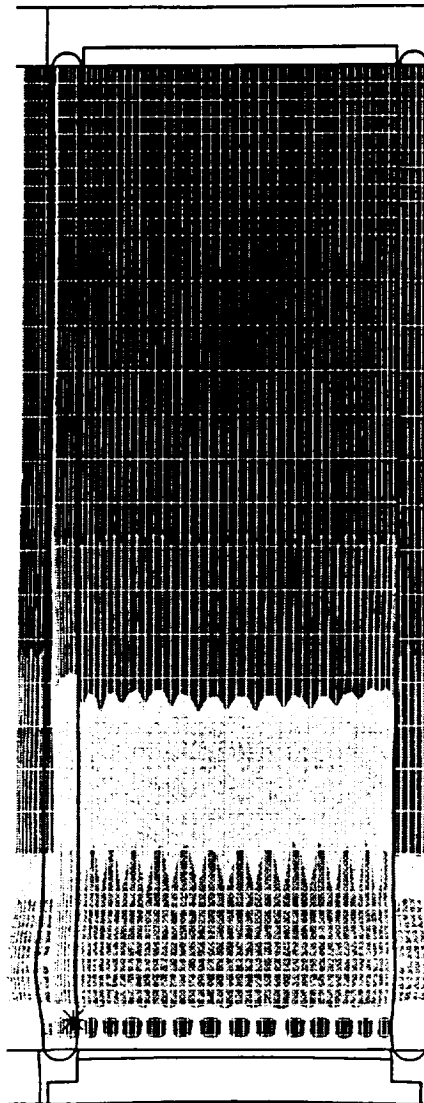
Figure A-28 Steel-lead-steel rail cask following a 90 mph end impact
