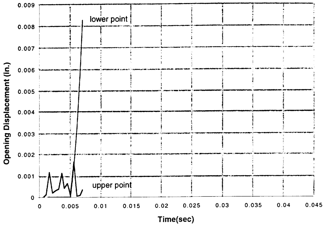
Figure A-67 Steel-lead-steel rail cask following a 30 mph corner impact
