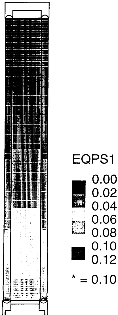
Figure A-18 Steel-DU-steel truck cask following a 90 mph end impact
