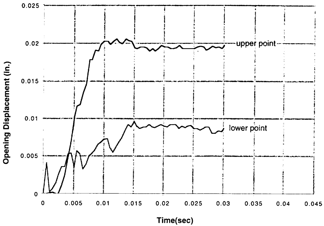
Figure A-55 Steel-lead-steel truck cask following a 120 mph side impact
