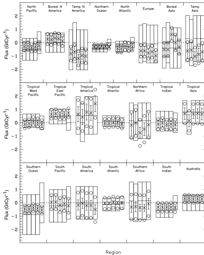
Fig. 6. Results of sensitivity tests 2–5. The control inversion is denoted by the leftmost set of symbols (as in Fig. 5). The ‘Zero Land Priors’ case (sensitivity test 2), ‘No Rect’ case (sensitivity test 3), ‘Adjust Rect’ case (sensitivity test 4), and ‘Zero Ocean’ (sensitivity test 5) are denoted progressively to the right. Mean does not include CSIRO.
