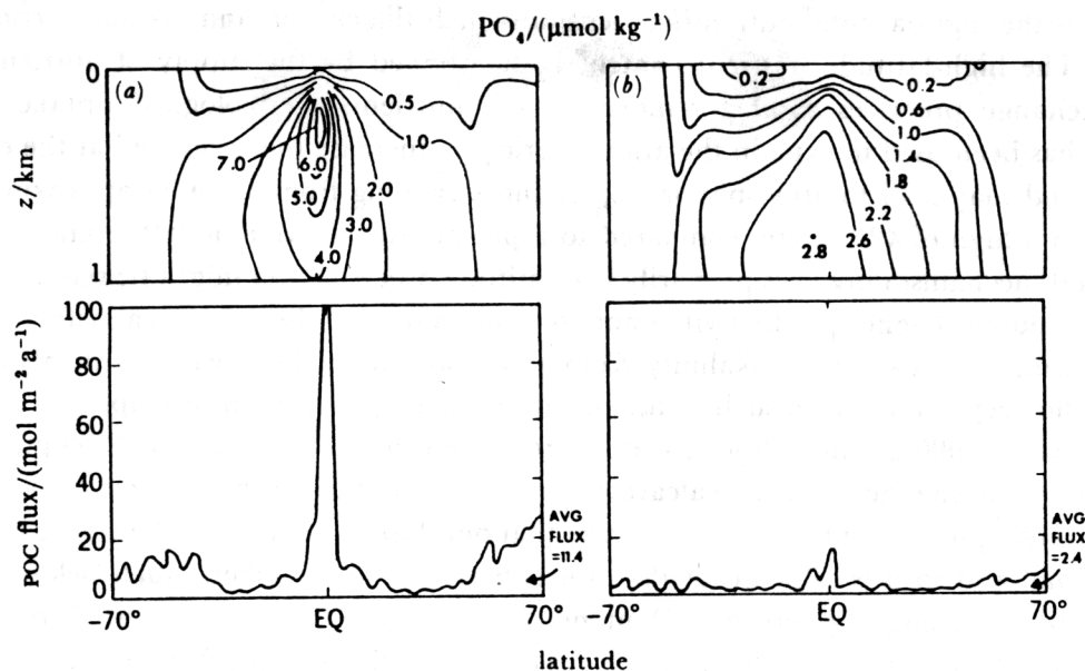
FIGURE 9. (a) Phosphate in the upper 1000 m, and particulate organic carbon flux (POC) predicted by a two-dimensional model obtained by zonally averaging the three-dimensional model in figure 7. (b) The same figures for a version of the two-dimensional model in which half of the organic carbon production is put into the form of dissolved organic matter with a regeneration timescale of 166 years.
