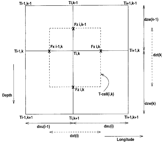
FIG. 3. Grid arrangement in the longitudinal-vertical plane for the ocean model. The dashed lines represent the boundary of the T -cell, with T_{i,k} at the center. The discretized horizontal component of the diffusive flux F^x is located on the vertical boundaries, and the vertical component F^z on the horizontal boundaries. The grid dimensions are indicated. Note that the i, k label is used for the flux F^x located on the east boundary of the tracer cell, whose center is the tracer point T_{i,k} , and likewise for the flux F^z at the bottom of the T -cell. The difference operators acting on a tracer are given by \delta_x T_{i,k} = (T_{i+1,k} - T_{i,k})/dxu_i and \delta_z T_{i,k} = (T_{k,i} - T_{k+1,i})/dzw_k . On a flux, they are \delta_x F_{i,k}^x = (F_{i+1,k}^x - F_{i,k}^x)/dxu_i and \delta_z F_{i,k}^z = (F_{i,k}^z - F_{i,k+1}^z)/dzt_k . The divergence of the diffusive flux yields the diffusion operator R_{i,k} = -(\delta_x F_{i-1,k}^x + \delta_z F_{i,k-1}^z) centered at the tracer point T_{i,k} .
