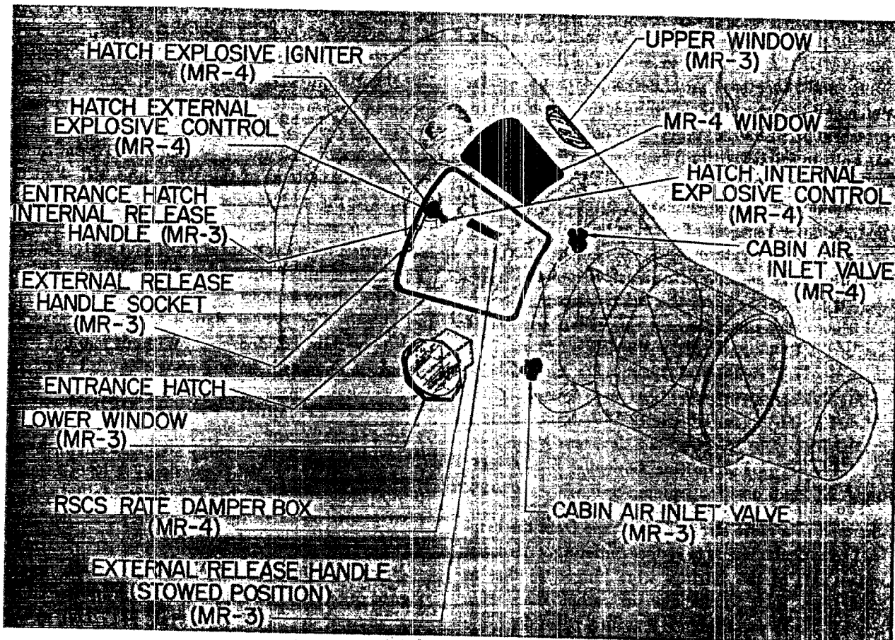
FIGURE 2-1. Configuration differences between MR-3 and MR-4 spacecraft.
