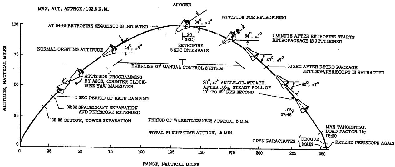
FIGURE 2-5. Flight profile for MR-4.
