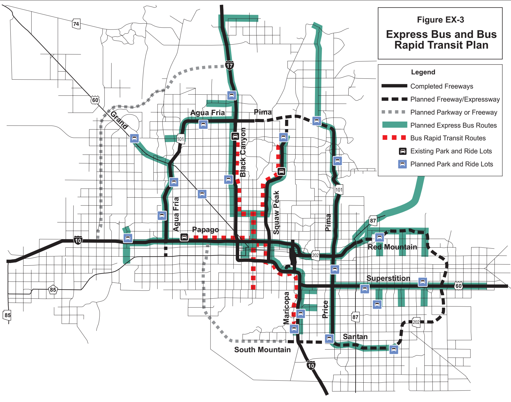
Figure EX-3: Express Bus and Bus Rapid Transit Plan
