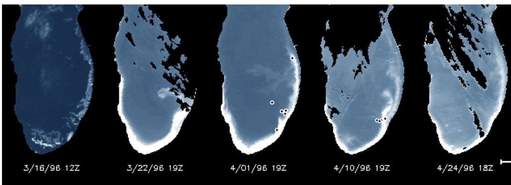
Visible band satellite imagery of southern Lake Michigan AVHRR Channel 1. 3/16/96: Shore-fast ice along eastern shore, large ice floes in the south. 3/22/96 & 4/1/96: Highly reflective plume (+) = stations sampled by helicopter. 4/10/96: Off-shore eddying of plume coincides with zone of maximum sediment deposition in lake (+) = stations sampled by small boat. 4/24/96: Dissipation of plume. (Clouds are masked out on 3/22/96, 4/10/96 and 4/24/96 images.)
