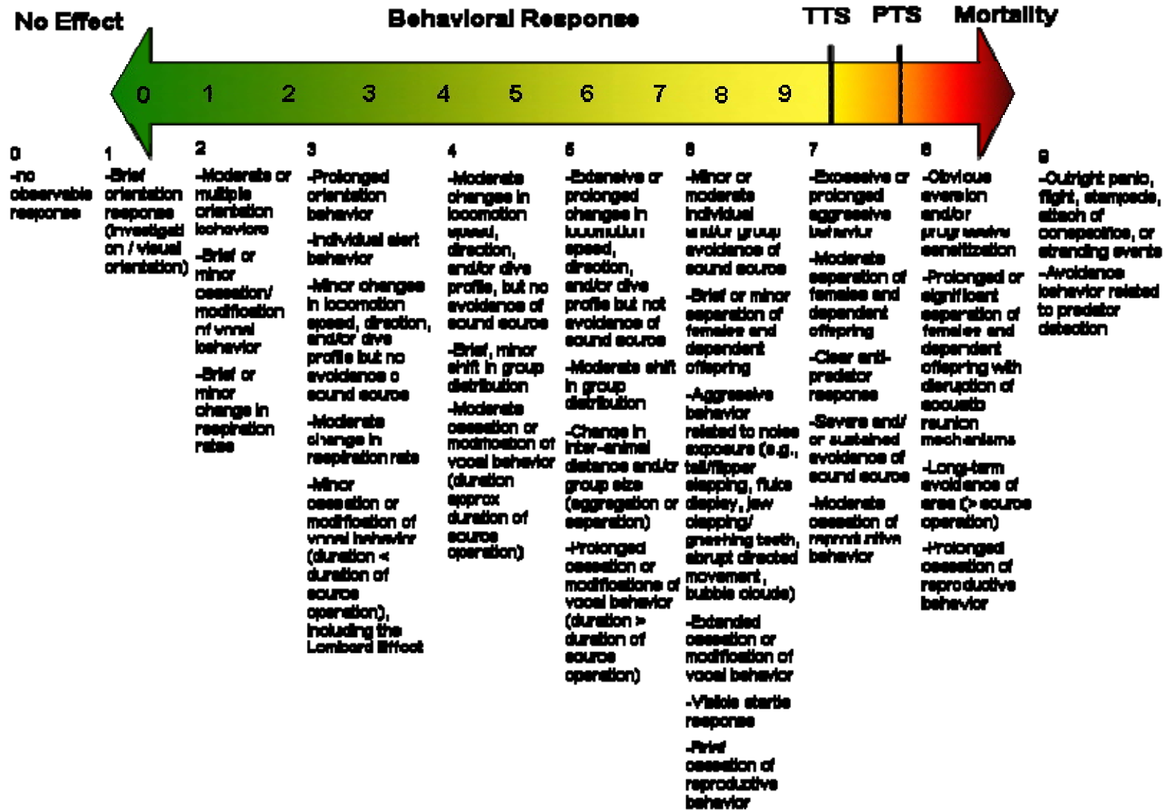
Figure 3.9-7: Marine Mammal Response Spectrum to Anthropogenic Sounds (Numbered severity scale for ranking observed behaviors from Southall et al. 2007).
