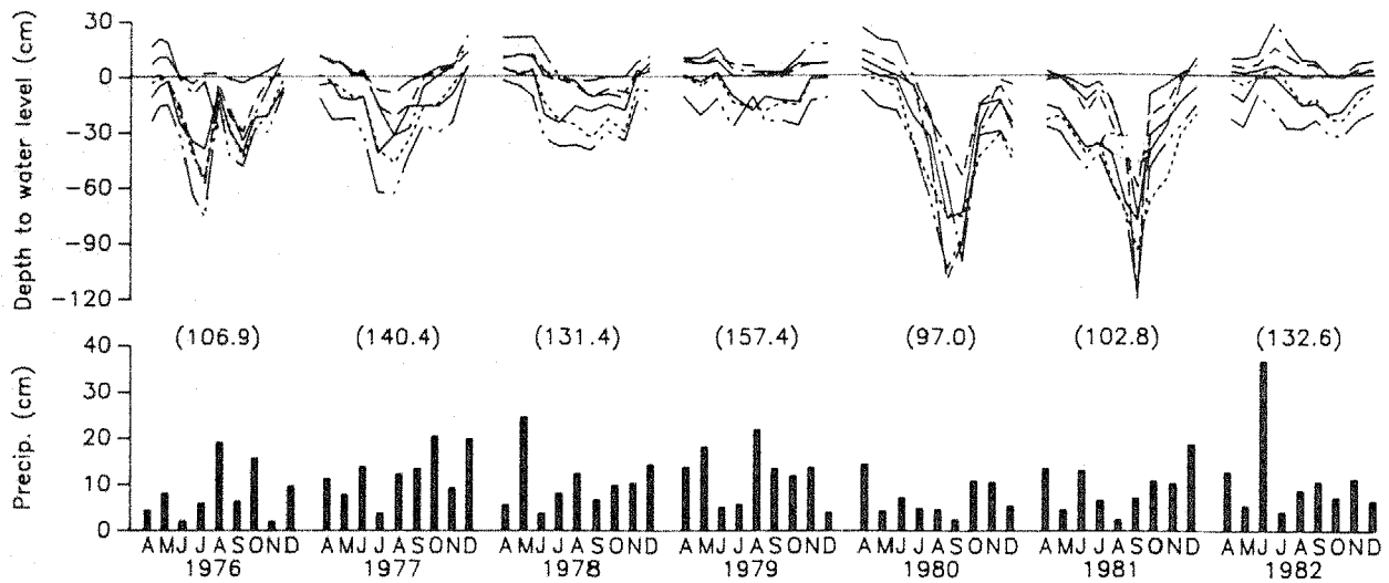
Fig. 2.7. Water levels in six Rhode Island red maple swamps during a 7-year period. Annual precipitation values are shown in parentheses. Mean annual precipitation for 1951-80 was 123.2 cm (data from Lowry 1984).
