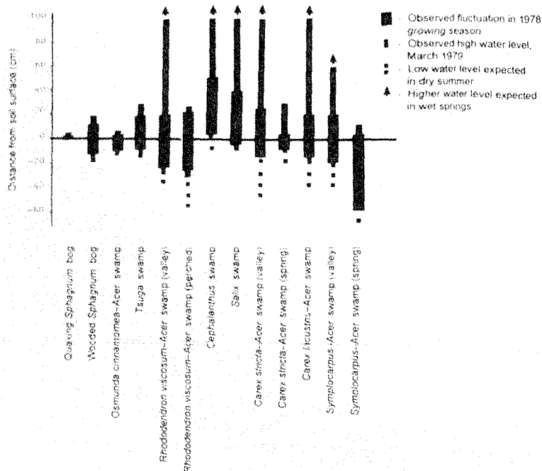
Fig. 4.2. Water level fluctuation in red maple swamps and other wetland communities of northwestern Connecticut (redrafted from Messier 1980).
