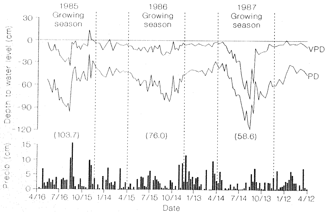
Fig. 2.8. Groundwater levels in very poorly drained (VPD) and poorly drained (PD) soils in Rhode Island red maple swamps during a 3-year period. Each curve represents a single monitoring station selected to portray average conditions for that drainage class. Both stations had a seasonally saturated water regime. Growing season precipitation totals are shown in parentheses (F. C. Golet, unpublished data).
