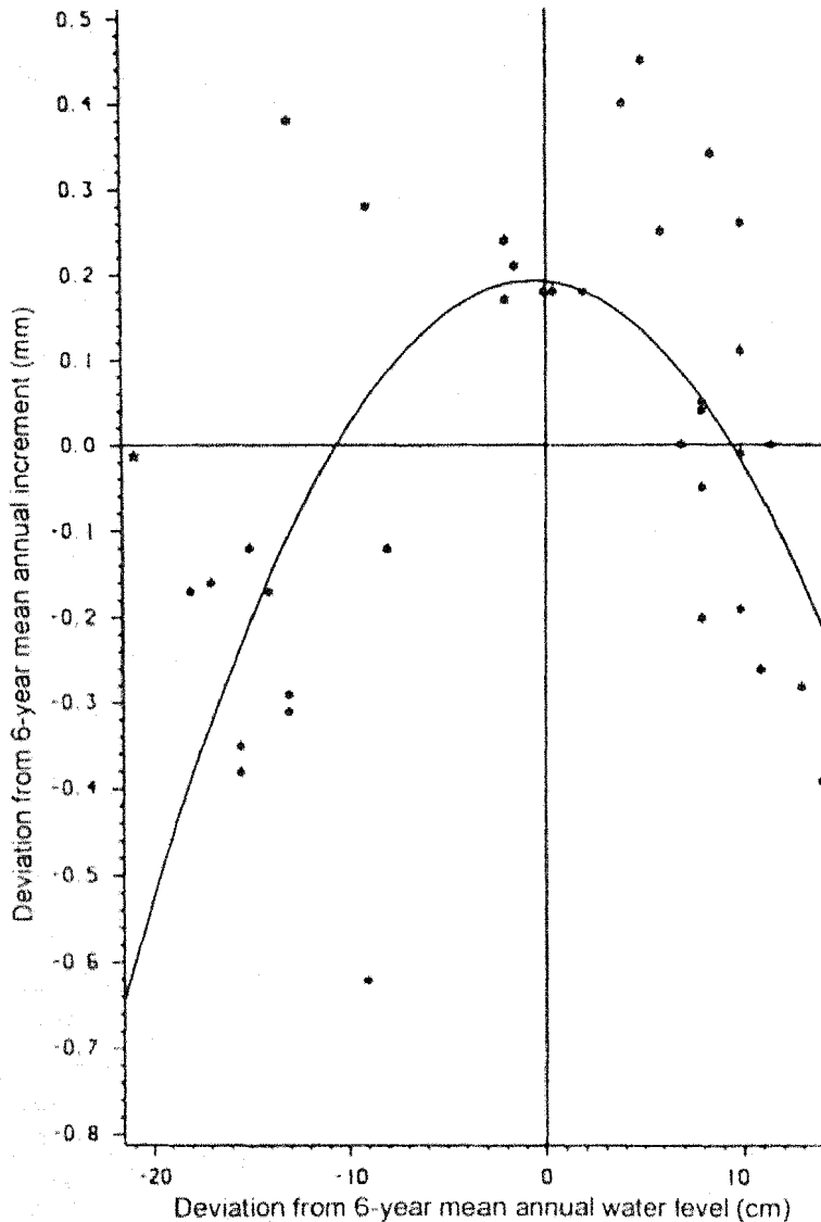
Fig. 5.2. Relationship between annual radial growth of red maple and mean annual water level in six Rhode Island red maple swamps from 1976 through 1981 (after Lowry 1984). Each point represents one year's data from one swamp.
