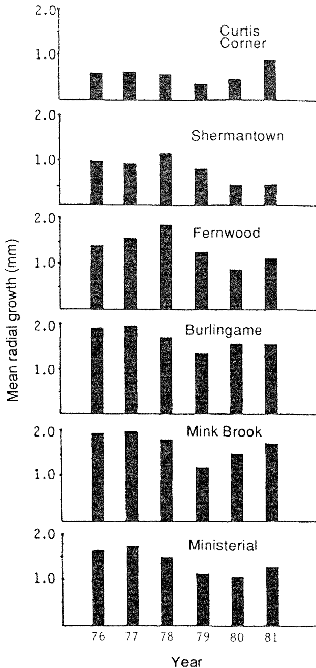
Fig. 5.1. Annual radial growth of red maple in six Rhode Island swamps from 1976 through 1981 (after Lowry 1984). Data are based on 30 trees per site, two increment cores per tree.
