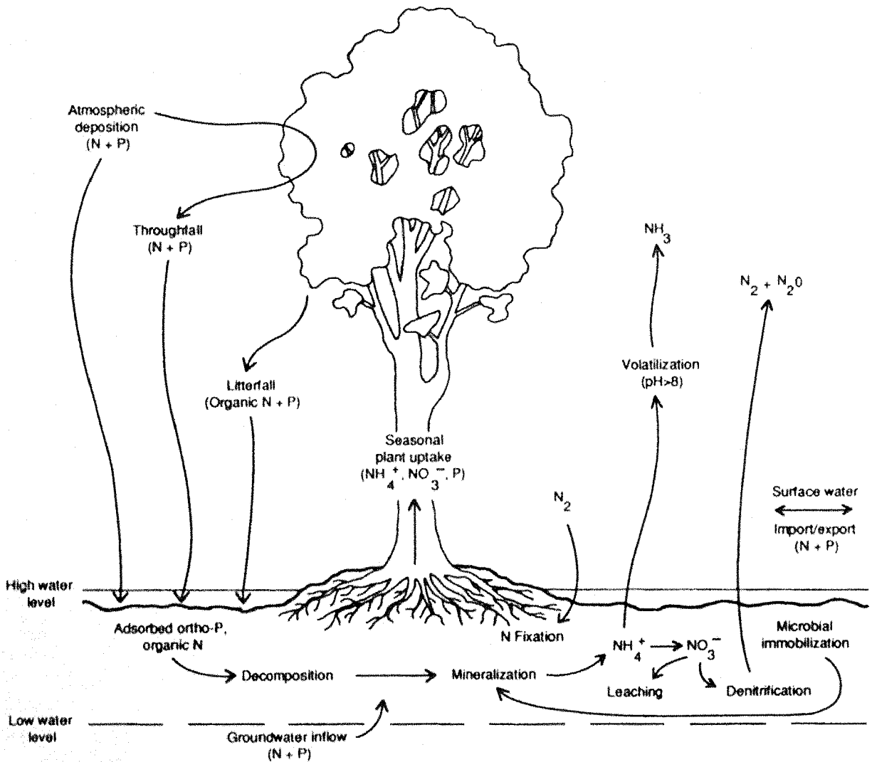
Fig. 5.4. Nutrient-cycling processes and pathways in a red maple forested wetland (modified from Brinson et al. 1981c).
