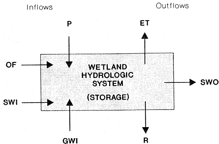
Fig. 2.5. Inflow-outflow components and water budget equation for a red maple swamp (based on Novitzki 1982).
