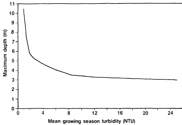
Figure 23. Relationship between maximum depth of boundaries of submersed meadows and mean turbidity in water over these boundaries during growing seasons of 1982 and 1983 in the St. Marys River. Left portion of the curve is for upstream locations and right portion is for downstream sites.
