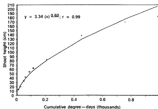
Figure 60. Relationship between mean height of tallest shoots for Sparganium eurycarpum and temperature as degree-days above the germination threshold of 7^{\circ}\text{C} .
