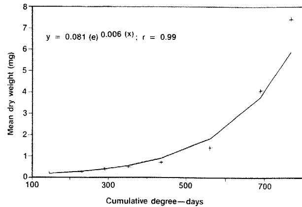
Figure 61. Relationship between mean dry weight of Lestes disjunctus disjunctus and temperature as degree-days above the developmental threshold of 4.3^{\circ}\text{C} .
