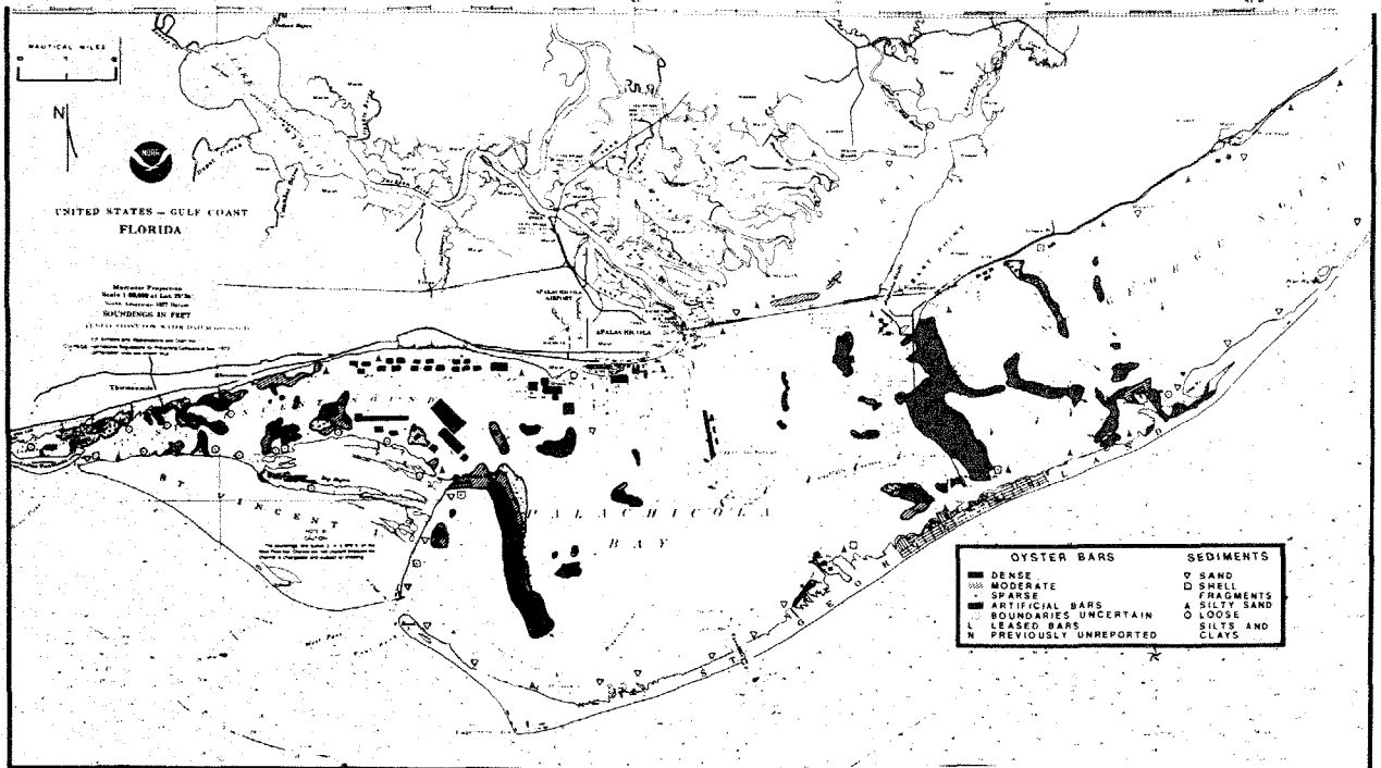
Figure 20. Distribution of oyster bars and sediments in the Apalachicola estuary (data from historic records, personal information from oyster dealers in Apalachicola, field observations by F.S.U. field personnel, and records from the Florida Department of Natural Resources) (Livingston 1980a). (This chart is currently being updated.)
