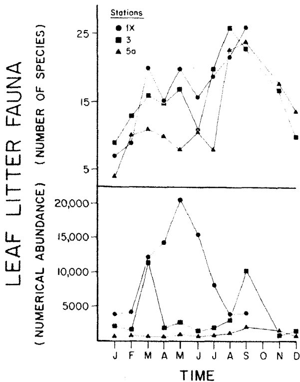
Figure 35. Numerical abundance and species richness of invertebrates taken in leaf-litter baskets at various permanent sampling sites in the Apalachicola estuary, monthly from January, 1976, through December, 1976. After Livingston (1978) and Livingston et al. (1977).
