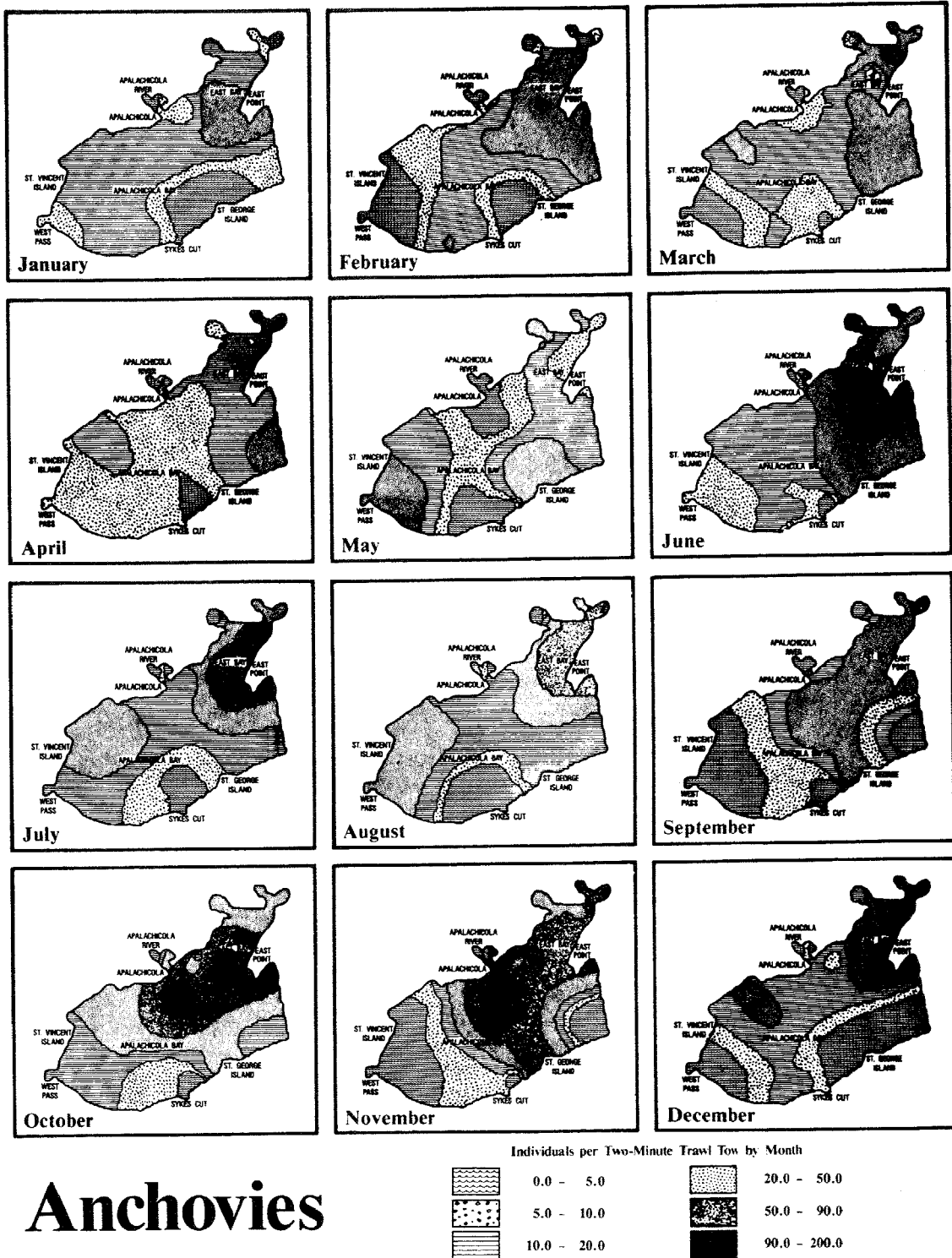
Figure 29. Average monthly distribution of anchovies ( Anchoa mitchilli ) in the Apalachicola estuary from 1972 to 1979.
