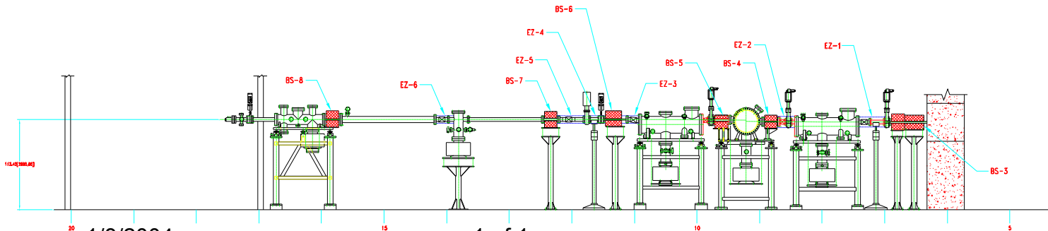
X-19A ELEVATION
