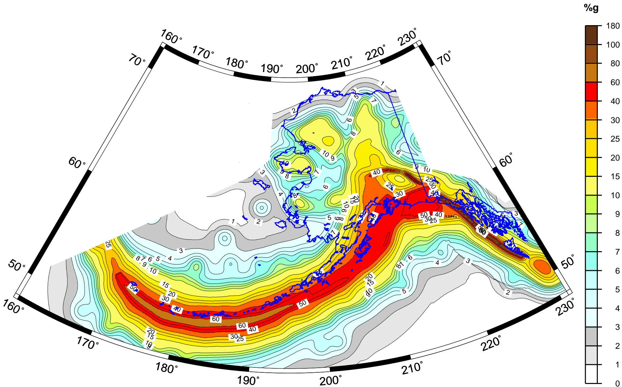
Peak Ground Acceleration (%g) with 10% Probability of Exceedance in 50 Years
