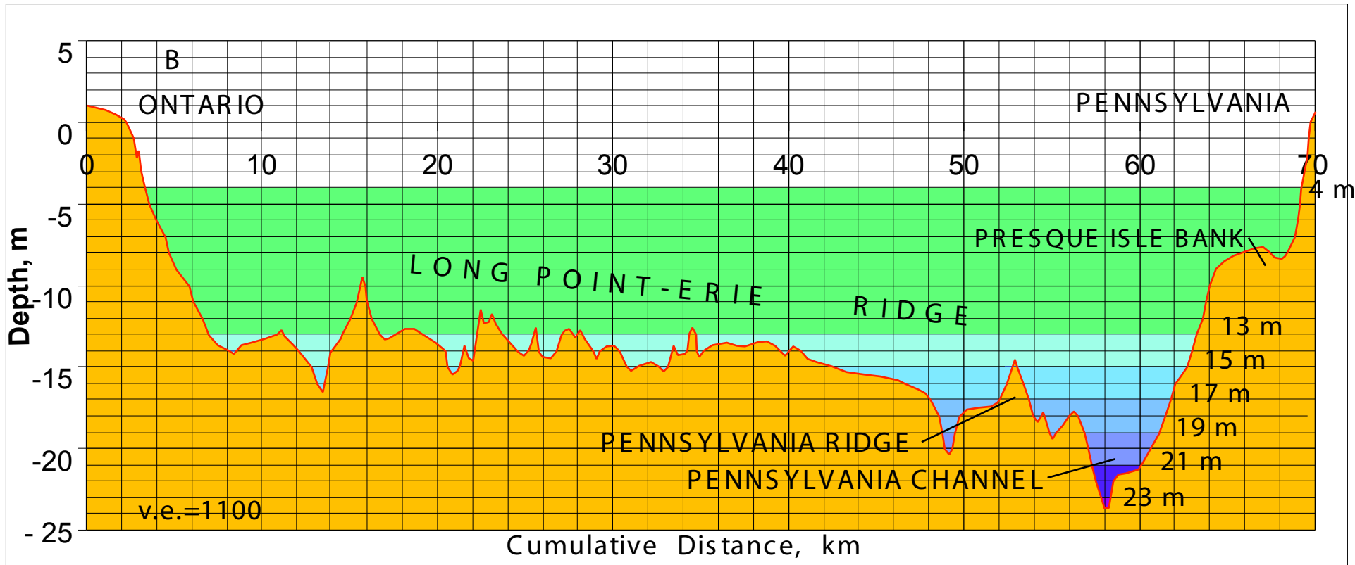
Figure 8 - Longitudinal section along the crest line of Long Point - Erie Ridge. Note that the crest of Long Point - Erie Ridge is shallower than Clear Creek Ridge.
