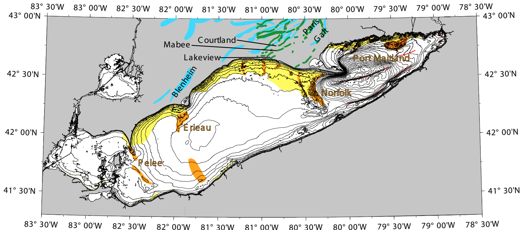
Figure 4 – Moraines occurring on the Lake Erie lake floor. Lake floor moraines, known or inferred, are positioned with bathymetry and are depicted in orange. Mapped areas where glacial drift crops out at the Lake surface are shown in yellow, adapted from Rukavina (1976), and Fuller and Foster (1998). Moraines from southern Ontario are shown in blue from Chapman and Putnam (1961) and in green from Barnett (1998) for spatial comparison with the lake floor moraines. Red lines portray topographic lineations in eastern Lake Erie.
