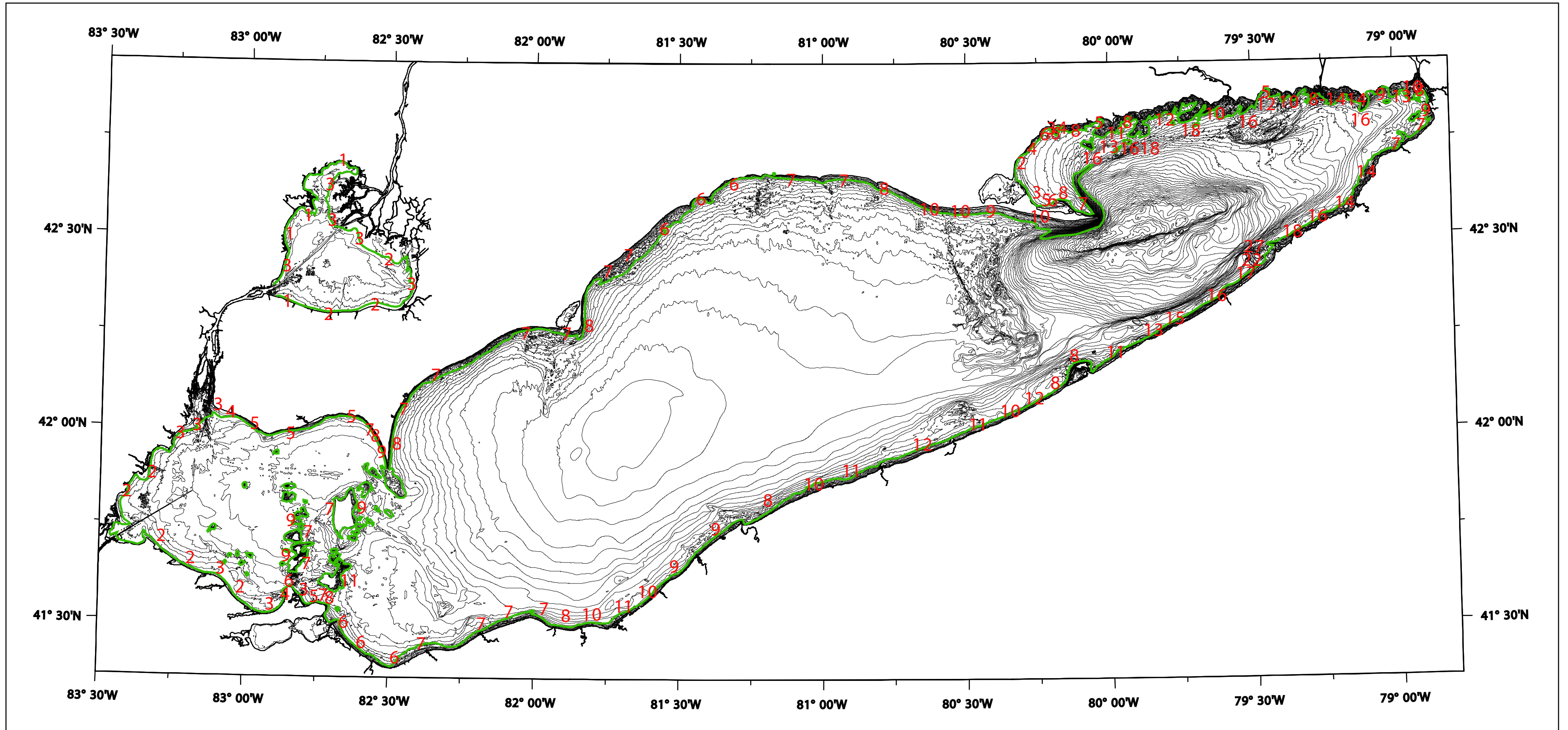
Figure 3 - Outer limits and maximum depths of the steep wave-cut shore zone of the perimeter of Lake Erie and its islands. The outer perimeter is shown as a green line. Spot depths to the lower limits of the steep shore zone are shown as red numerals.
