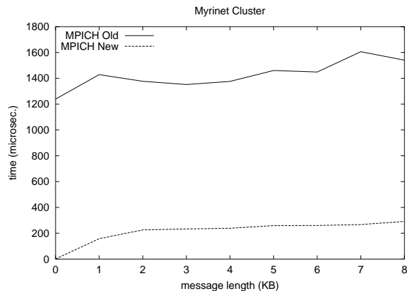
Figure 4: Performance of allgather for short messages (64 nodes). The size on the x-axis is the total amount of data gathered on each process.
