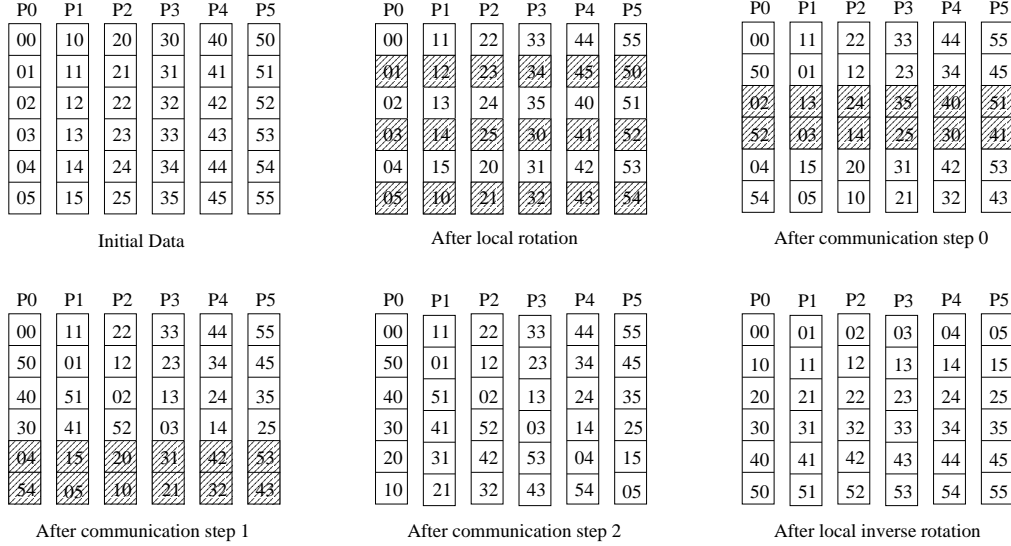
Figure 7: Bruck algorithm for all-to-all. The number ij in each box represents the data to be sent from process i to process j . The shaded boxes indicate the data to be communicated in the next step.
