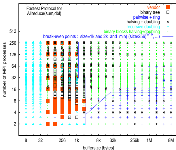
Figure 14: The fastest algorithm for allreduce ( MPI_DOUBLE , MPI_SUM ) on a Cray T3E 900
