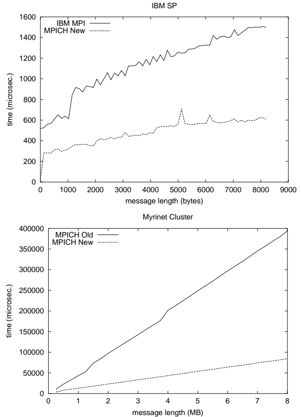
Figure 10: Performance of reduce-scatter for short messages on the IBM SP (64 nodes) and for long messages on the Myrinet cluster (32 nodes)
