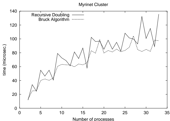
Figure 3: Performance of recursive doubling versus Bruck allgather for power-of-two and non-power-of-two numbers of processes (message size 16 bytes per process).
