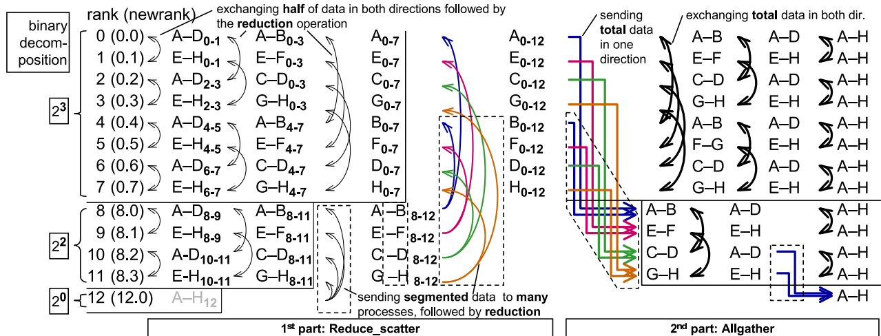
Figure 13: Allreduce using the binary blocks algorithm
