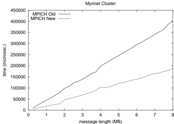
Figure 11: Performance of reduce (64 nodes)
