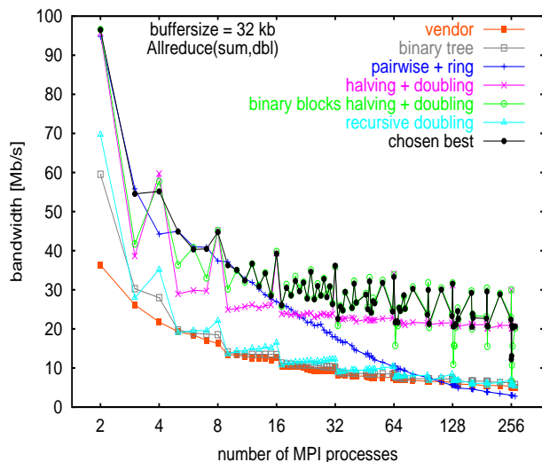
Figure 15: Bandwidth comparison for allreduce ( MPI_DOUBLE , MPI_SUM ) with 32 KB vectors on a Cray T3E 900.
