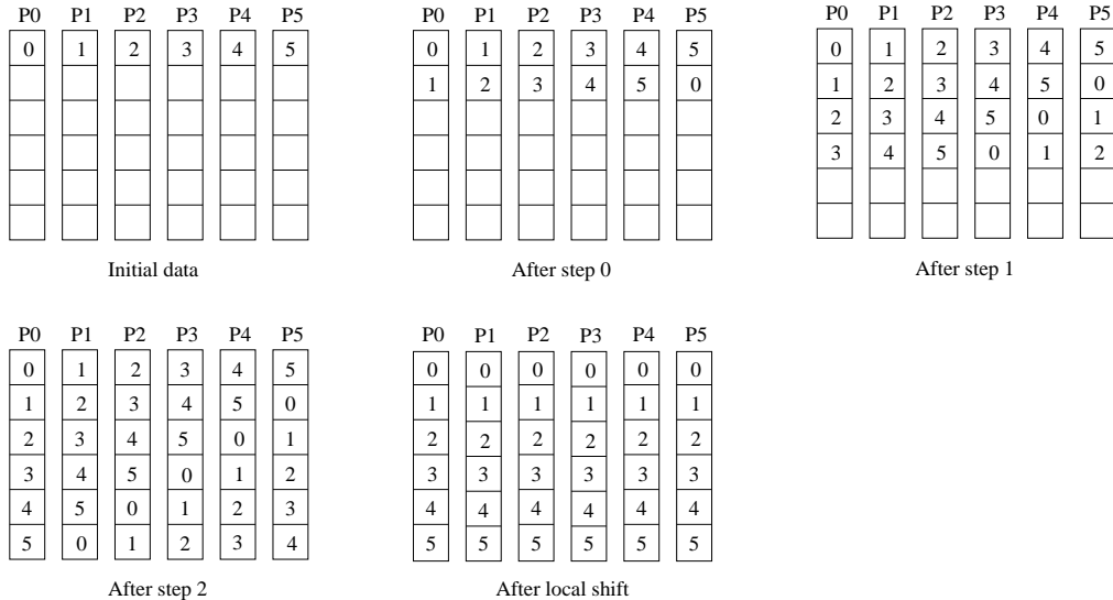
Figure 2: Bruck allgather
