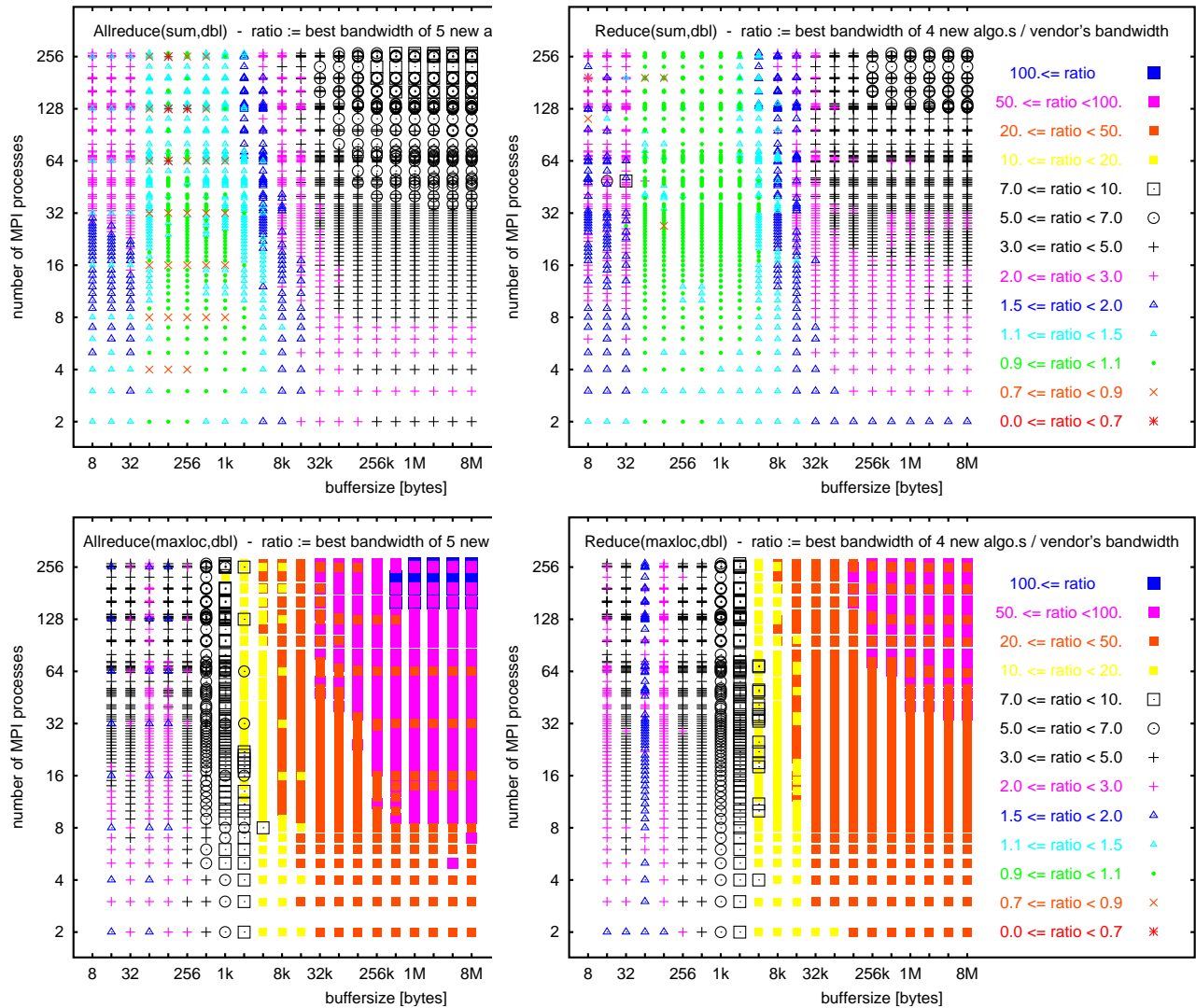
Figure 18: Ratio of the bandwidth of the fastest of the new algorithms and the vendor's algorithm for allreduce (left) and reduce (right) with operation MPI_SUM (first row) and MPI_MAXLOC (second row) on a Cray T3E 900
