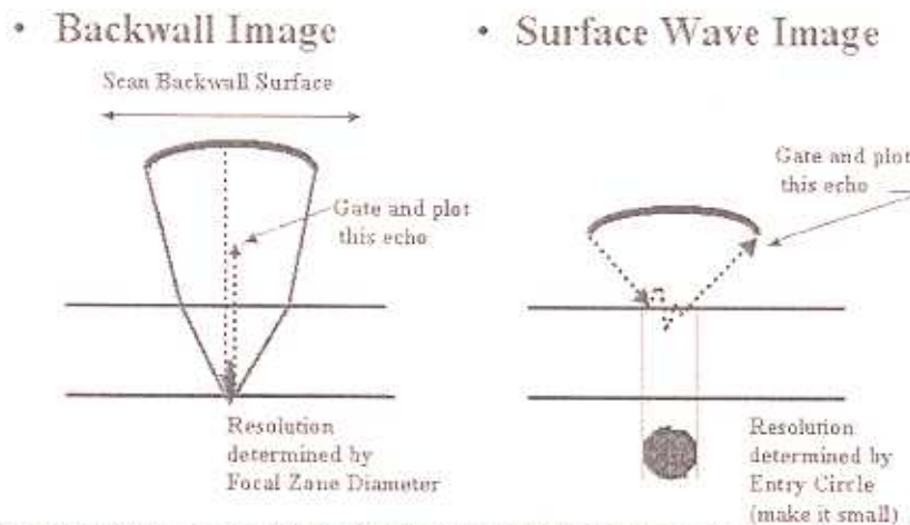
Figure 3: Schematic showing (a) Back surface reflection imaging (or back-wall imaging) and (b) mode converted surface wave imaging.
