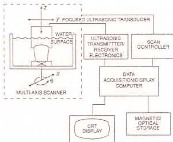
Figure 2: Schematic of an ultrasonic imaging system, higher frequencies and higher image magnification would make the same schematic an acoustic microscope.
