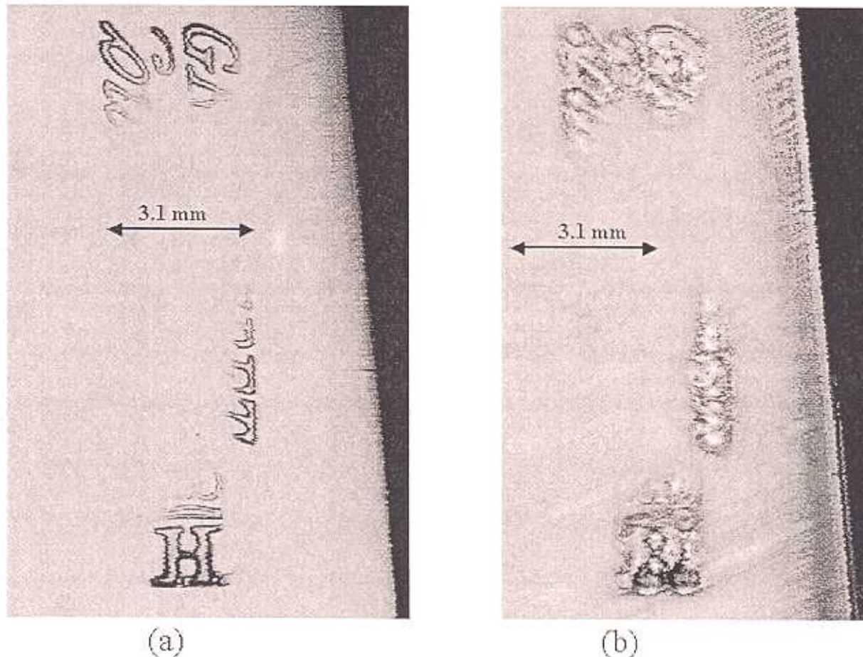
Figure 7: (a) A direct reflection image and (b) A surface wave image of the steel blade of a table knife. Deformation is not observed in the blade surface where the writing has been polished or ground away suggesting a poor original impression or, possibly, that etching produced the inscription.
