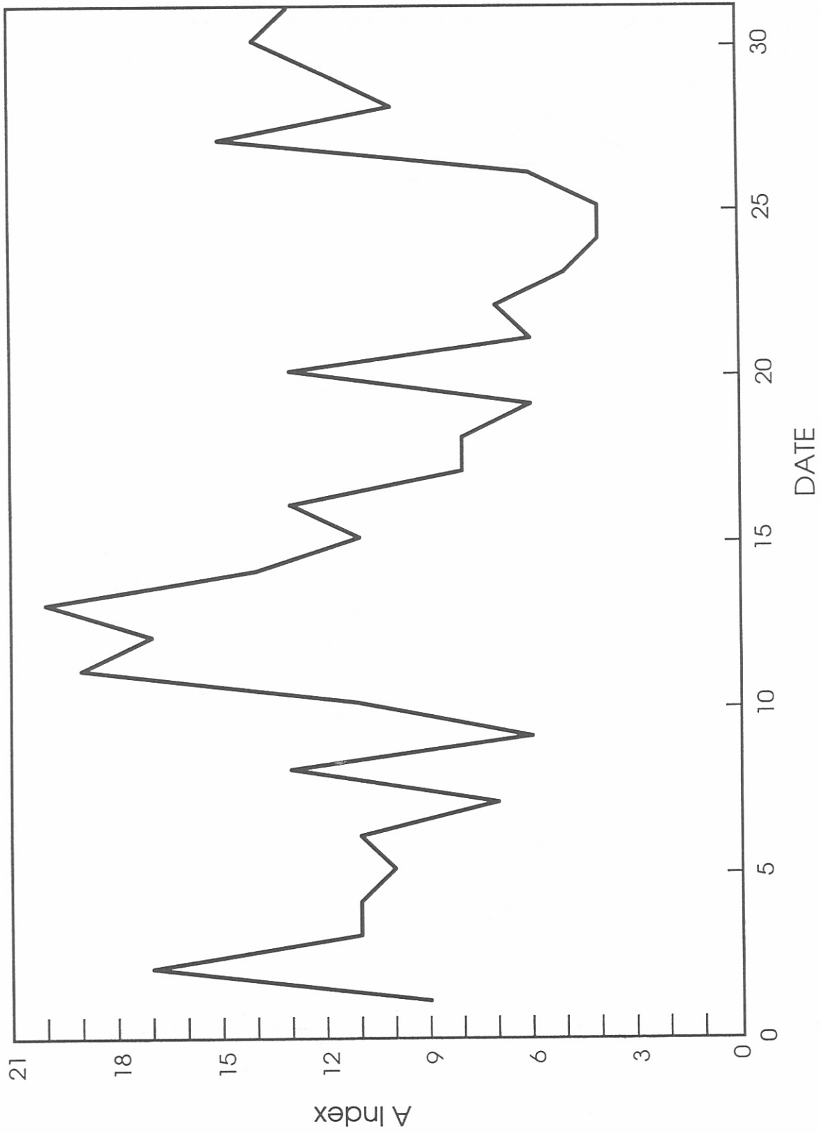
Figure A-2. Planetary - A index, January 1992.
