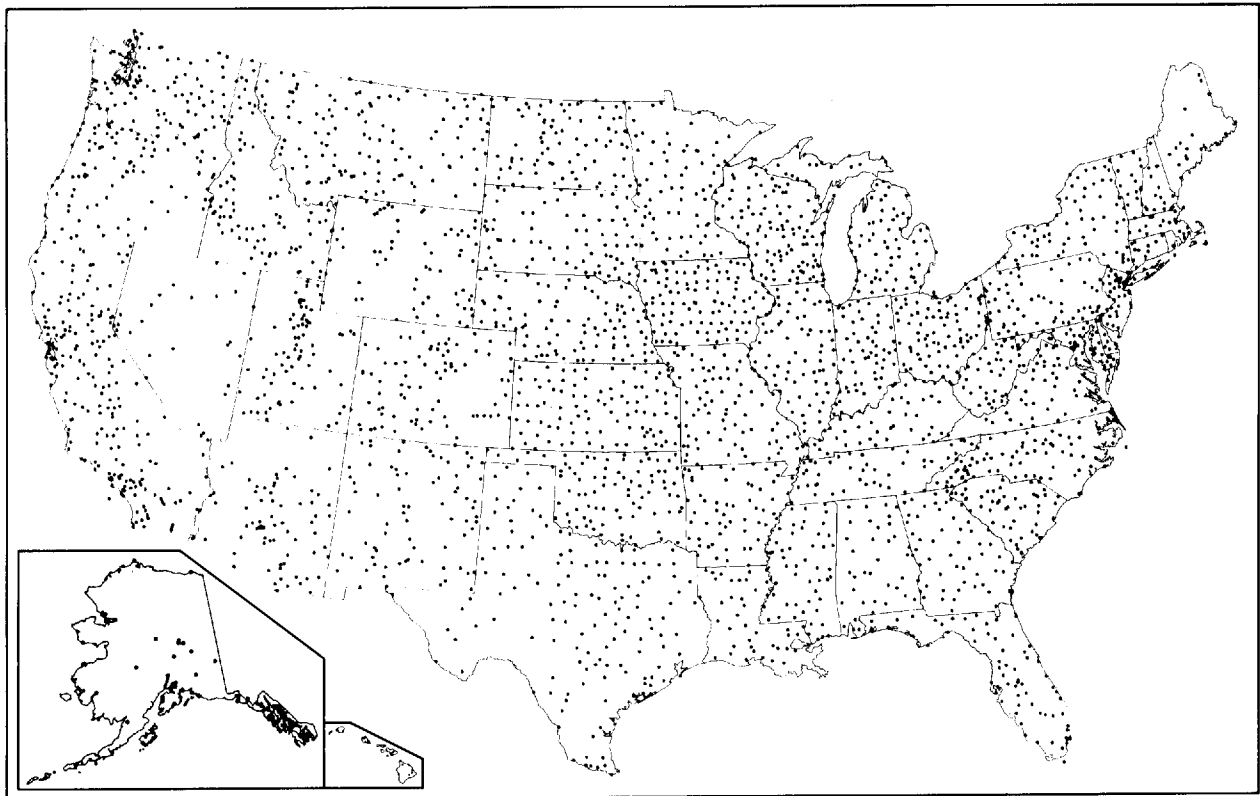
Fig. 1 Observation site distribution (3,106 locations)
