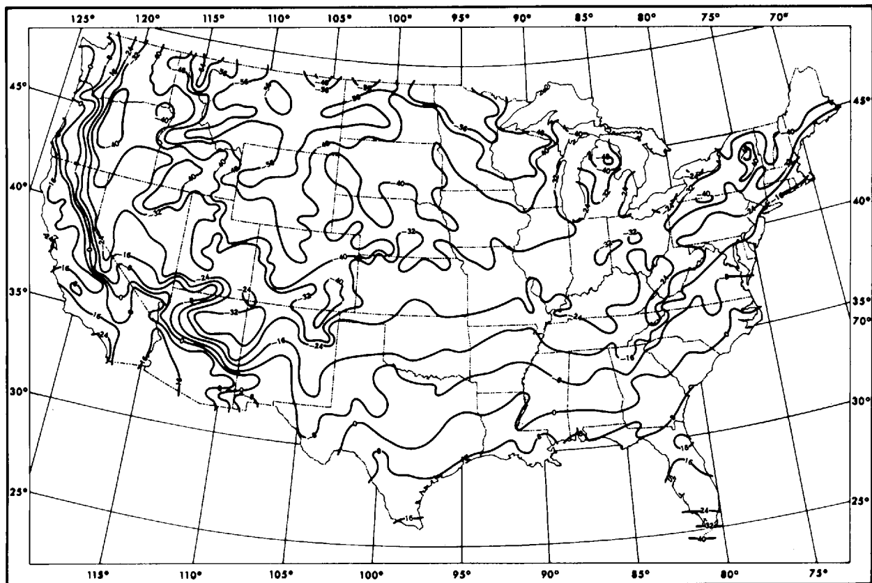
Fig. 2 50-year return period extreme annual minimum temperatures
